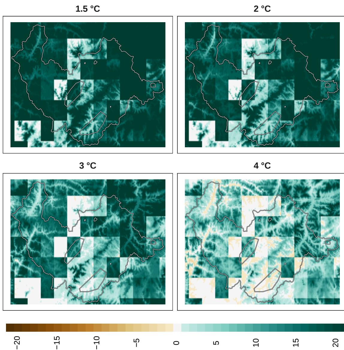
Figure 12: Adaptation effort for plants at 1 km resolution.
