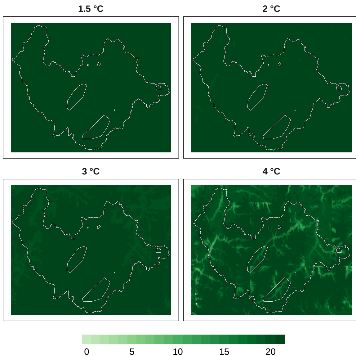
Figure 10: Number of models in agreement for insect refugia at 1 km resolution.
