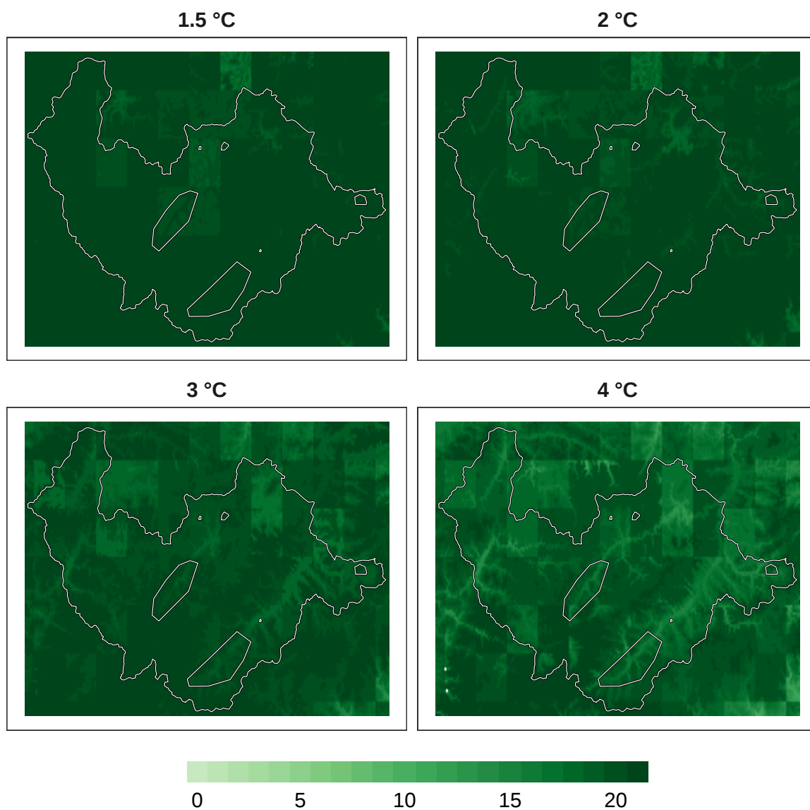
Figure 8: Number of models in agreement for bird refugia.
