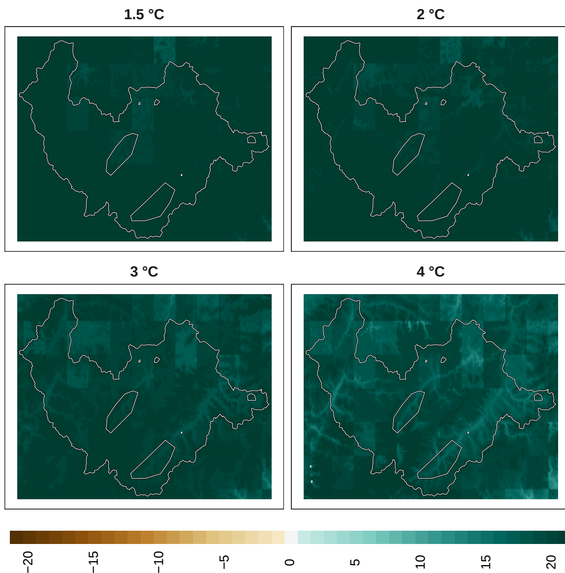
Figure 13: Adaptation effort for birds at 1 km resolution.
