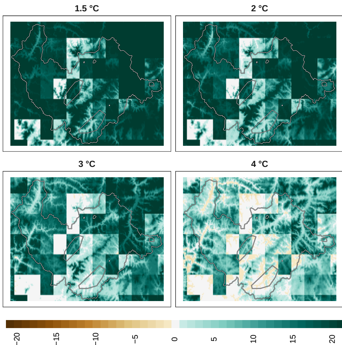
Figure 11: Adaptation effort for overall biodiversity at 1 km resolution.
