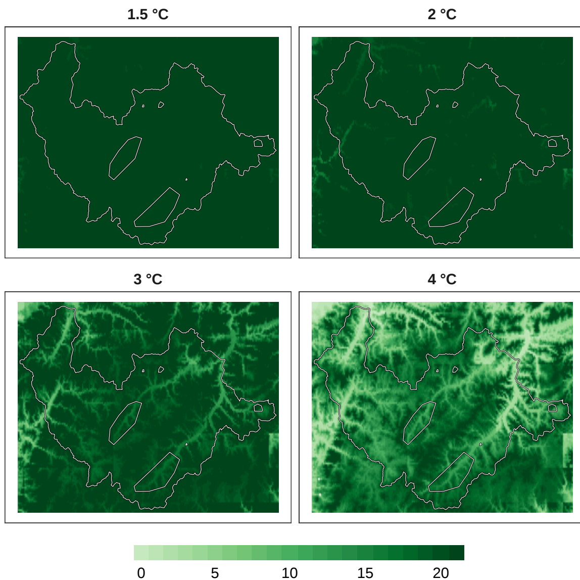
Figure 9: Number of models in agreement for mammal refugia at 1 km resolution.
