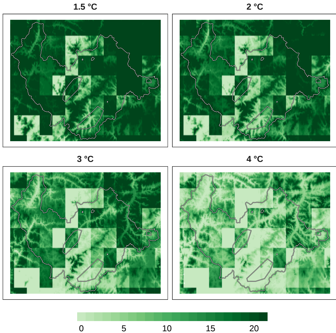
Figure 6: Number of models in agreement for overall biodiversity refugia at 1 km resolution.
