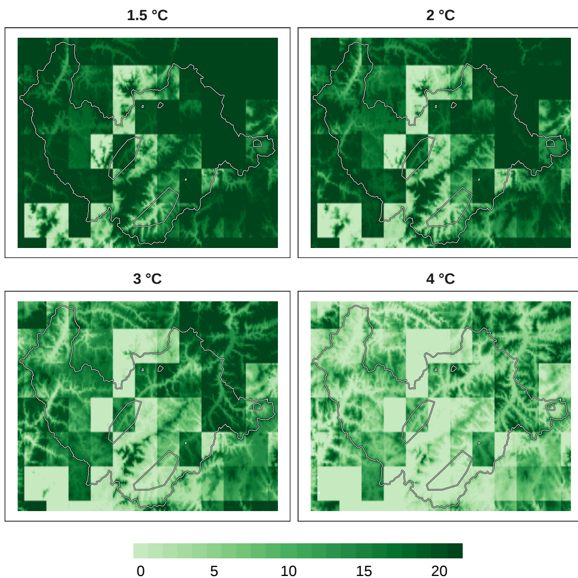
Figure 7: Number of models in agreement for plant refugia at 1 km resolution.
