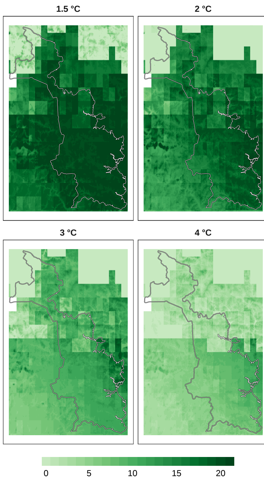
Figure 3: Number of models in agreement for overall biodiversity refugia at 1 km resolution.
