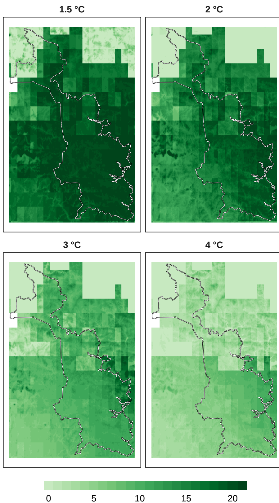
Figure 4: Number of models in agreement for mammal refugia at 1 km resolution.
