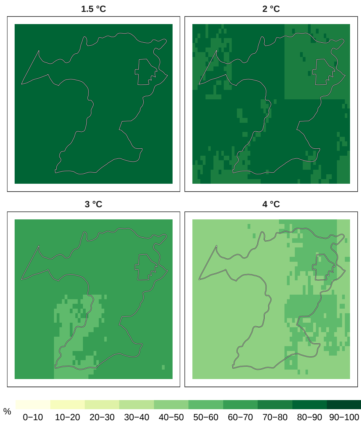
Figure 8: Percent timber species remaining at 1 km resolution.
