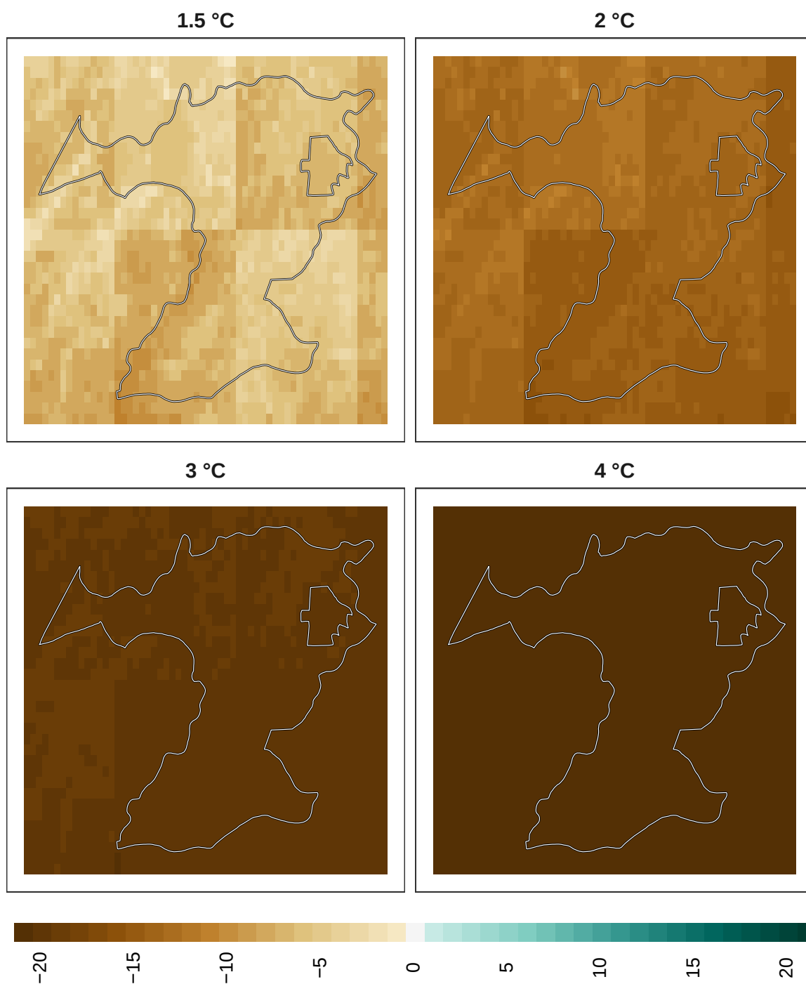
Figure 22: Adaptation effort for pollinators at 1 km resolution.
