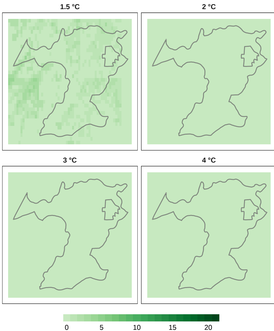
Figure 9: Number of models in agreement for overall biodiversity refugia at 1 km resolution.
