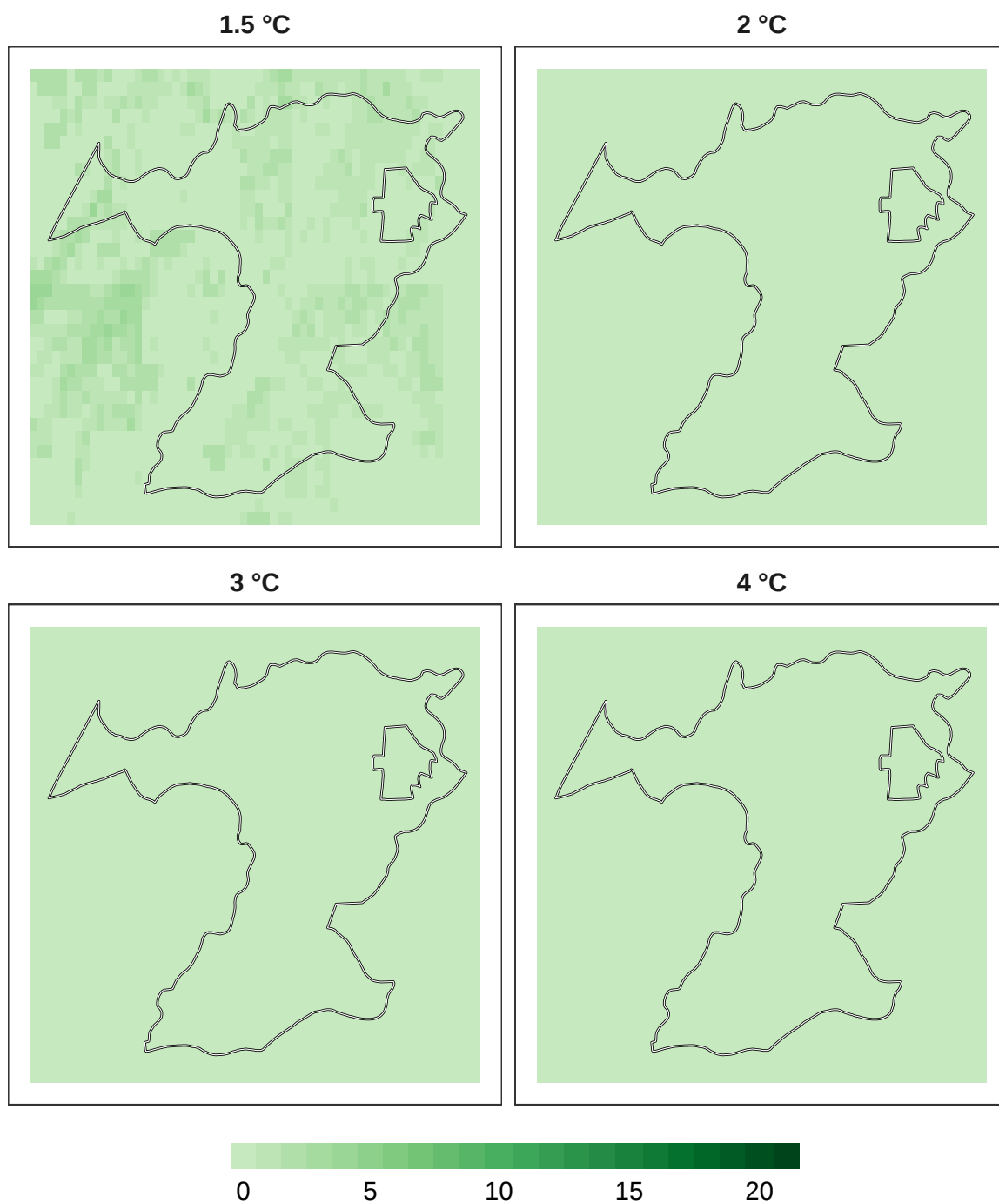
Figure 14: Number of models in agreement for insect refugia at 1 km resolution.
