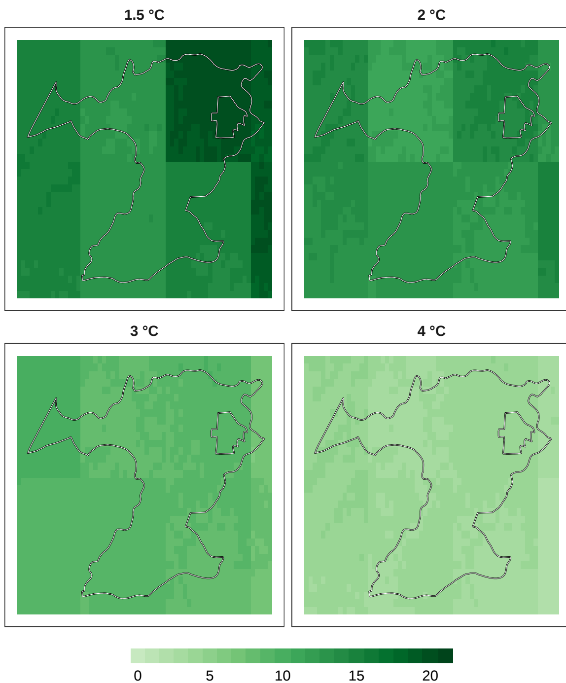
Figure 12: Number of models in agreement for mammal refugia at 1 km resolution.
