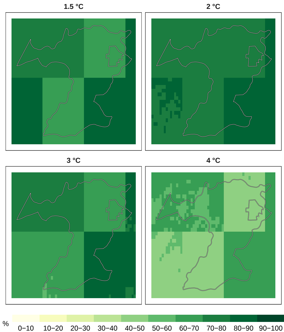
Figure 5: Percent reptiles remaining at 1 km resolution.
