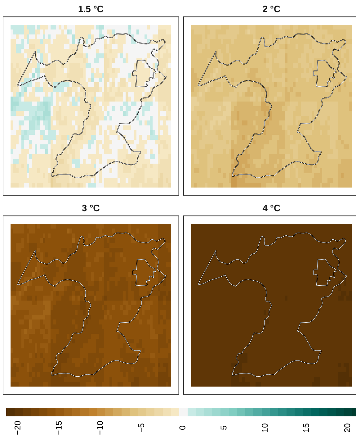
Figure 21: Adaptation effort for insects at 1 km resolution.
