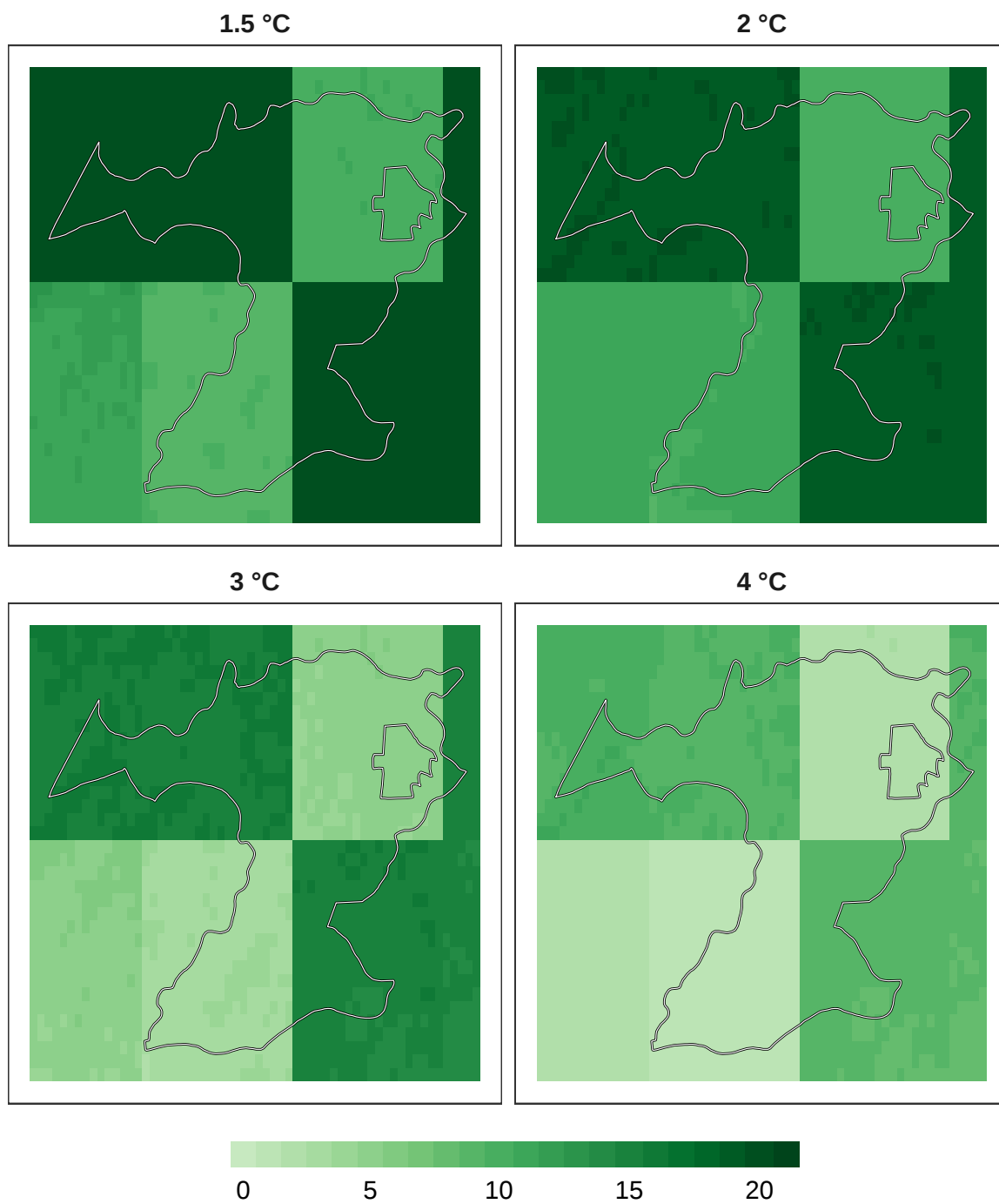
Figure 13: Number of models in agreement for reptile refugia at 1 km resolution.
