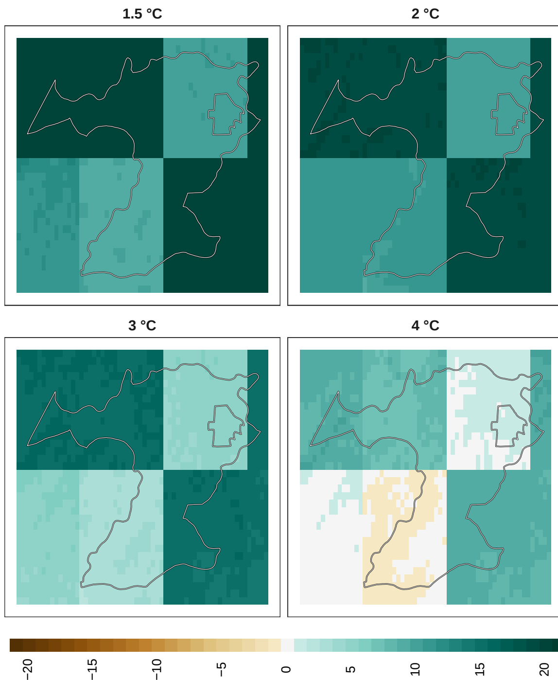
Figure 20: Adaptation effort for reptiles at 1 km resolution.
