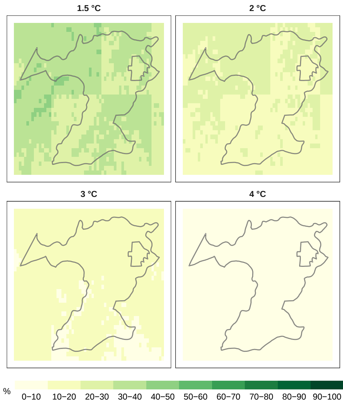
Figure 7: Percent pollinators remaining at 1 km resolution.
