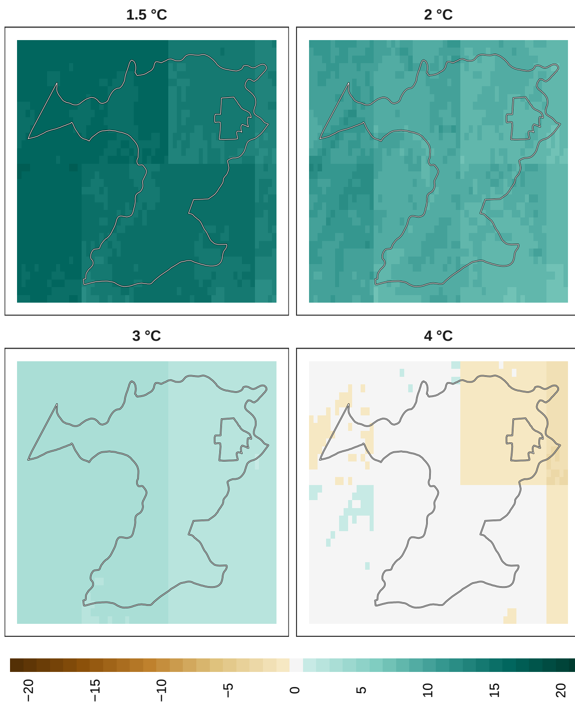
Figure 17: Adaptation effort for plants at 1 km resolution.
