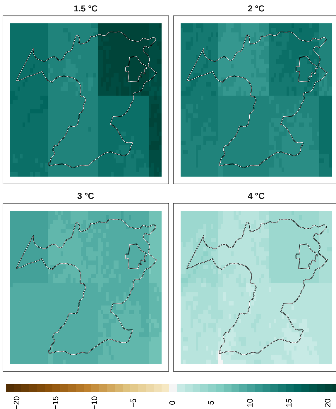
Figure 19: Adaptation effort for mammals at 1 km resolution.
