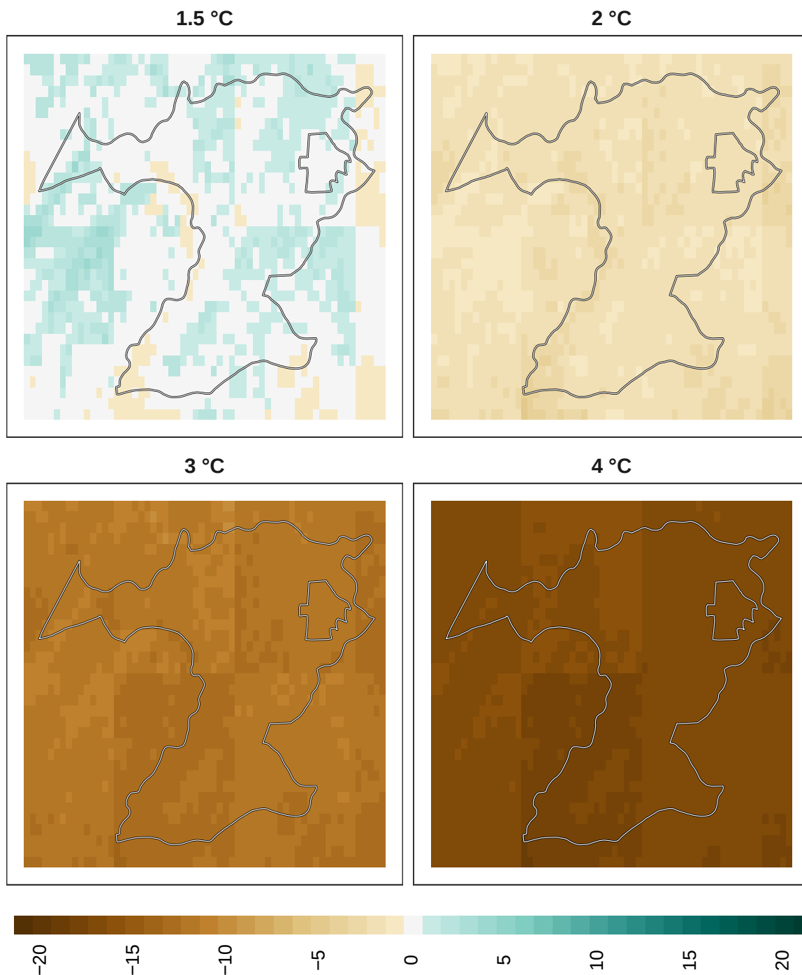
Figure 16: Adaptation effort for overall biodiversity at 1 km resolution.
