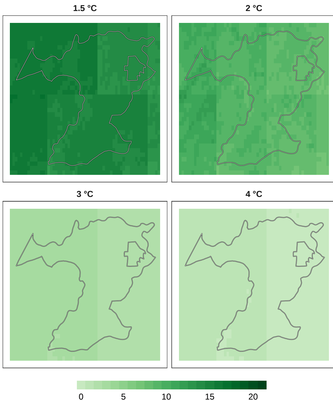
Figure 10: Number of models in agreement for plant refugia at 1 km resolution.
