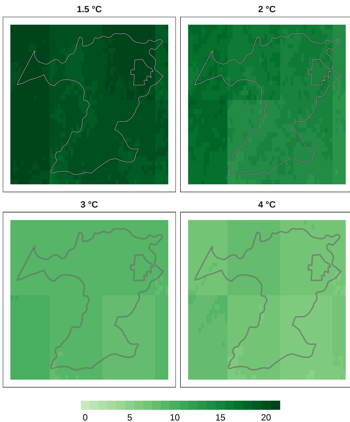
Figure 11: Number of models in agreement for bird refugia.
