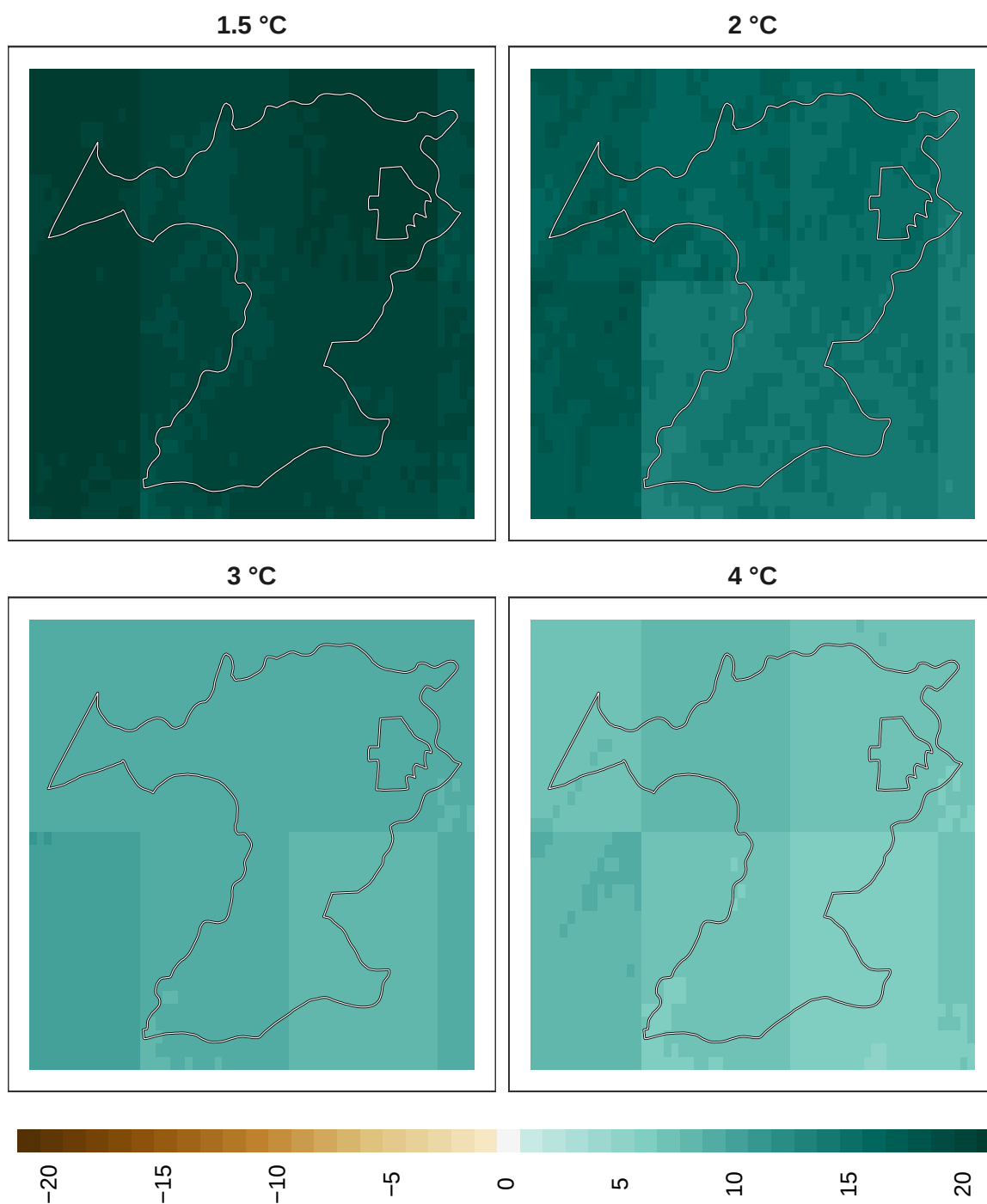
Figure 18: Adaptation effort for birds at 1 km resolution.
