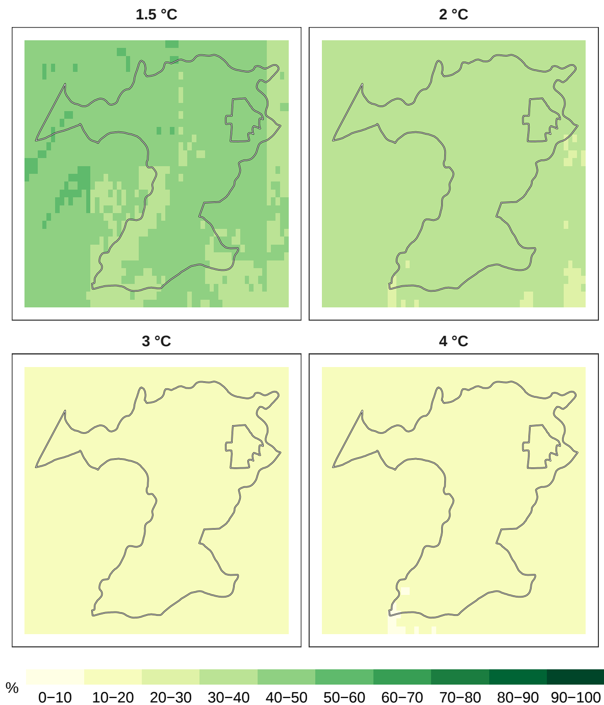
Figure 6: Percent insects remaining at 1 km resolution.
