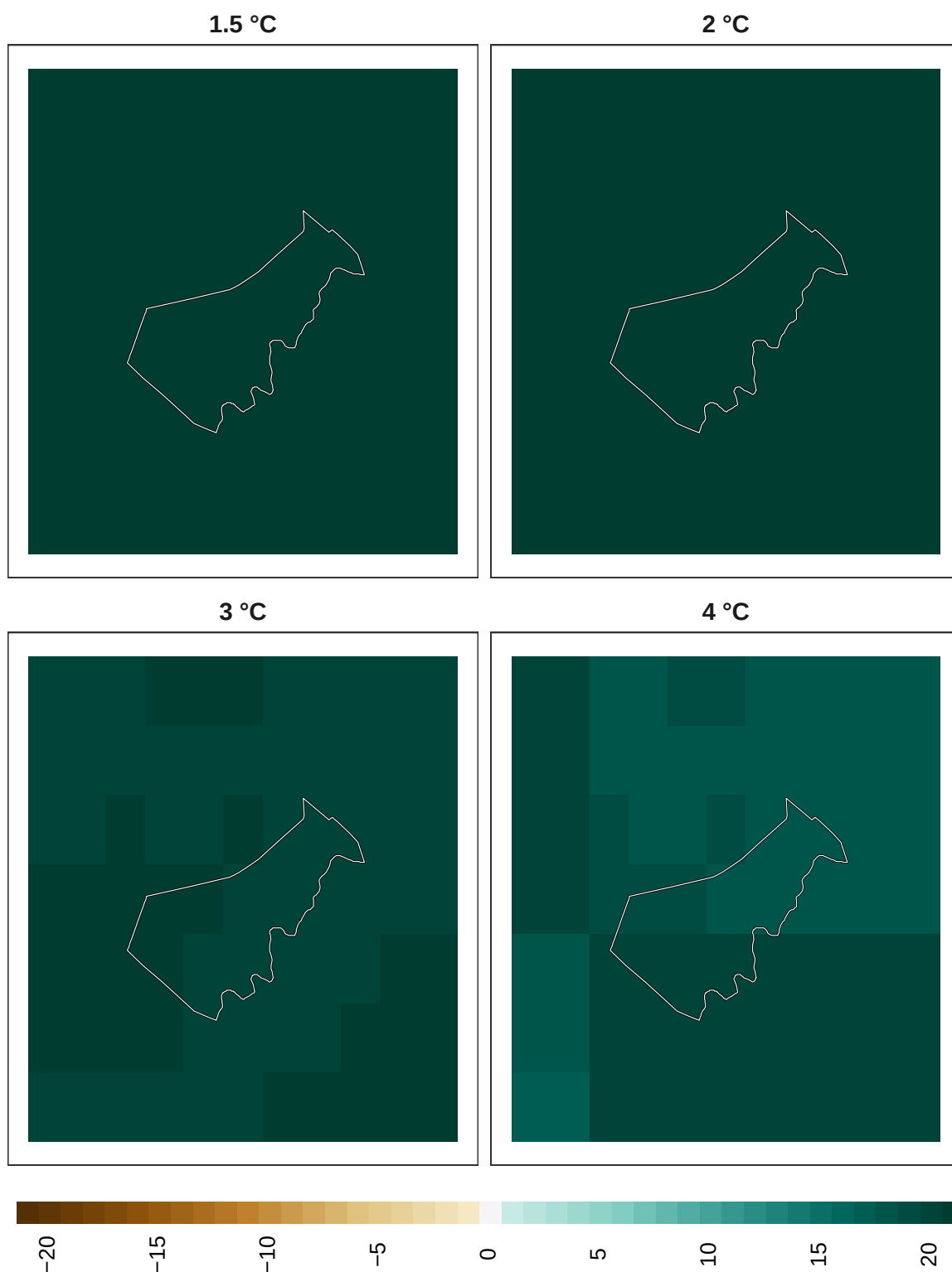
Figure 13: Adaptation effort for birds at 1 km resolution.
