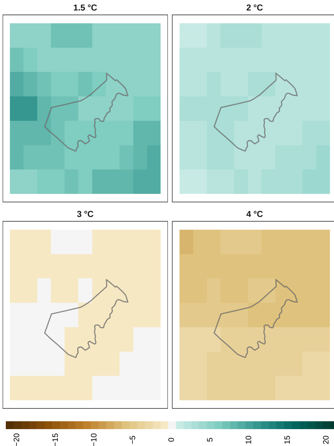
Figure 11: Adaptation effort for overall biodiversity at 1 km resolution.
