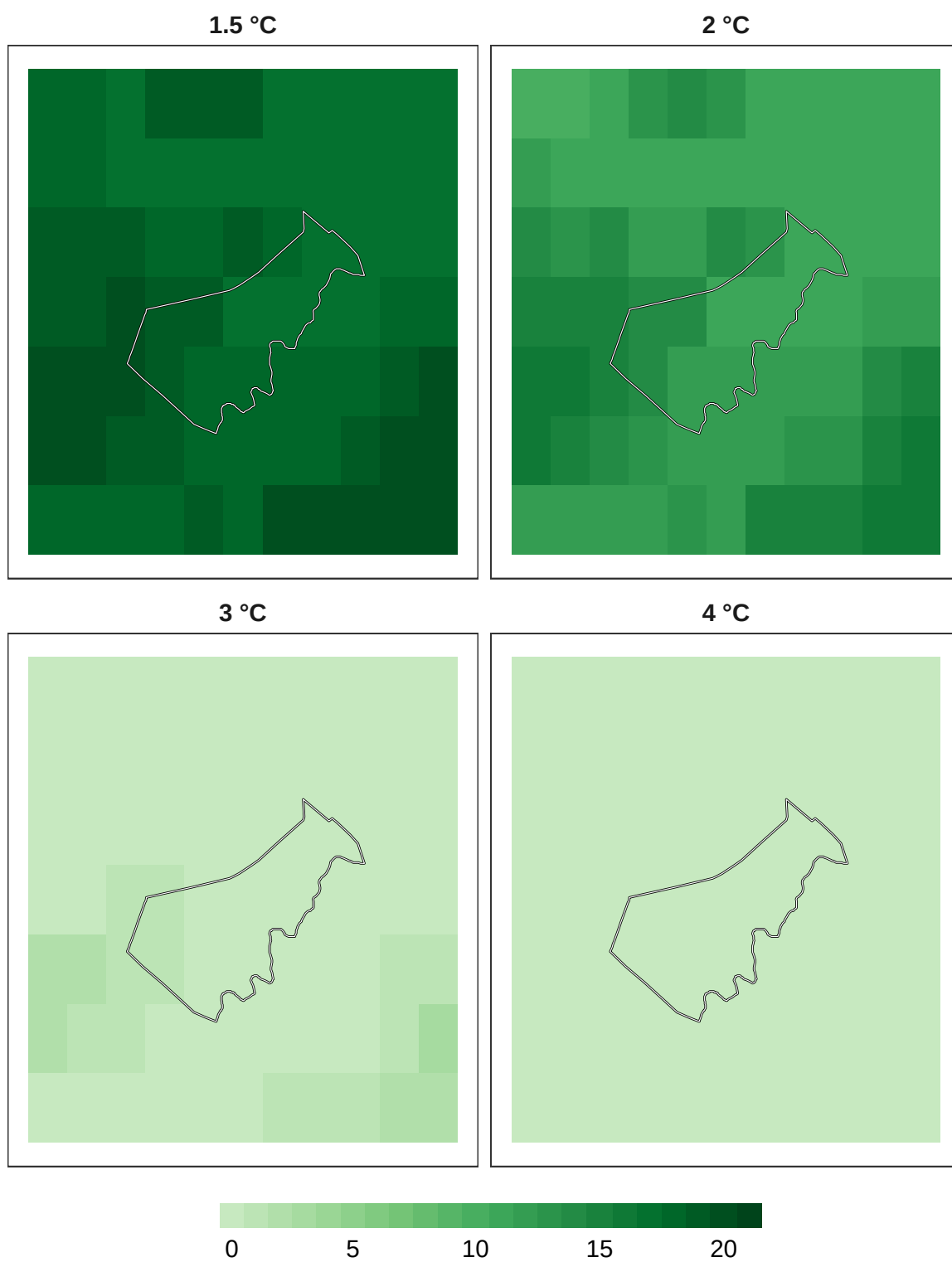
Figure 9: Number of models in agreement for mammal refugia at 1 km resolution.
