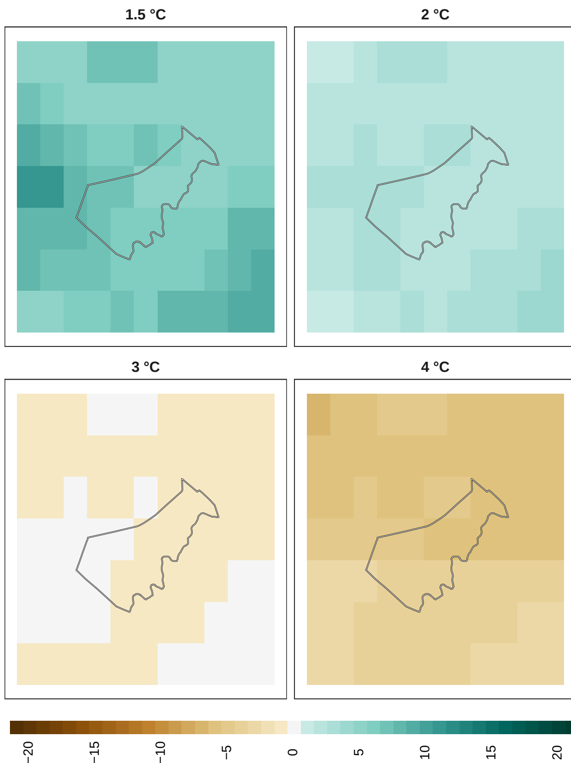
Figure 12: Adaptation effort for plants at 1 km resolution.
