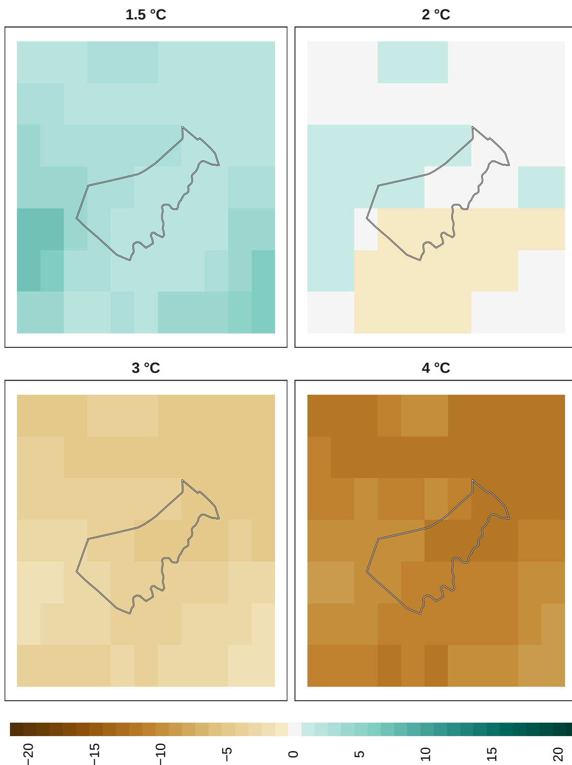
Figure 15: Adaptation effort for insects at 1 km resolution.
