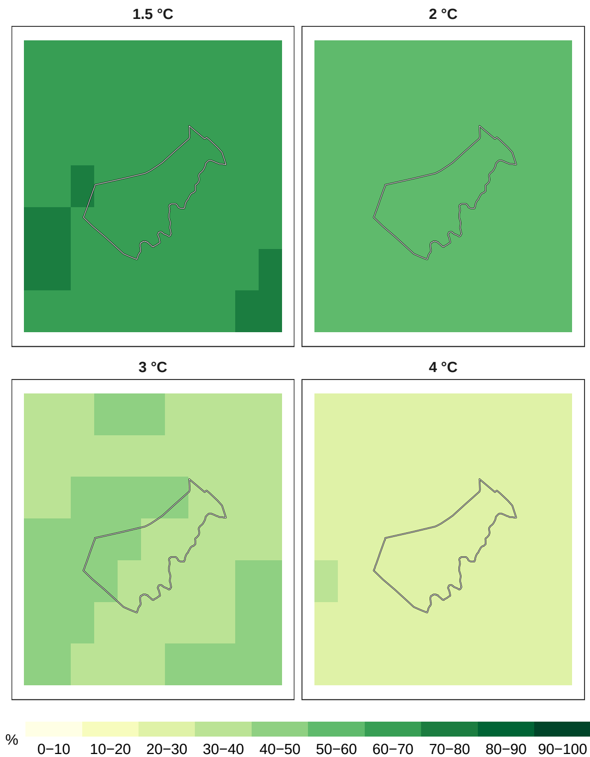
Figure 5: Percent insects remaining at 1 km resolution.
