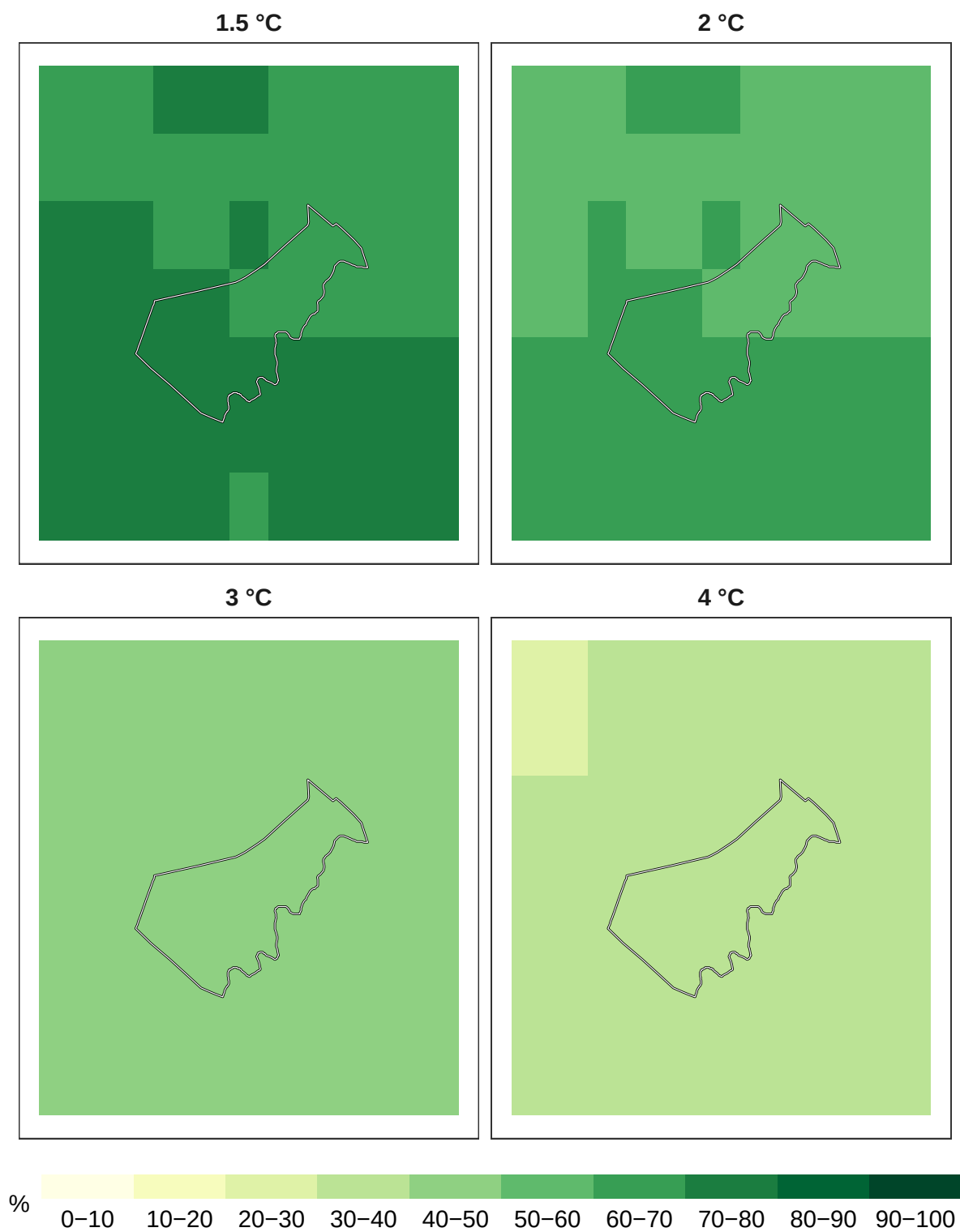
Figure 2: Percent plants remaining at 1 km resolution.
