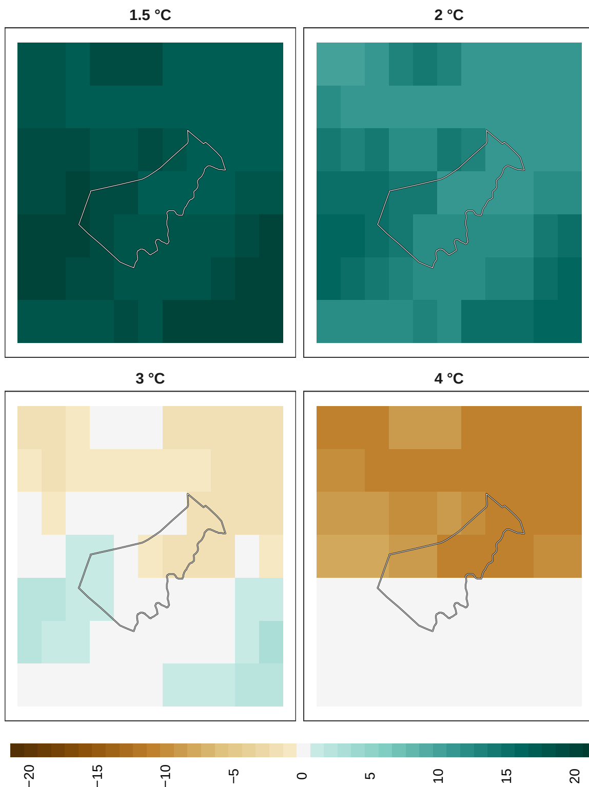
Figure 14: Adaptation effort for mammals at 1 km resolution.
