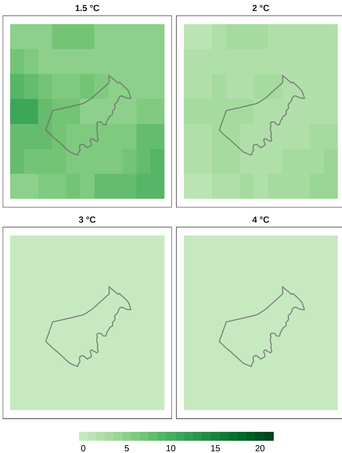
Figure 6: Number of models in agreement for overall biodiversity refugia at 1 km resolution.
