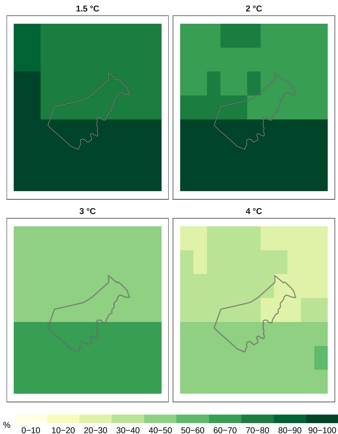
Figure 4: Percent mammals remaining at 1 km resolution.
