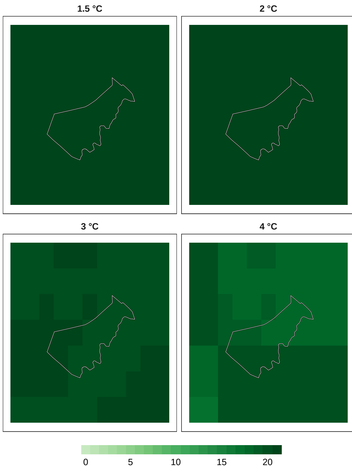
Figure 8: Number of models in agreement for bird refugia.
