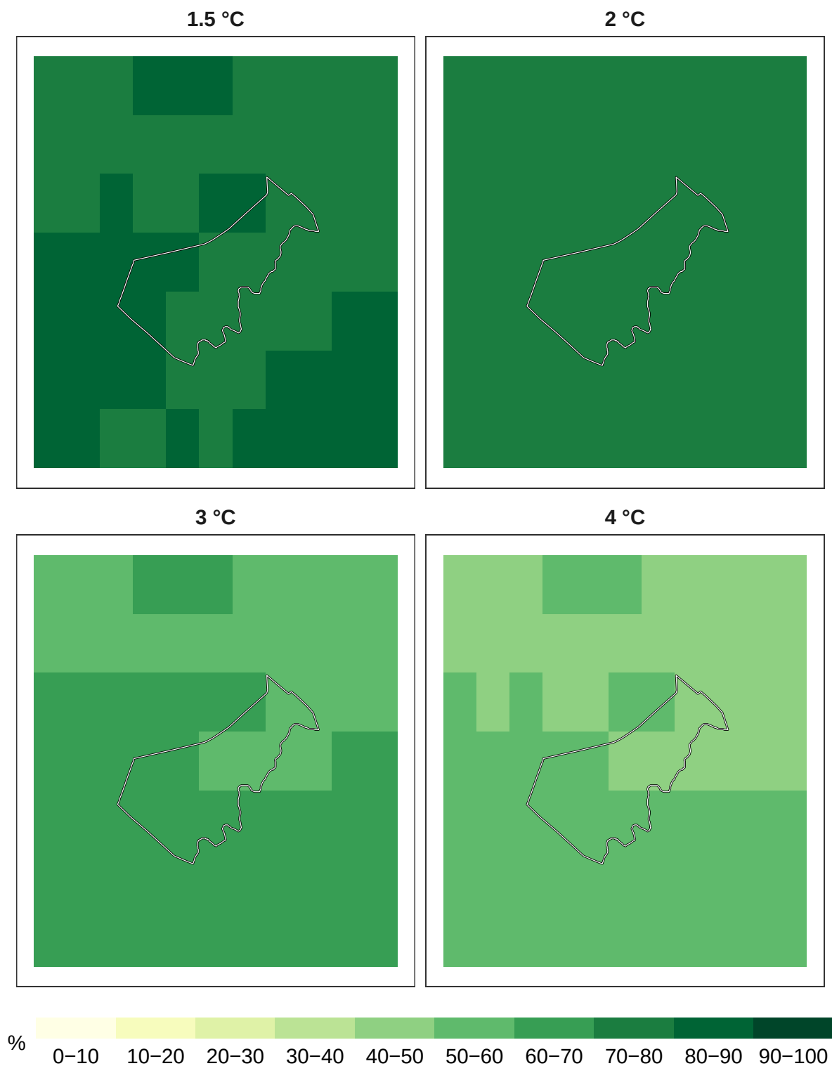
Figure 1: Percent overall biodiversity remaining at 1 km resolution.
