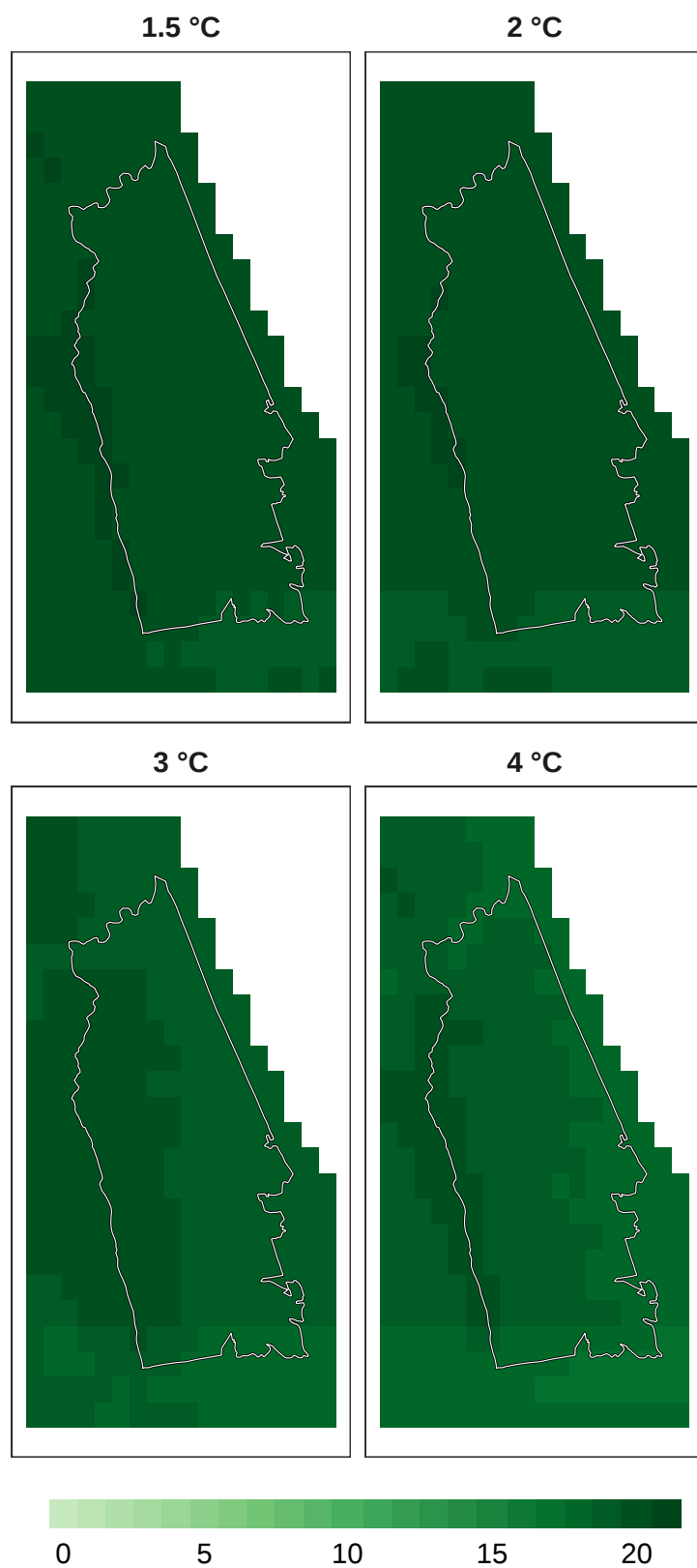
Figure 9: Number of models in agreement for bird refugia.
