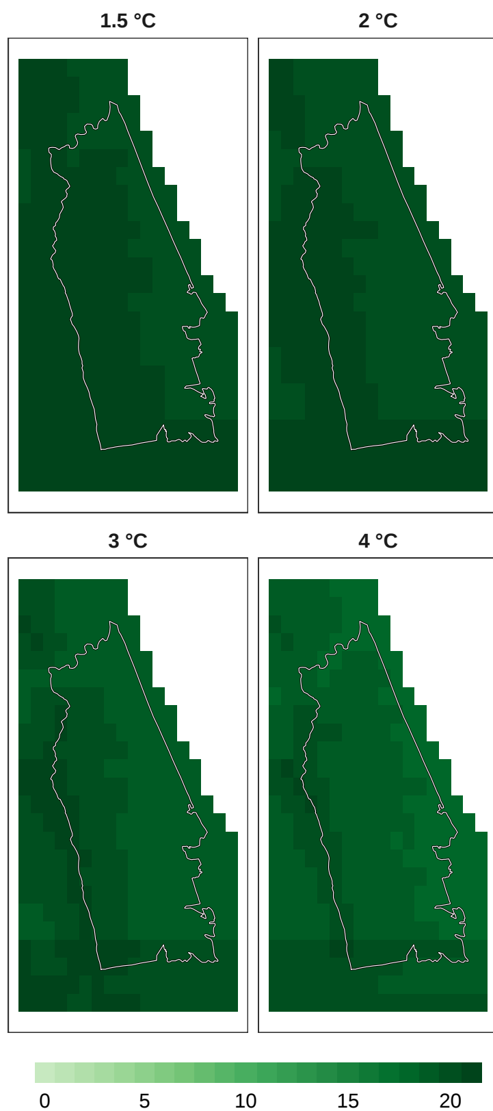
Figure 11: Number of models in agreement for insect refugia at 1 km resolution.
