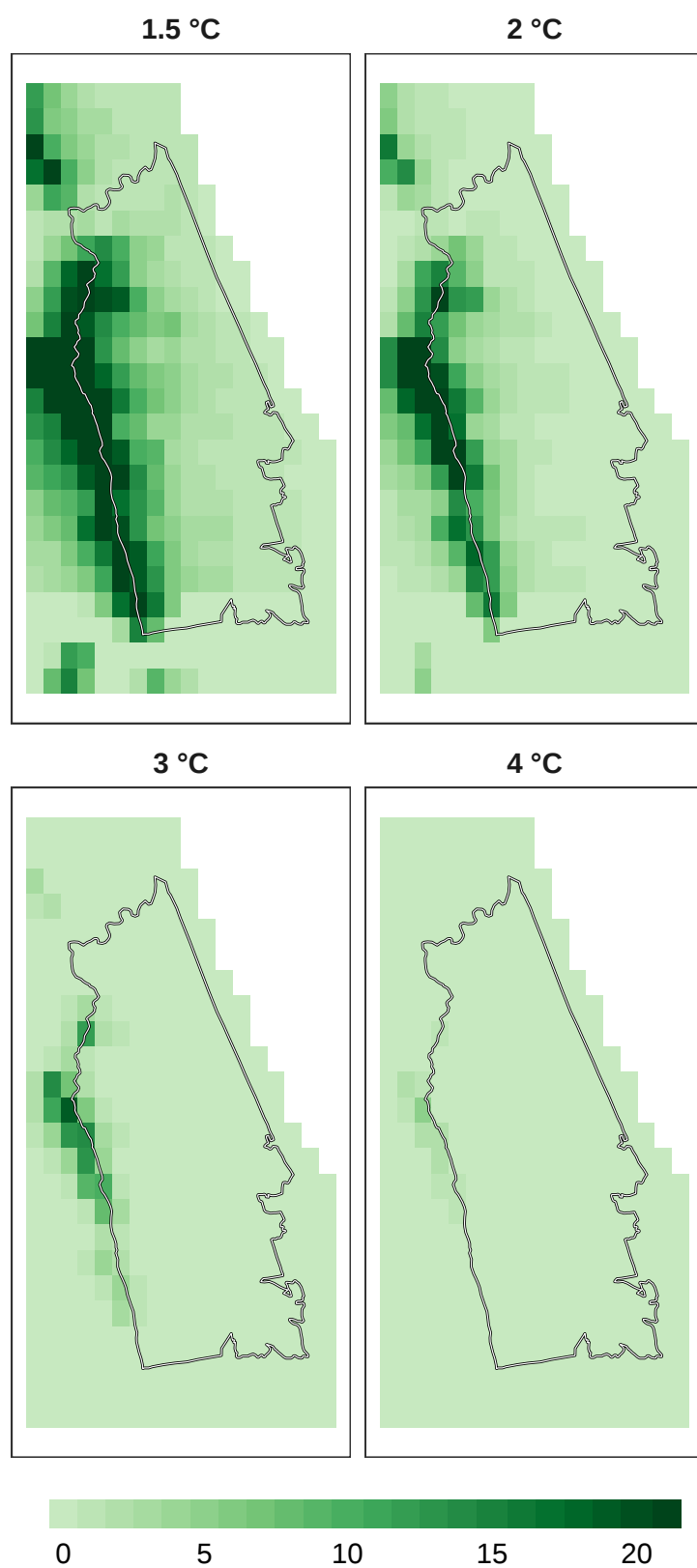
Figure 10: Number of models in agreement for mammal refugia at 1 km resolution.
