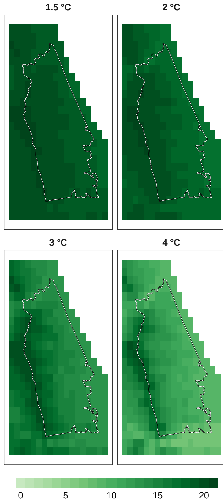
Figure 7: Number of models in agreement for overall biodiversity refugia at 1 km resolution.
