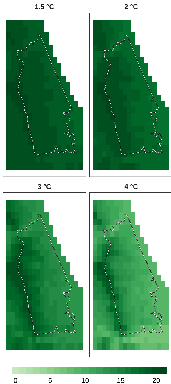
Figure 8: Number of models in agreement for plant refugia at 1 km resolution.
