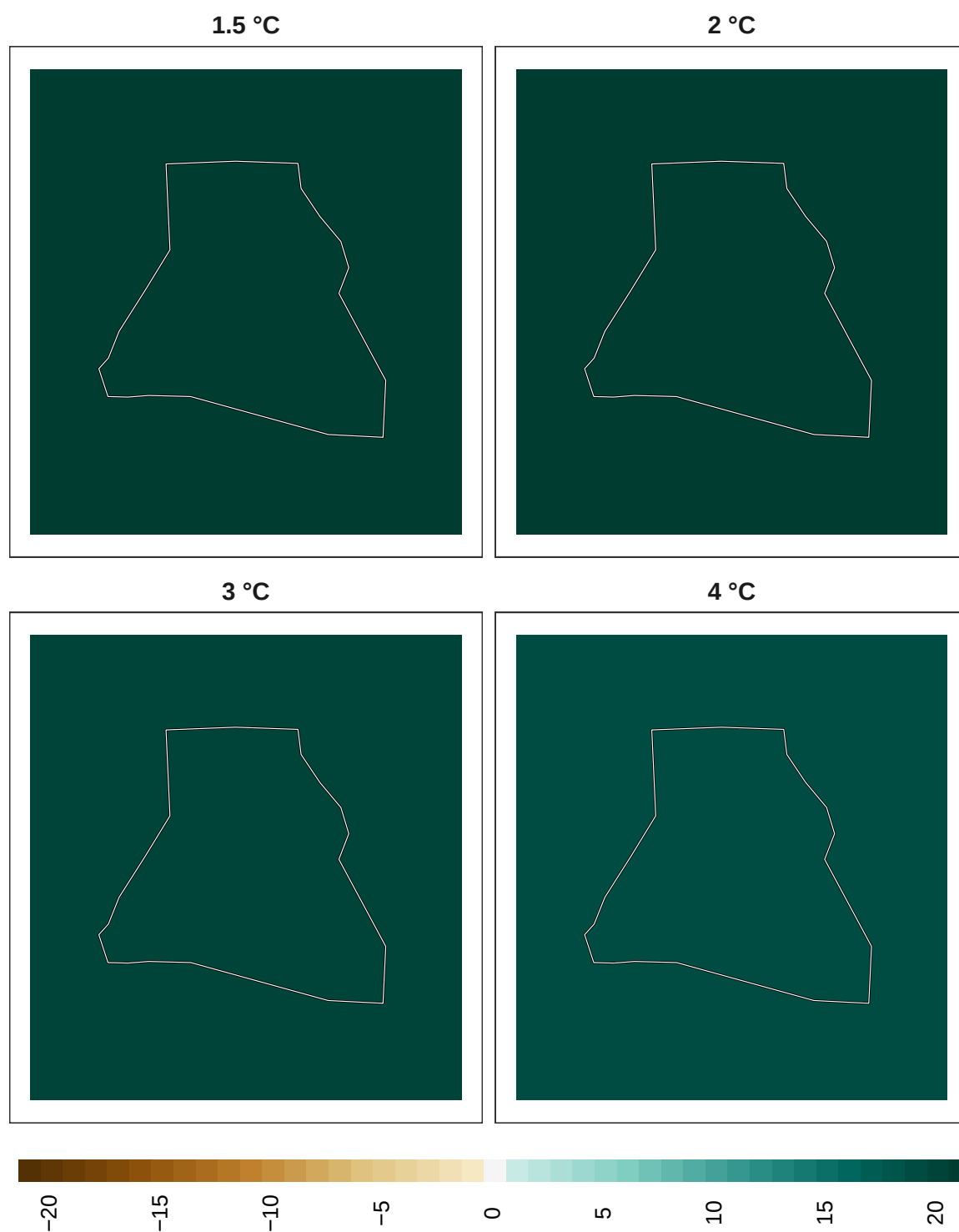
Figure 18: Adaptation effort for mammals at 1 km resolution.
