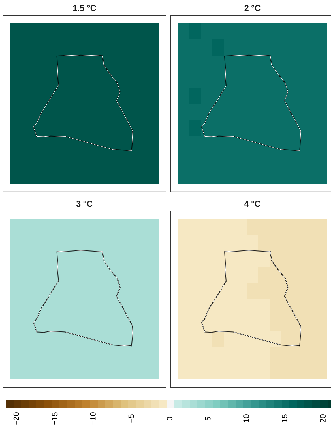
Figure 17: Adaptation effort for birds at 1 km resolution.
