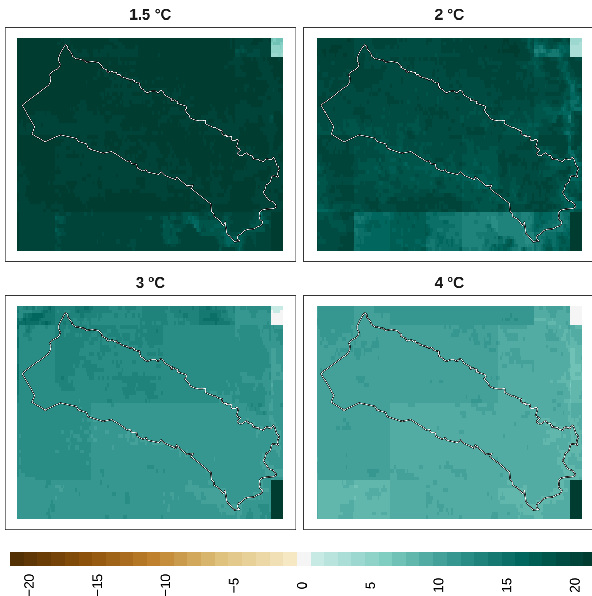
Figure 5: Adaptation effort for overall biodiversity at 1 km resolution.
