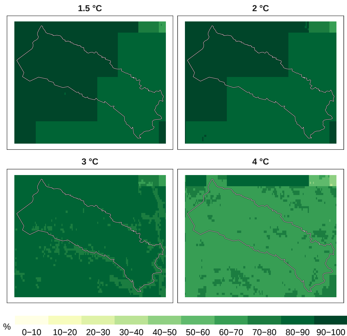
Figure 2: Percent mammals remaining at 1 km resolution.
