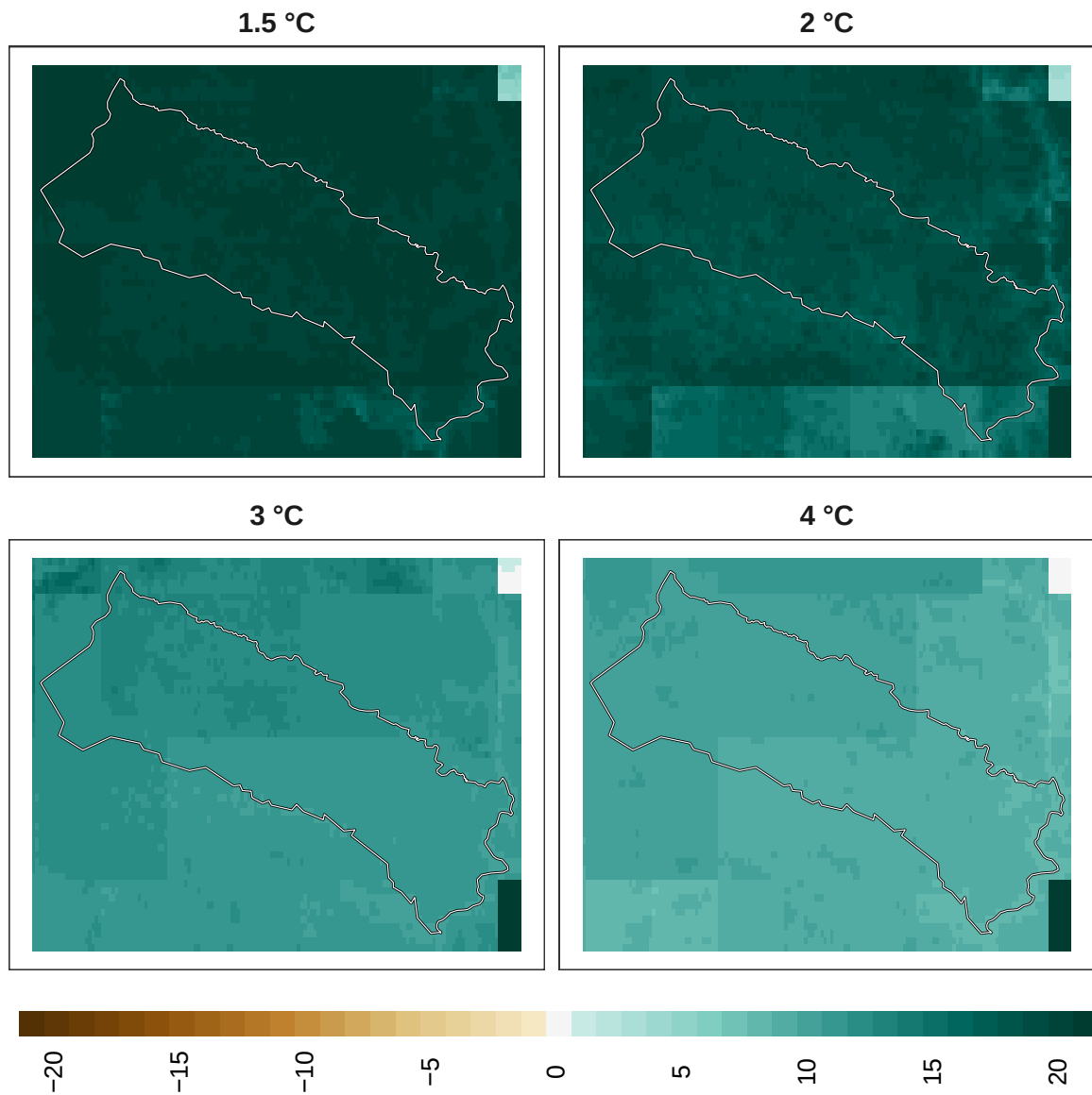
Figure 6: Adaptation effort for mammals at 1 km resolution.
