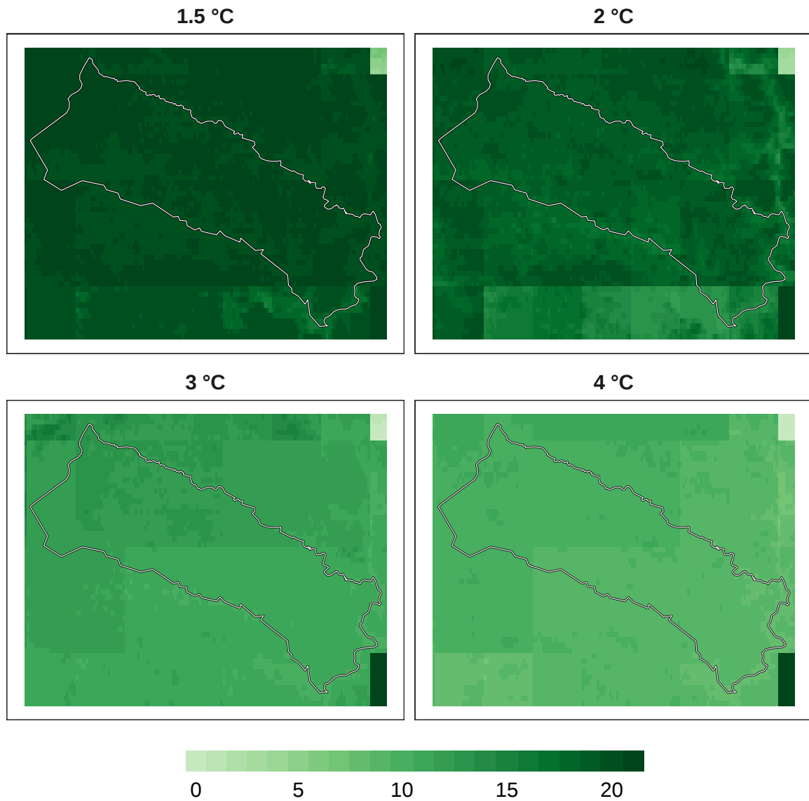
Figure 3: Number of models in agreement for overall biodiversity refugia at 1 km resolution.
