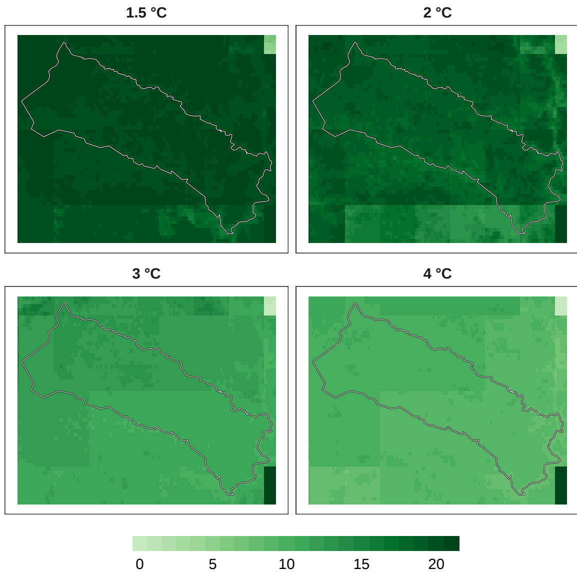
Figure 4: Number of models in agreement for mammal refugia at 1 km resolution.
