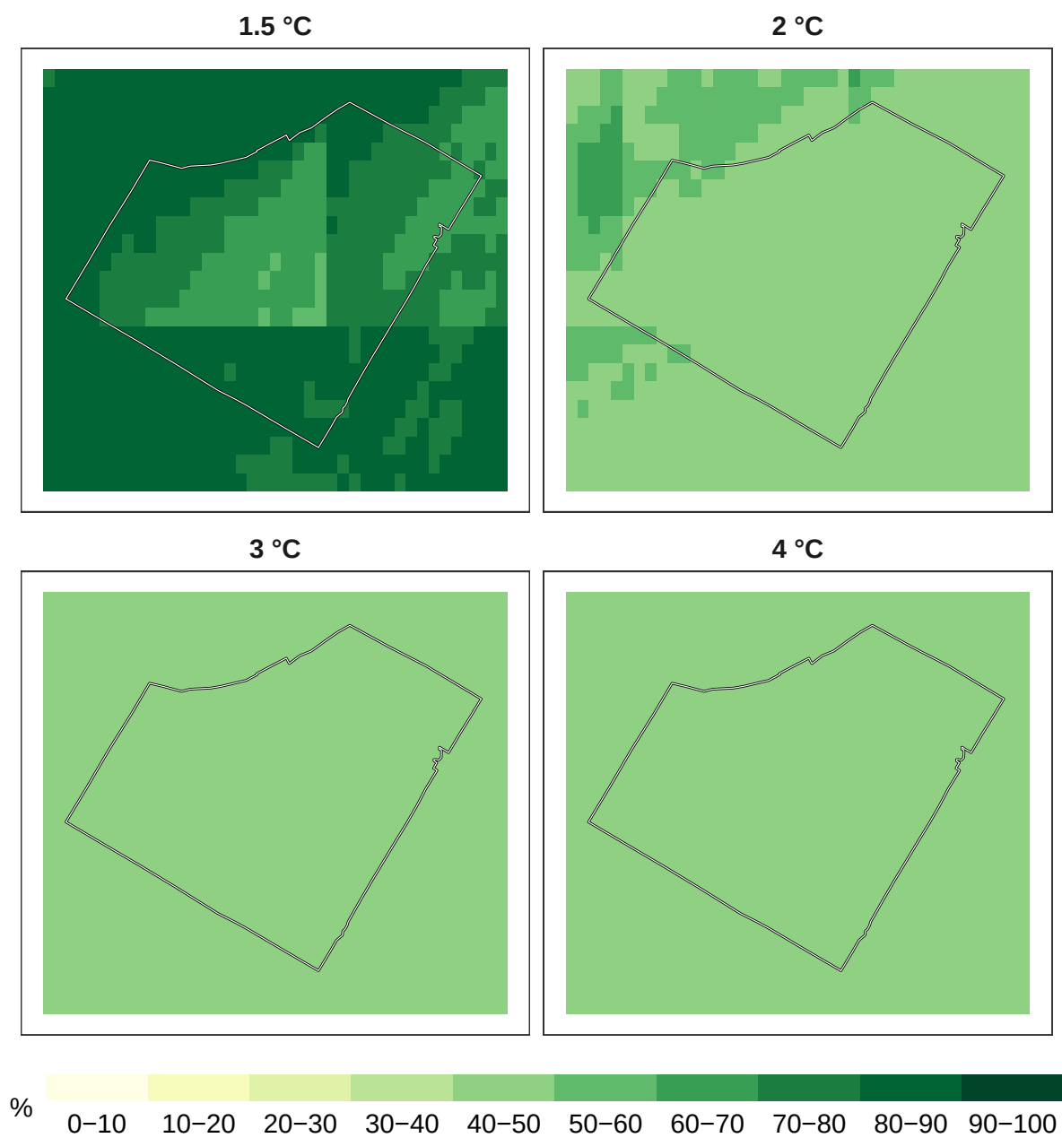
Figure 6: Percent insects remaining at 1 km resolution.
