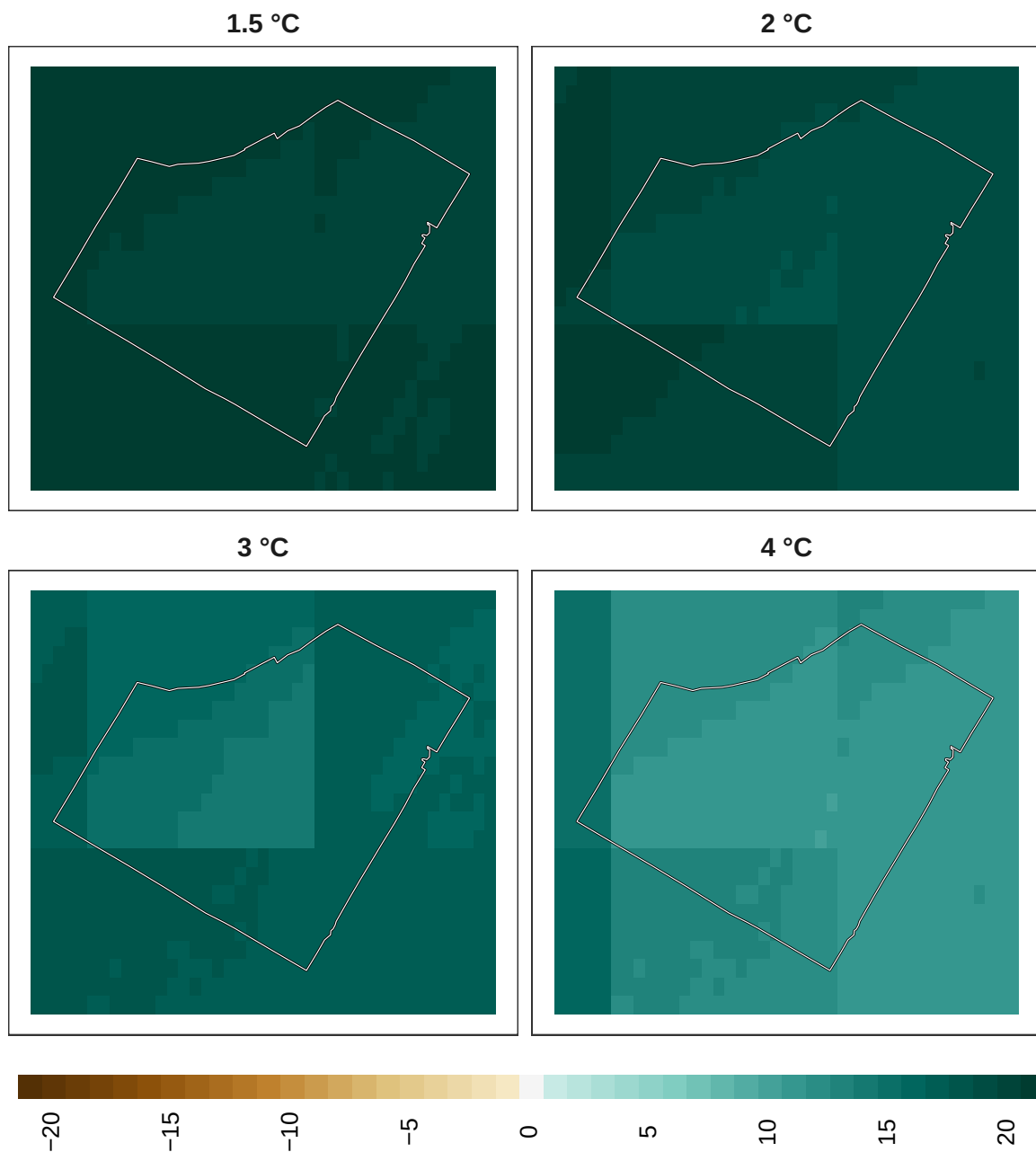
Figure 17: Adaptation effort for reptiles at 1 km resolution.
