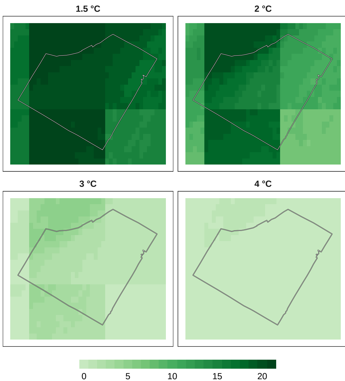
Figure 9: Number of models in agreement for bird refugia.
