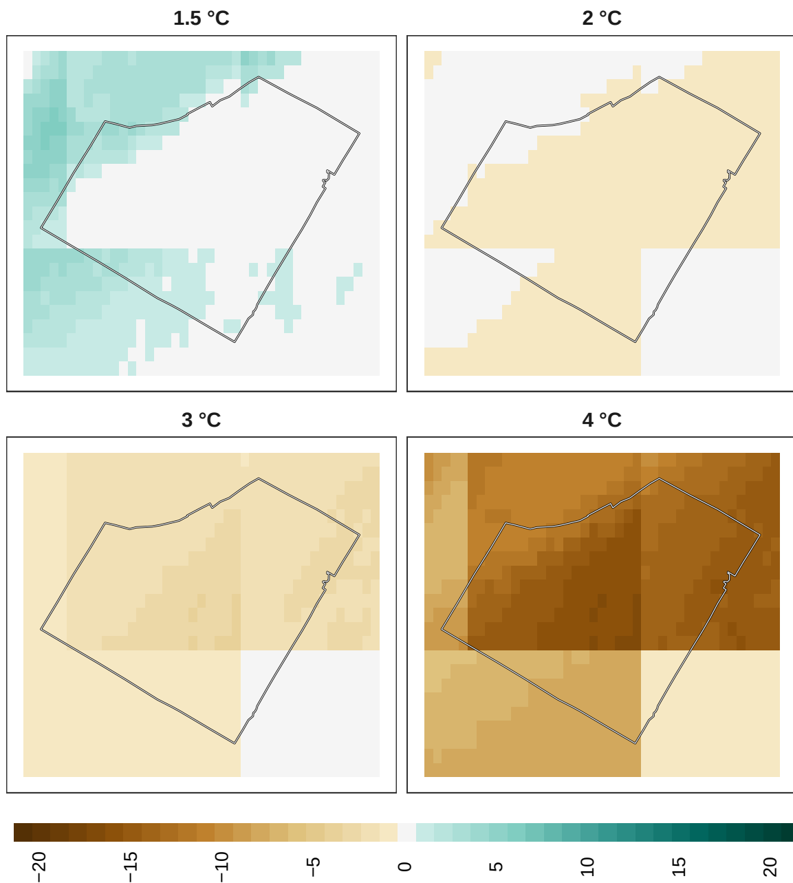
Figure 13: Adaptation effort for overall biodiversity at 1 km resolution.
