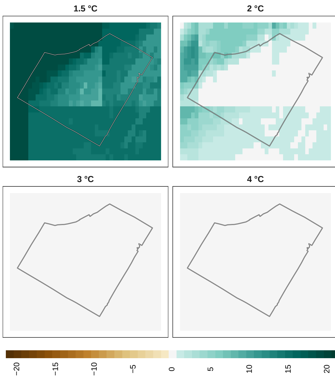
Figure 18: Adaptation effort for insects at 1 km resolution.
