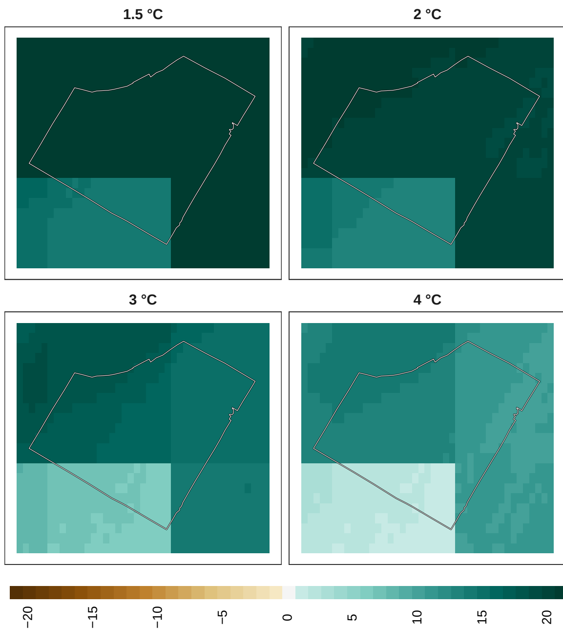
Figure 16: Adaptation effort for mammals at 1 km resolution.
