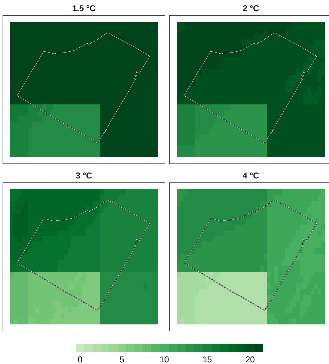
Figure 10: Number of models in agreement for mammal refugia at 1 km resolution.
