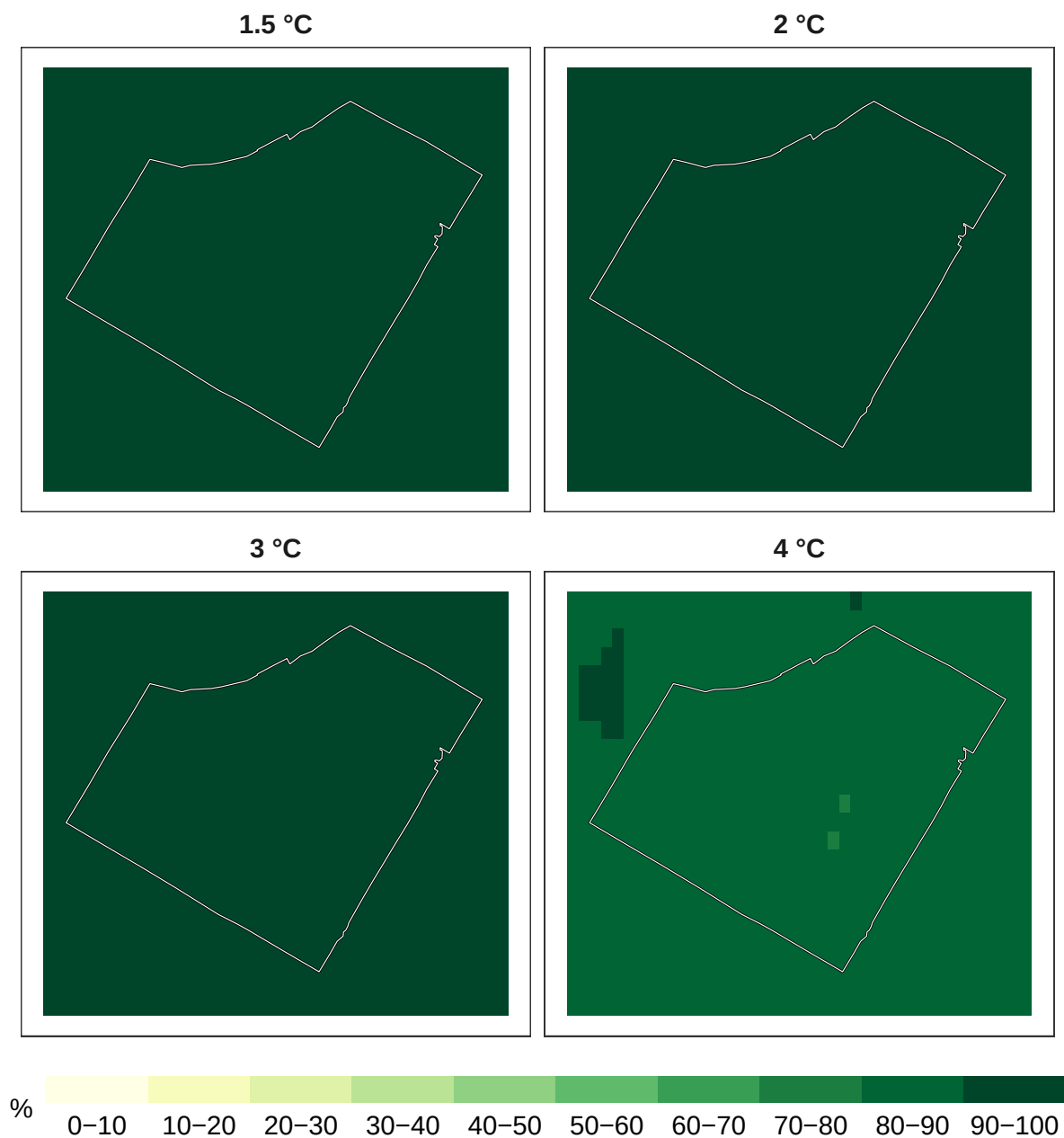
Figure 5: Percent reptiles remaining at 1 km resolution.
