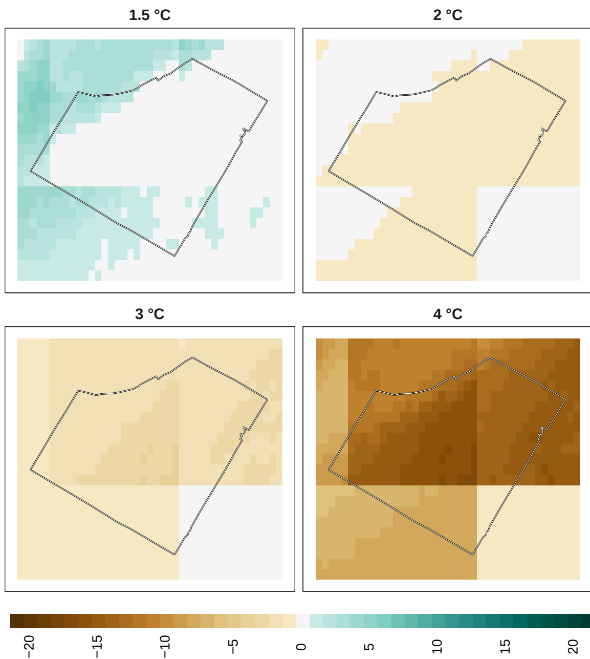
Figure 14: Adaptation effort for plants at 1 km resolution.
