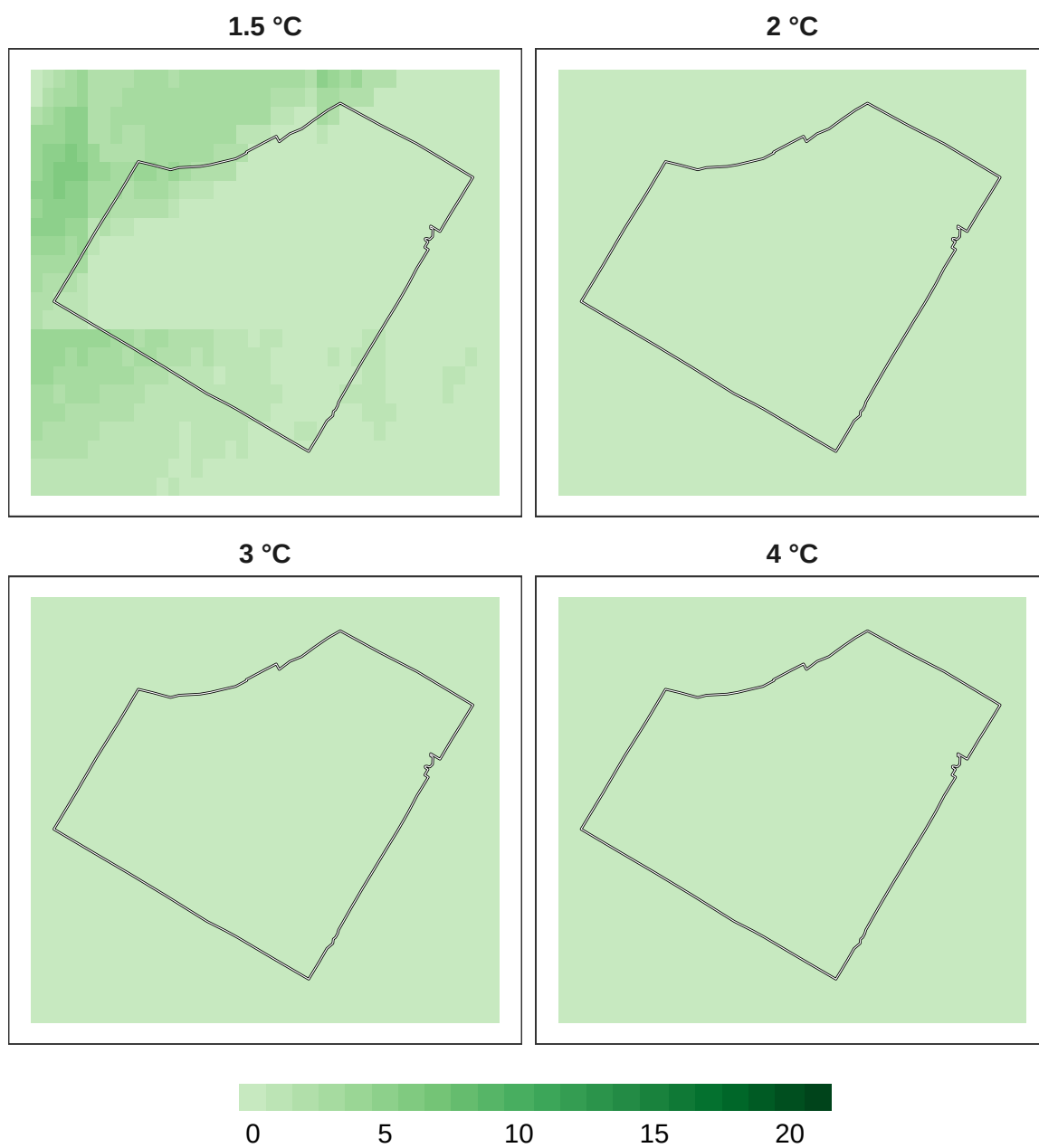
Figure 8: Number of models in agreement for plant refugia at 1 km resolution.
