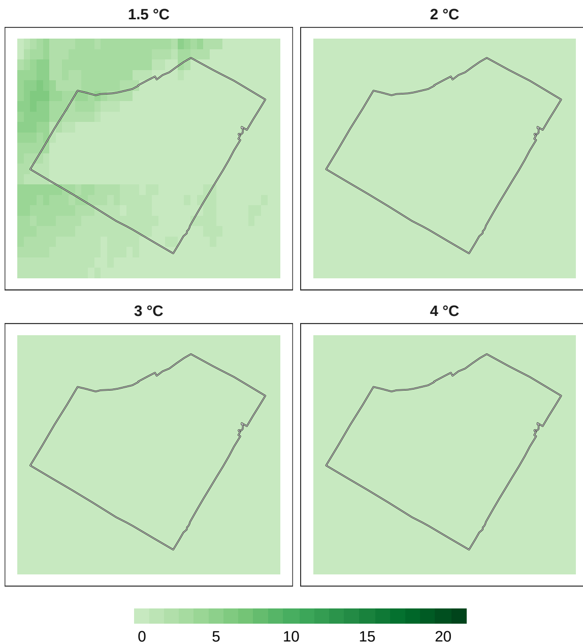
Figure 7: Number of models in agreement for overall biodiversity refugia at 1 km resolution.
