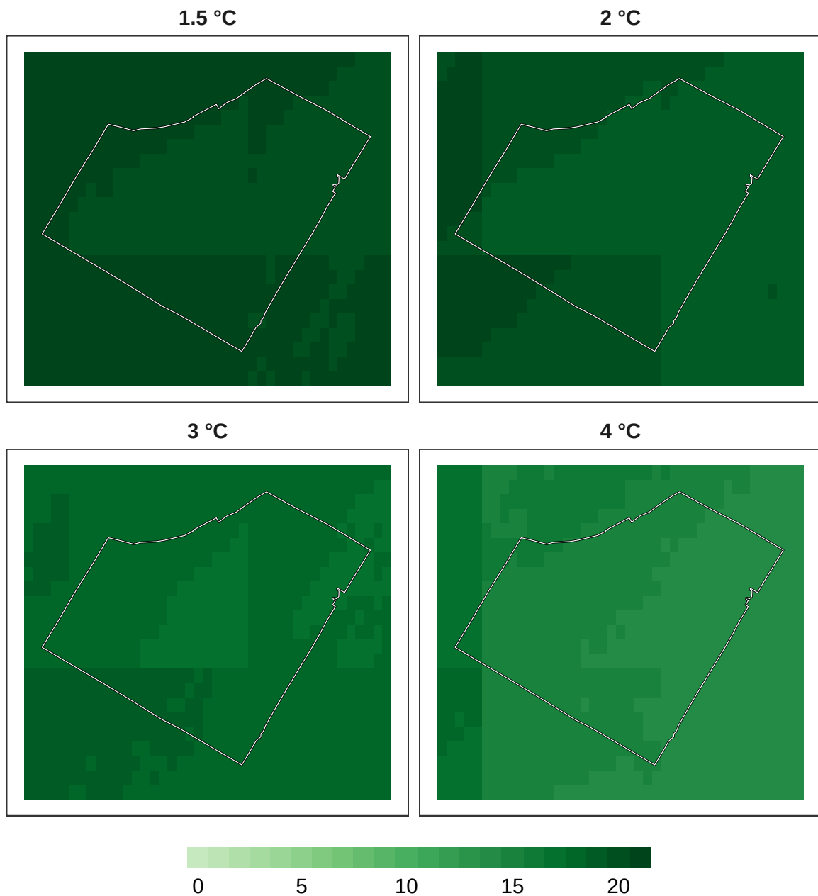
Figure 11: Number of models in agreement for reptile refugia at 1 km resolution.
