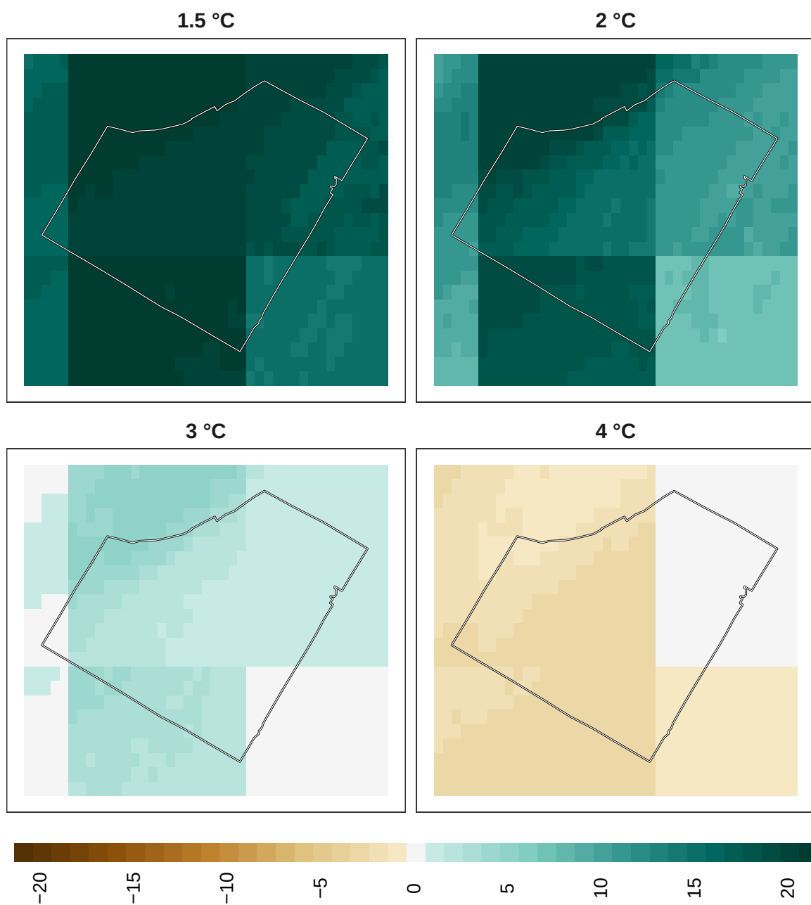
Figure 15: Adaptation effort for birds at 1 km resolution.
