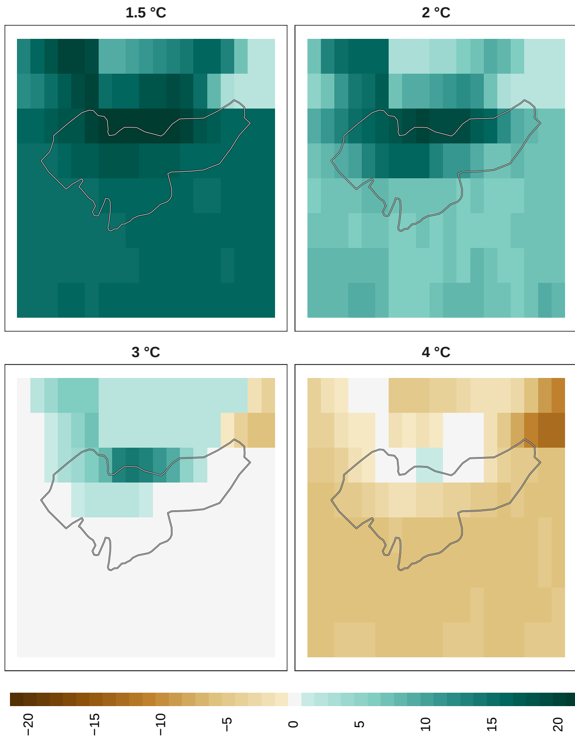
Figure 12: Adaptation effort for insects at 1 km resolution.
