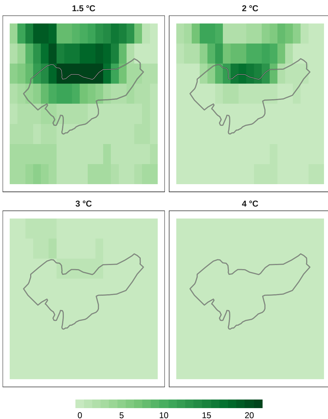
Figure 7: Number of models in agreement for mammal refugia at 1 km resolution.
