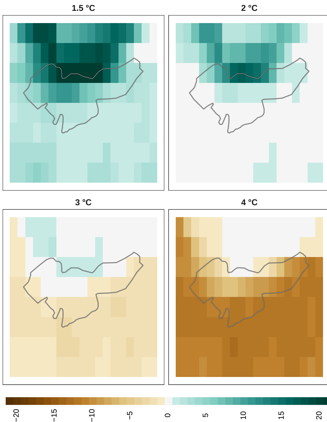
Figure 11: Adaptation effort for mammals at 1 km resolution.
