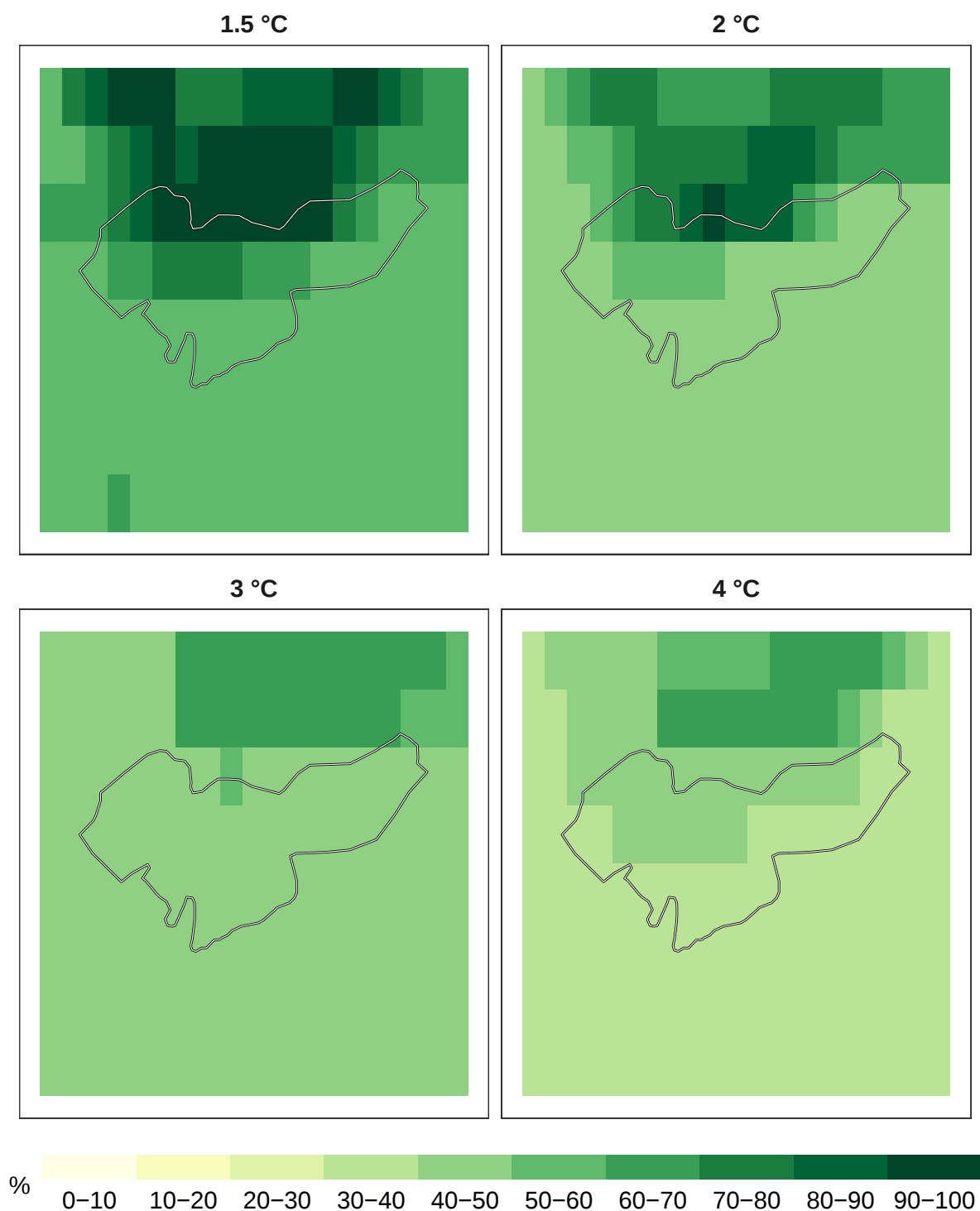
Figure 3: Percent mammals remaining at 1 km resolution.
