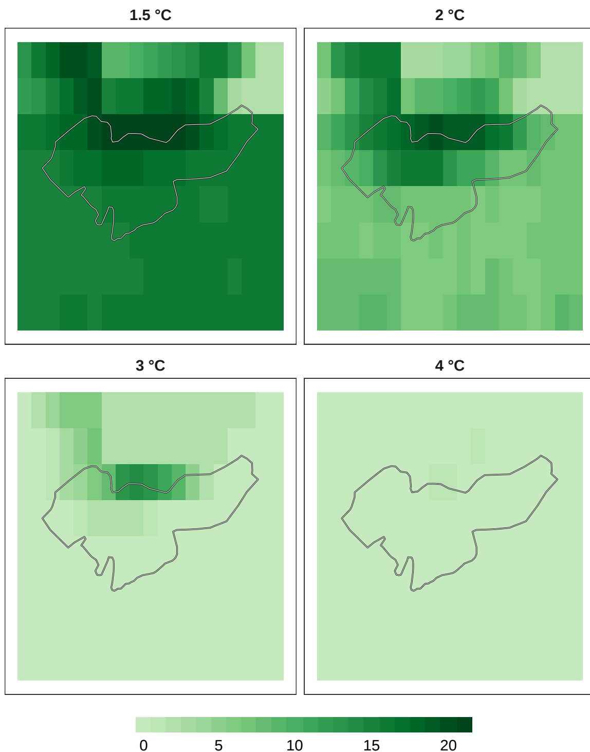
Figure 8: Number of models in agreement for insect refugia at 1 km resolution.
