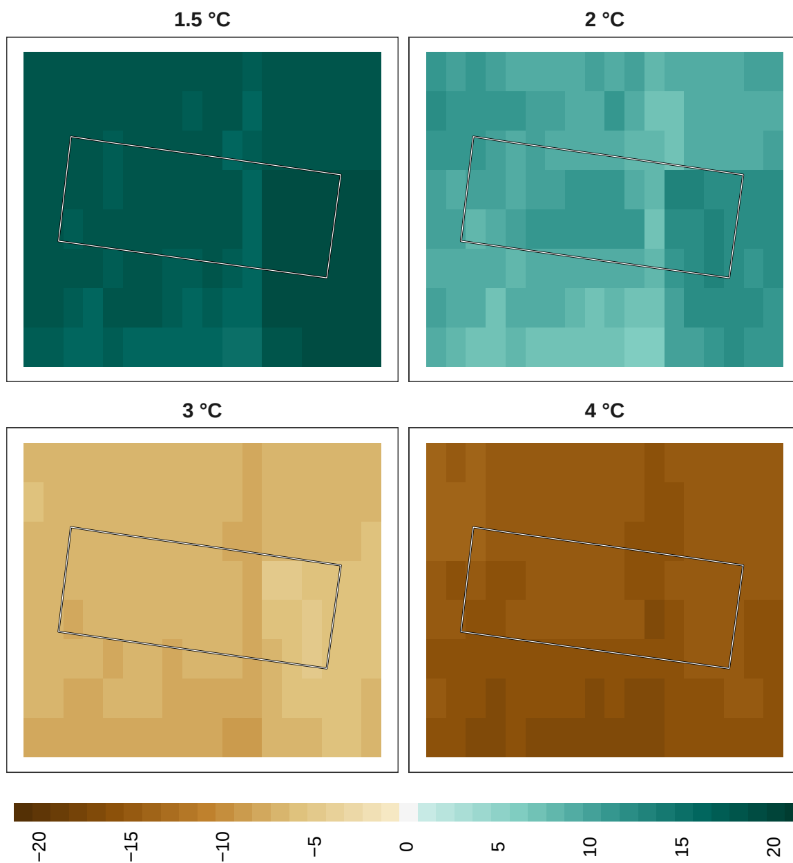
Figure 19: Adaptation effort for pollinators at 1 km resolution.
