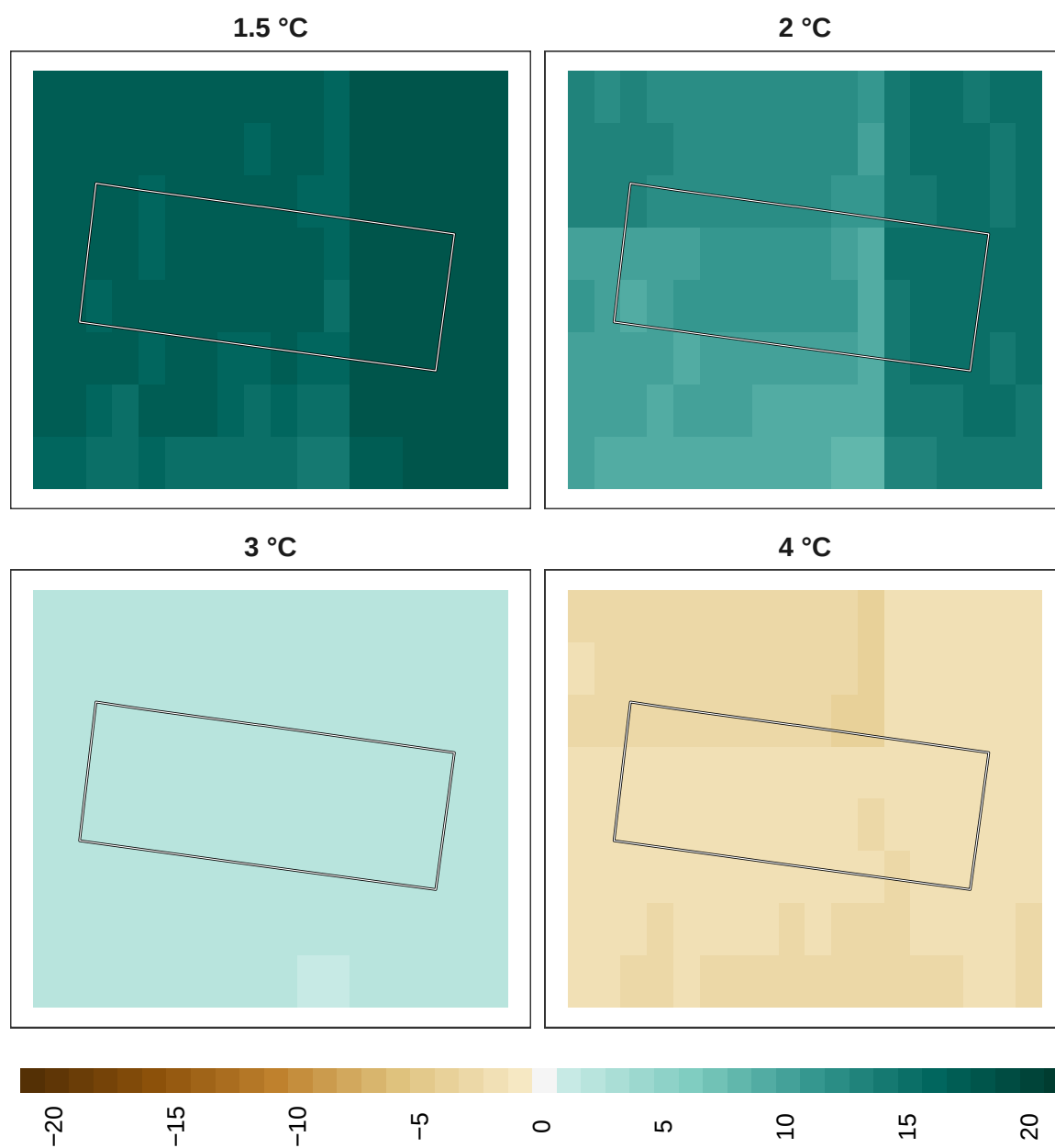
Figure 15: Adaptation effort for plants at 1 km resolution.
