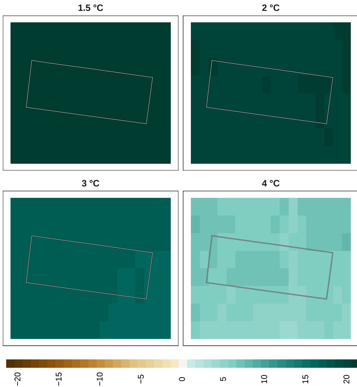
Figure 17: Adaptation effort for mammals at 1 km resolution.
