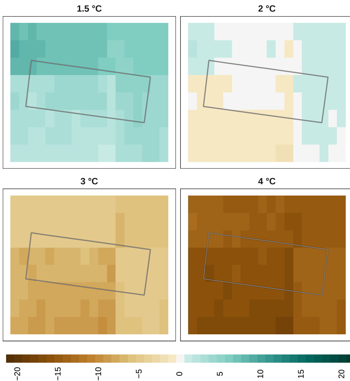
Figure 18: Adaptation effort for insects at 1 km resolution.
