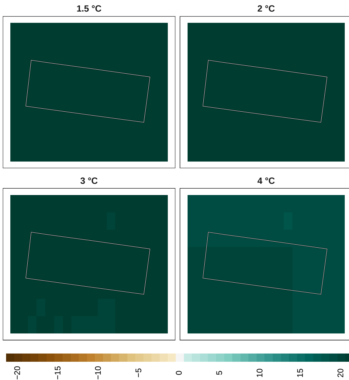
Figure 16: Adaptation effort for birds at 1 km resolution.
