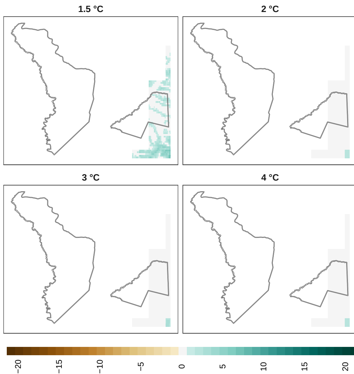
Figure 8: Adaptation effort for plants at 1 km resolution.
