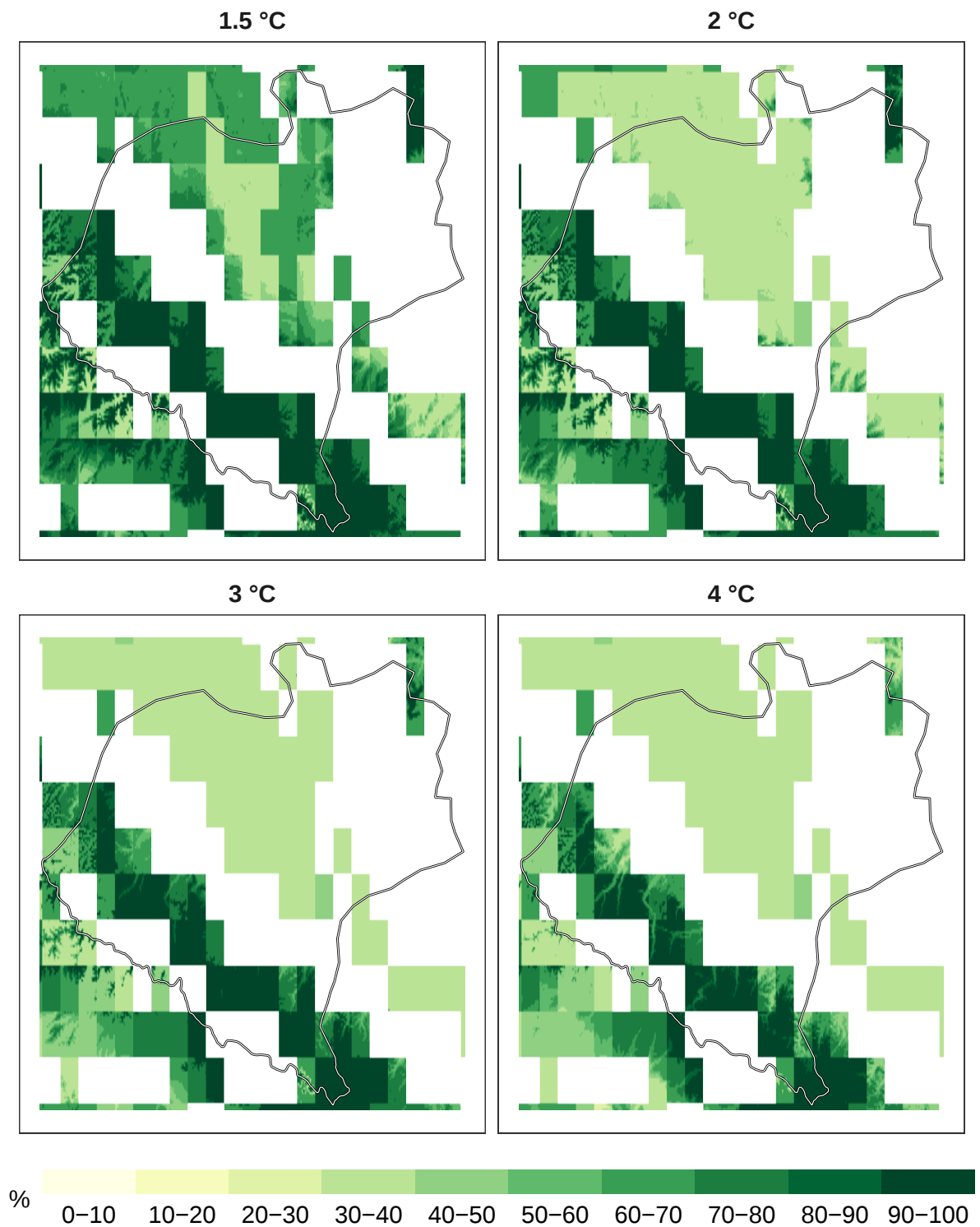
Figure 3: Percent mammals remaining at 1 km resolution.
