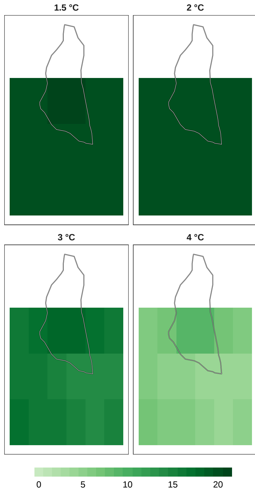
Figure 7: Number of models in agreement for mammal refugia at 1 km resolution.
