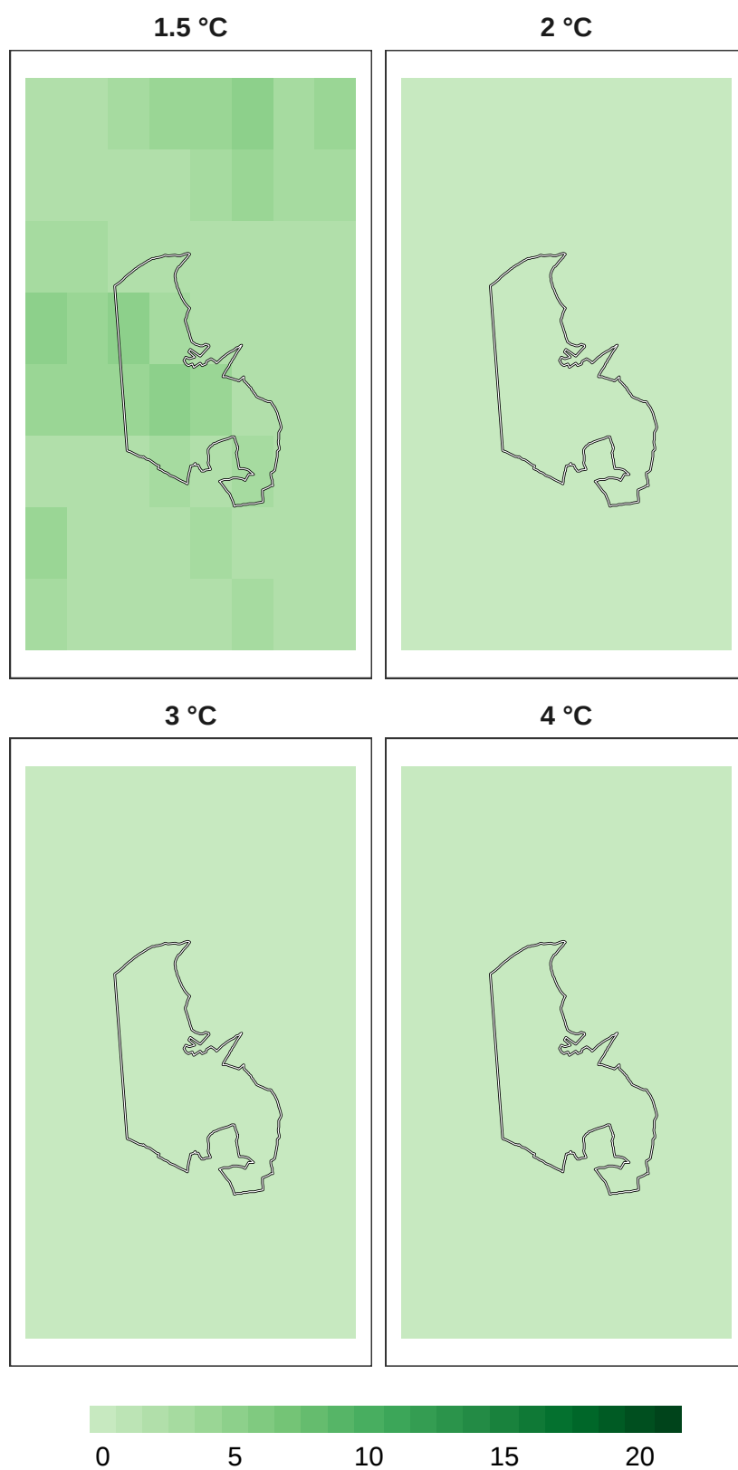
Figure 12: Number of models in agreement for insect refugia at 1 km resolution.
