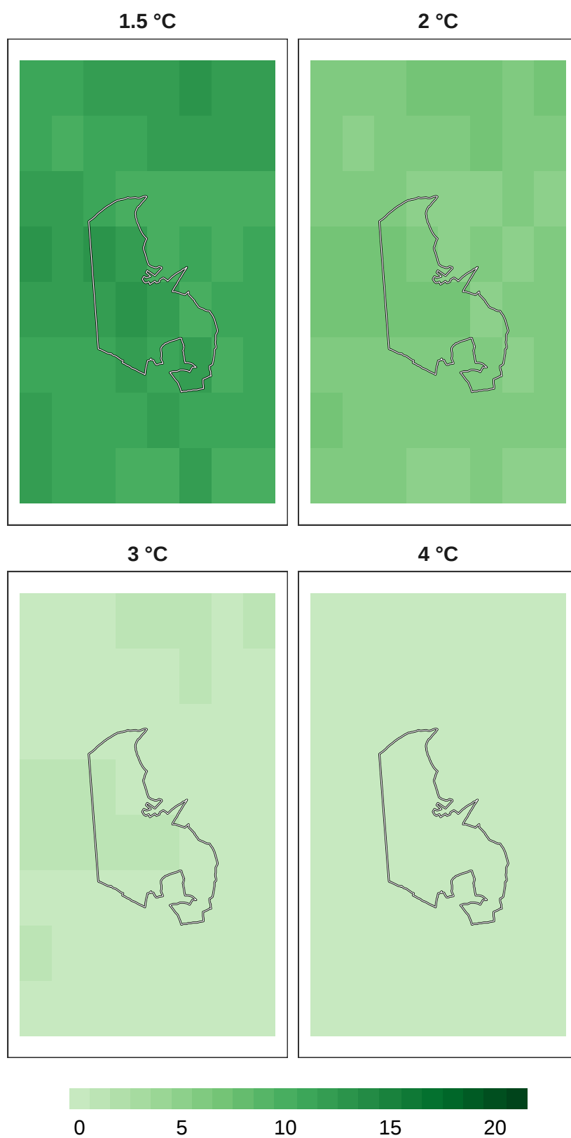
Figure 11: Number of models in agreement for mammal refugia at 1 km resolution.
