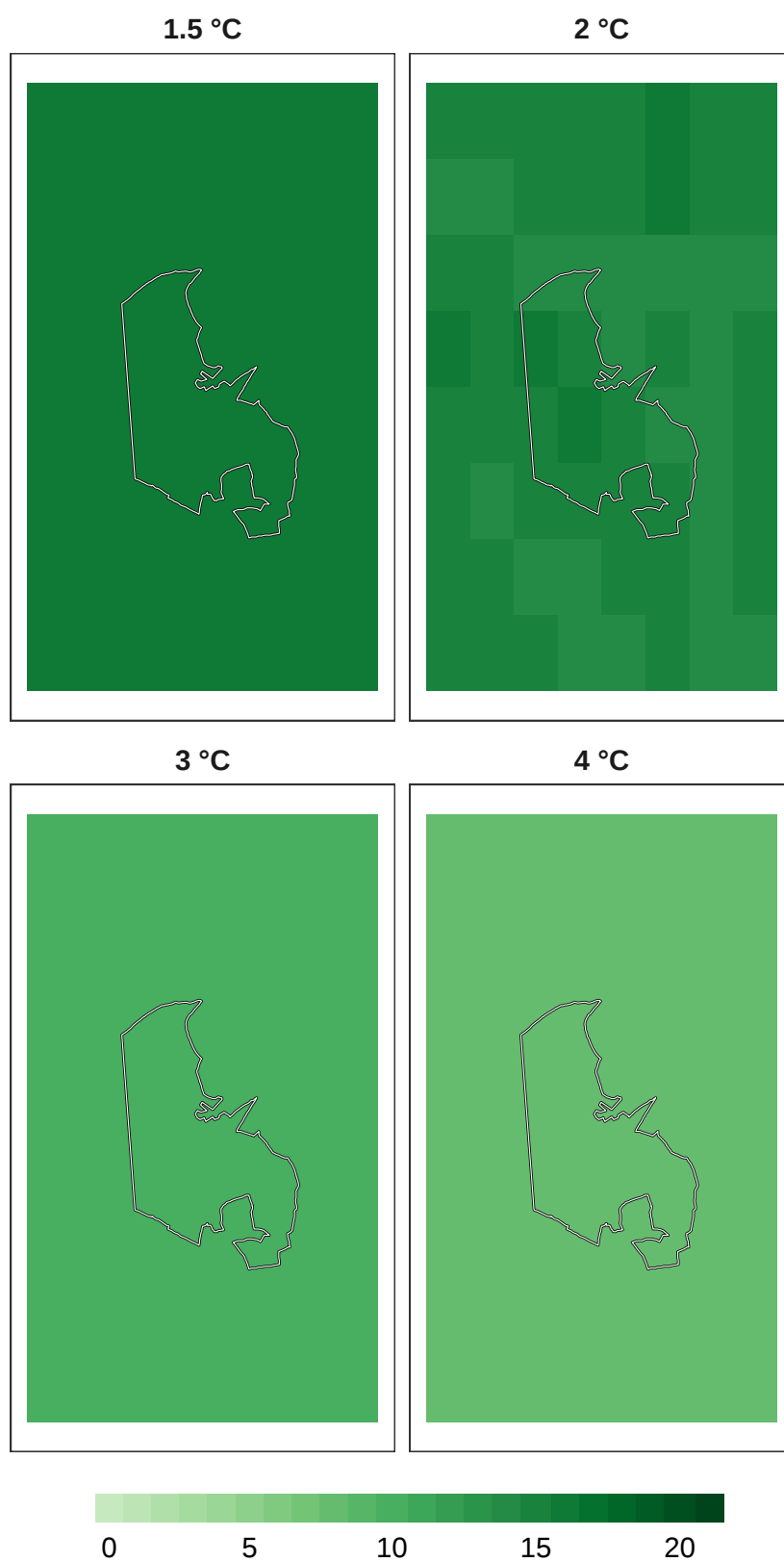
Figure 10: Number of models in agreement for bird refugia.
