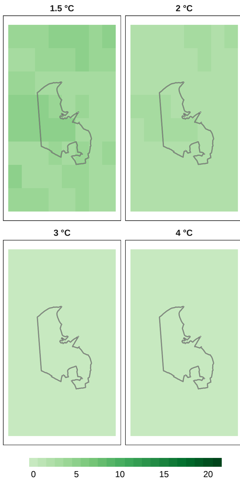
Figure 8: Number of models in agreement for overall biodiversity refugia at 1 km resolution.
