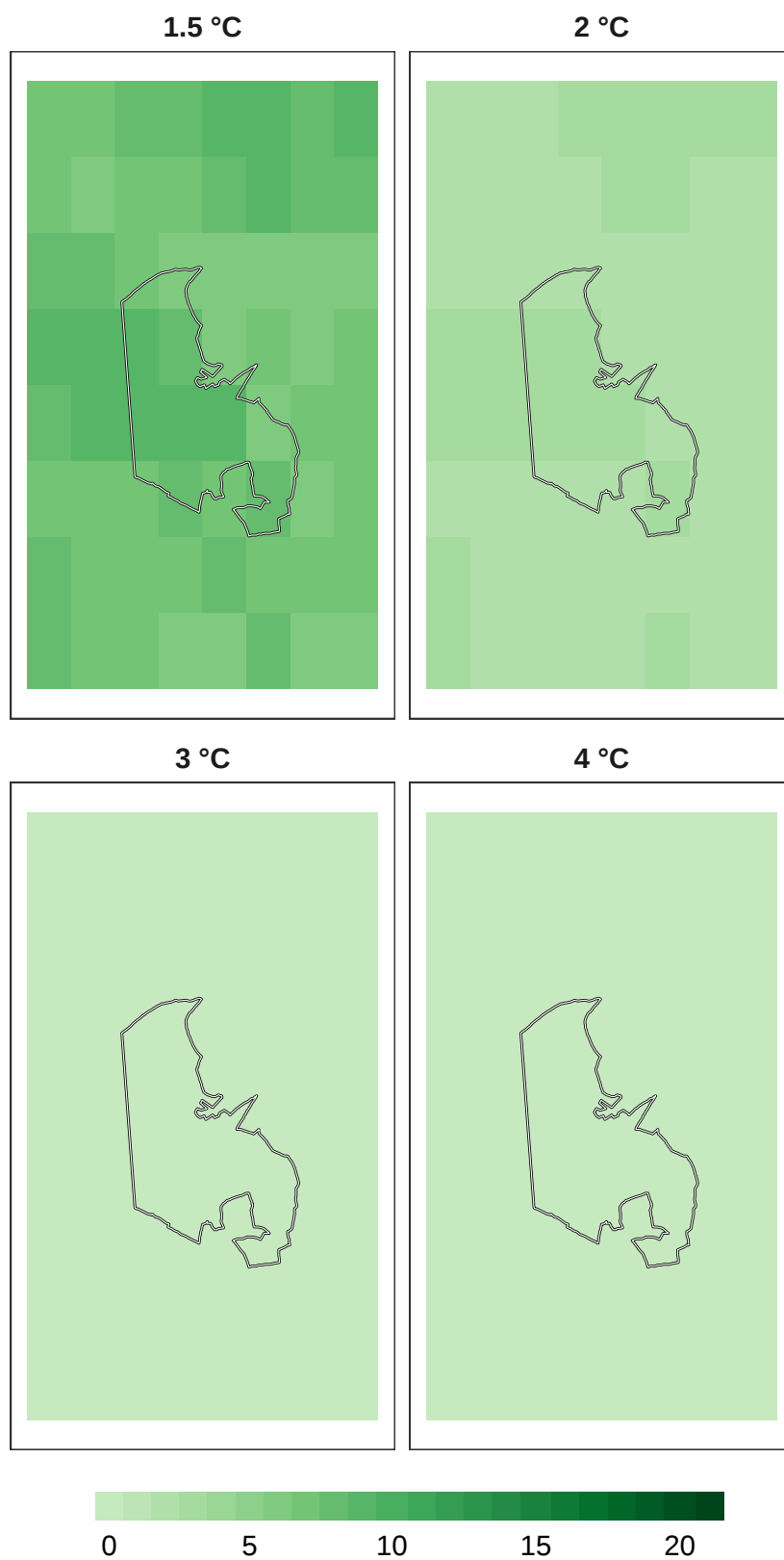
Figure 13: Number of models in agreement for pollinator refugia at 1 km resolution.
