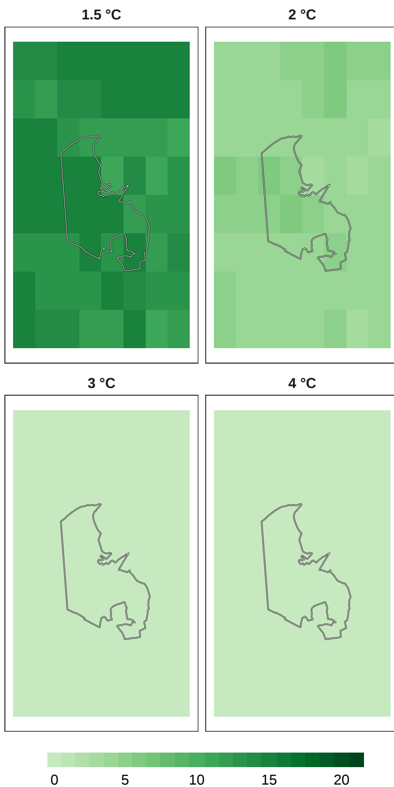
Figure 9: Number of models in agreement for plant refugia at 1 km resolution.
