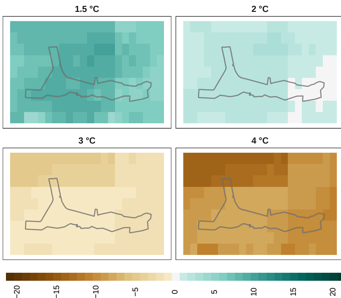
Figure 19: Adaptation effort for insects at 1 km resolution.
