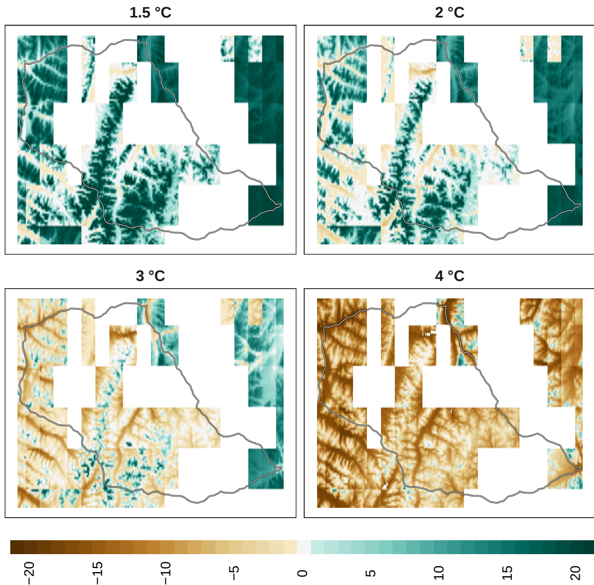
Figure 8: Adaptation effort for plants at 1 km resolution.
