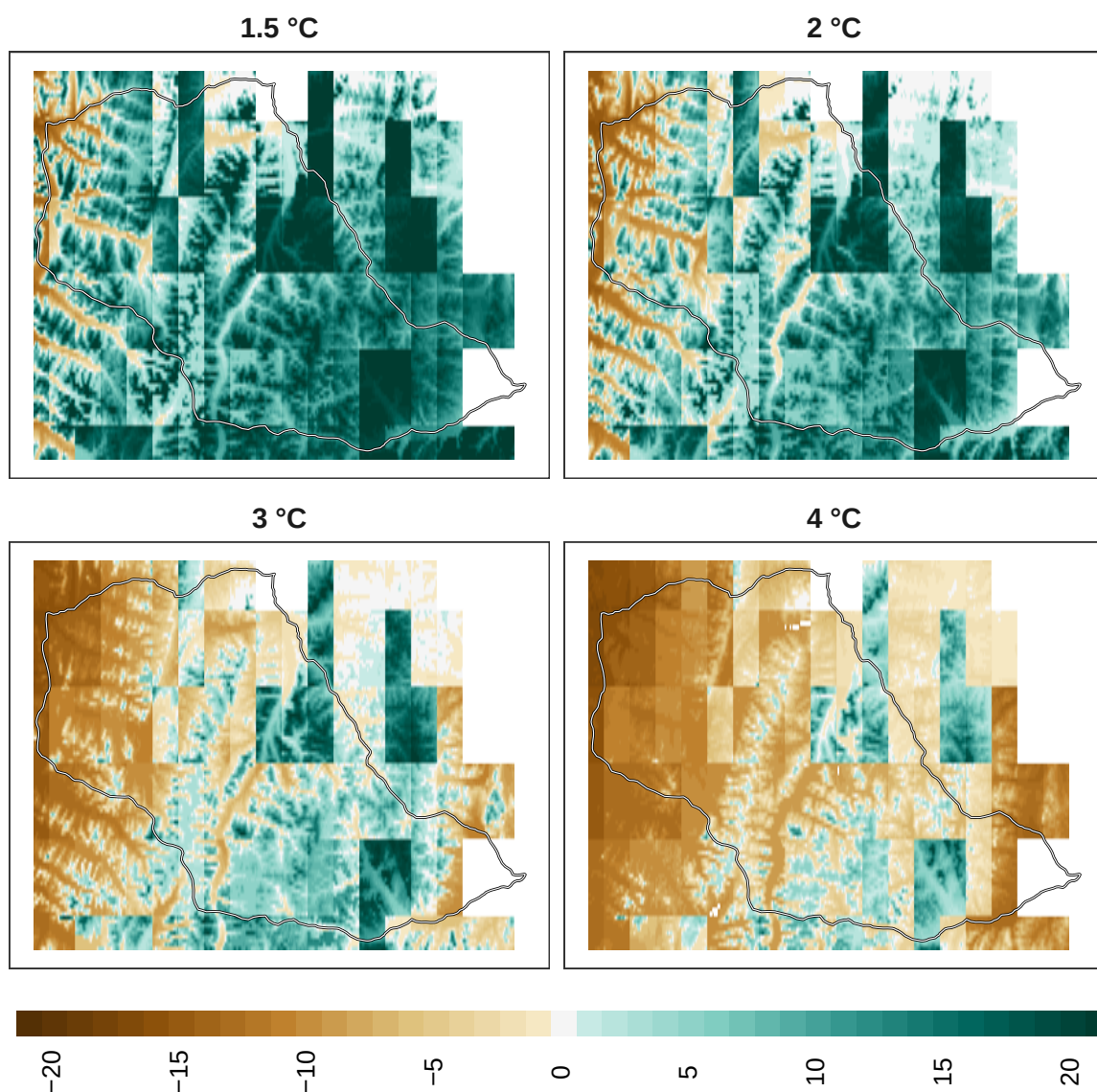
Figure 9: Adaptation effort for mammals at 1 km resolution.
