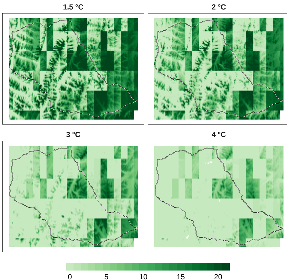
Figure 4: Number of models in agreement for overall biodiversity refugia at 1 km resolution.
