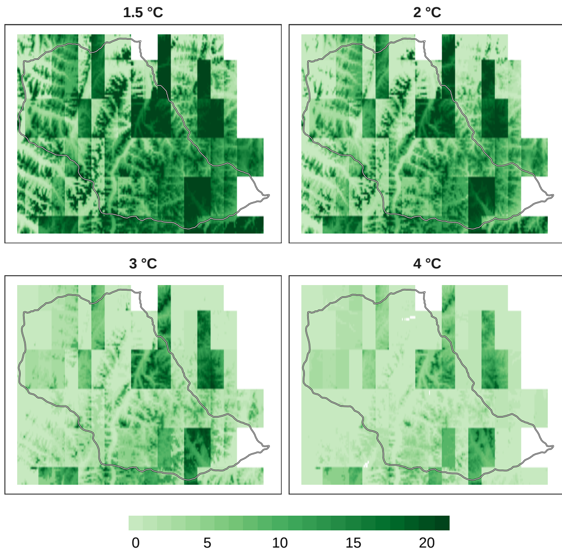
Figure 6: Number of models in agreement for mammal refugia at 1 km resolution.
