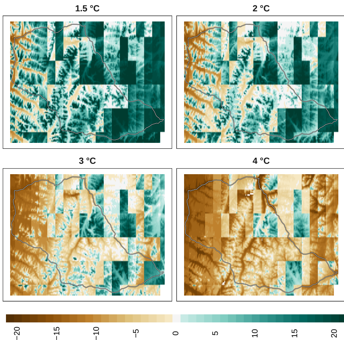
Figure 7: Adaptation effort for overall biodiversity at 1 km resolution.
