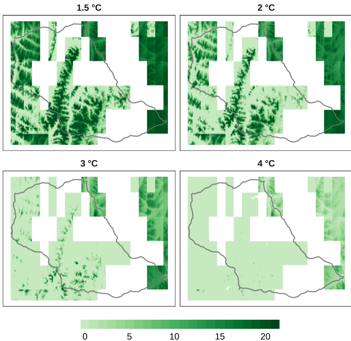
Figure 5: Number of models in agreement for plant refugia at 1 km resolution.
