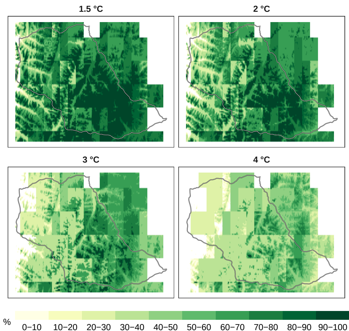
Figure 3: Percent mammals remaining at 1 km resolution.
