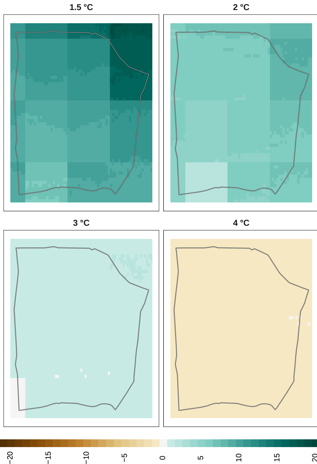
Figure 16: Adaptation effort for mammals at 1 km resolution.
