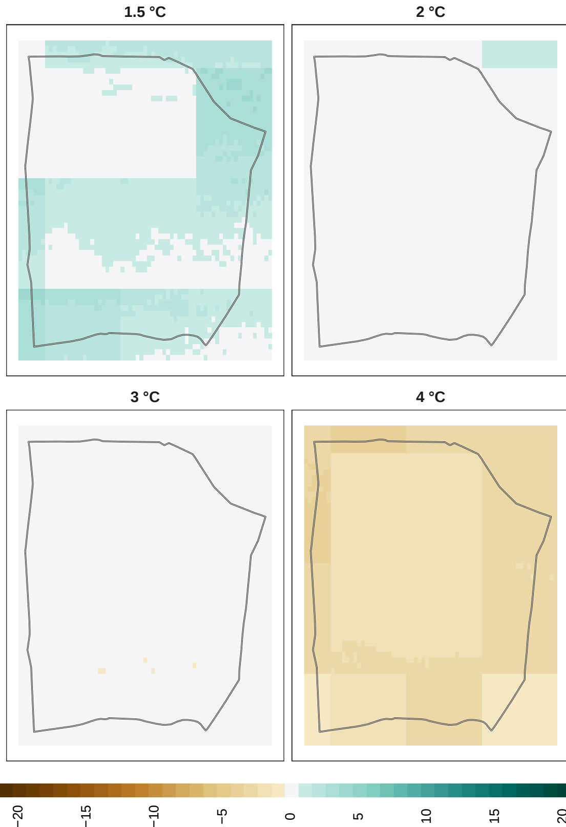
Figure 13: Adaptation effort for overall biodiversity at 1 km resolution.
