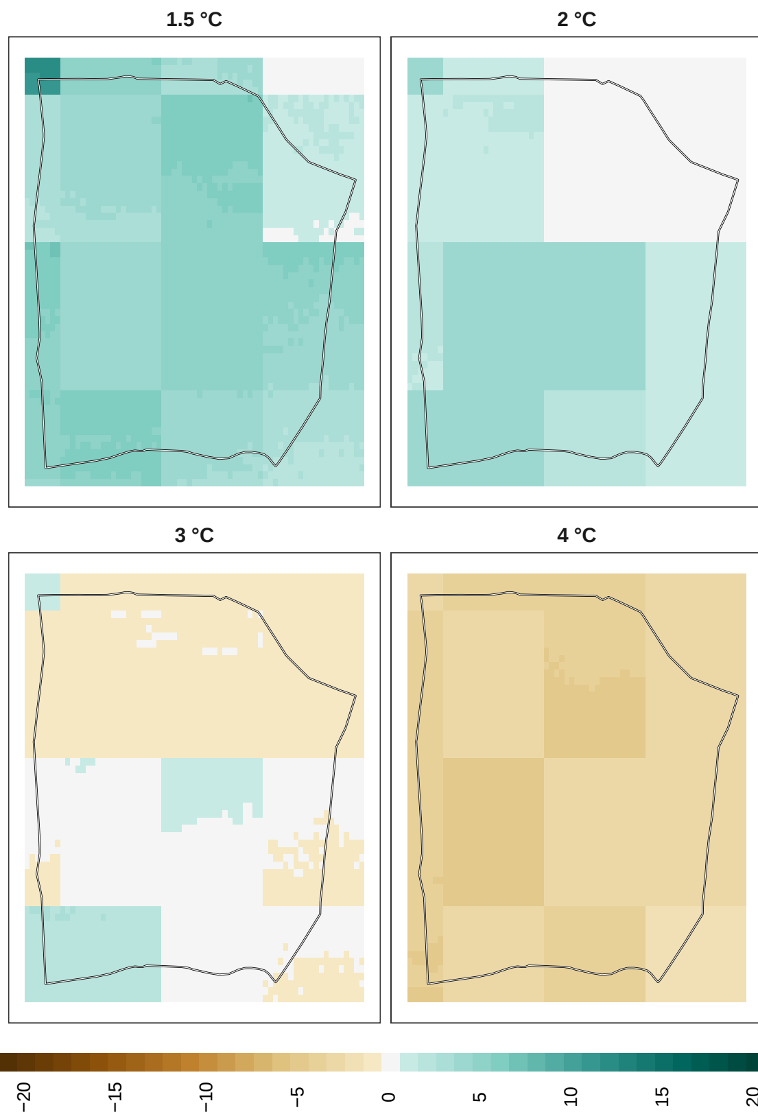
Figure 15: Adaptation effort for birds at 1 km resolution.
