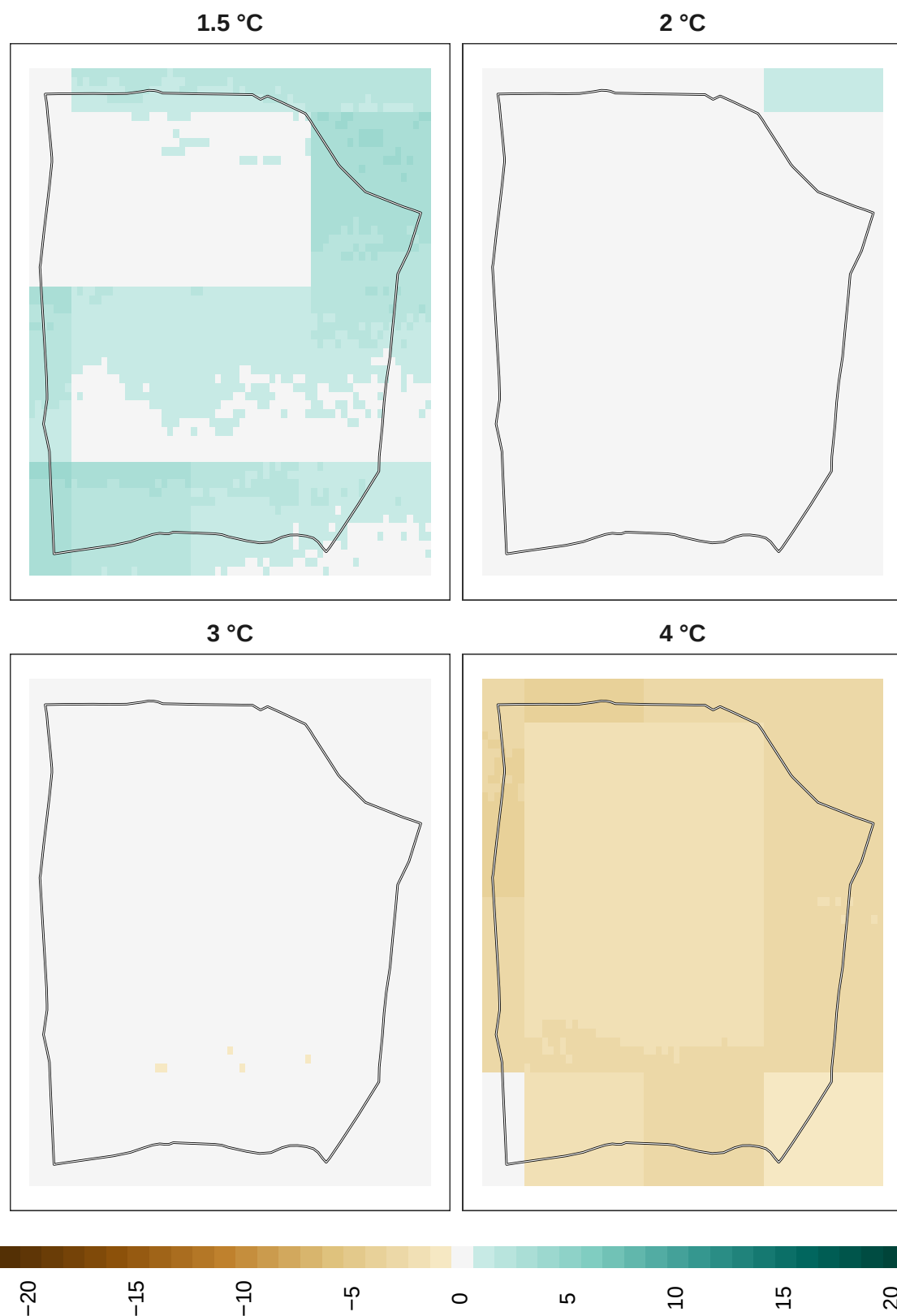
Figure 14: Adaptation effort for plants at 1 km resolution.
