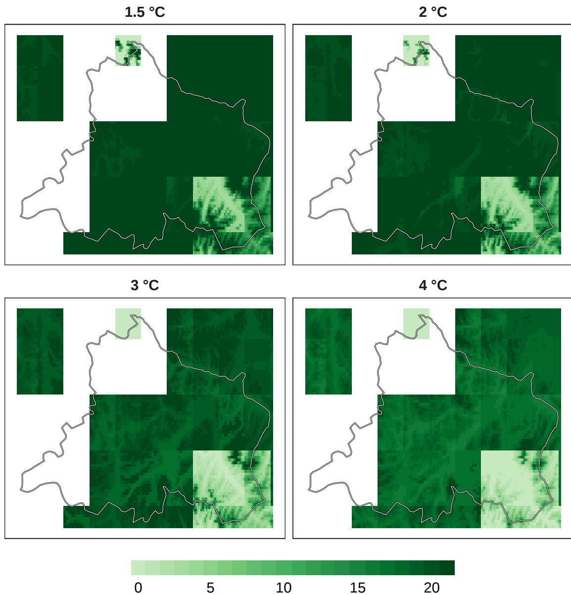
Figure 6: Number of models in agreement for mammal refugia at 1 km resolution.
