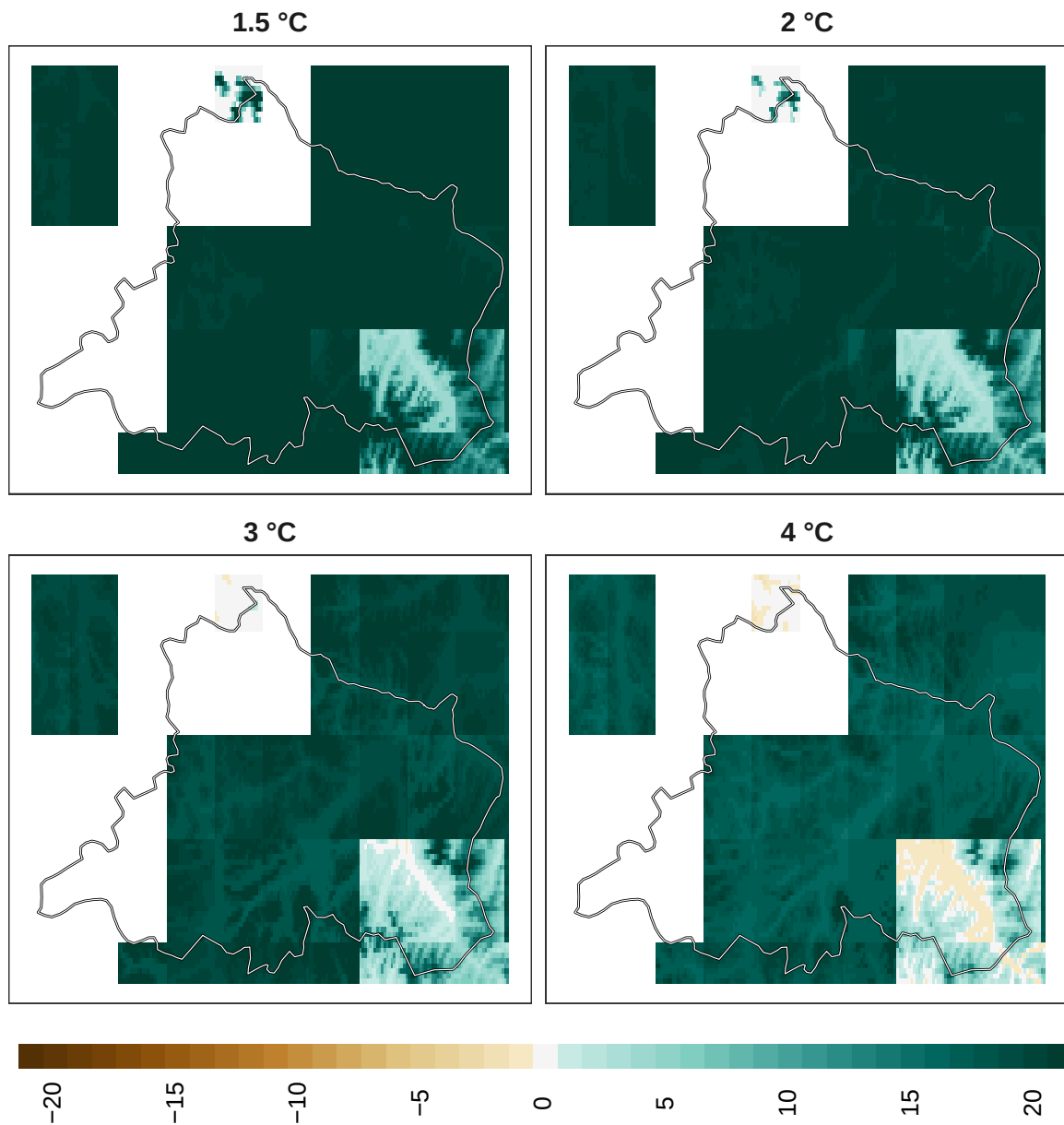
Figure 9: Adaptation effort for mammals at 1 km resolution.
