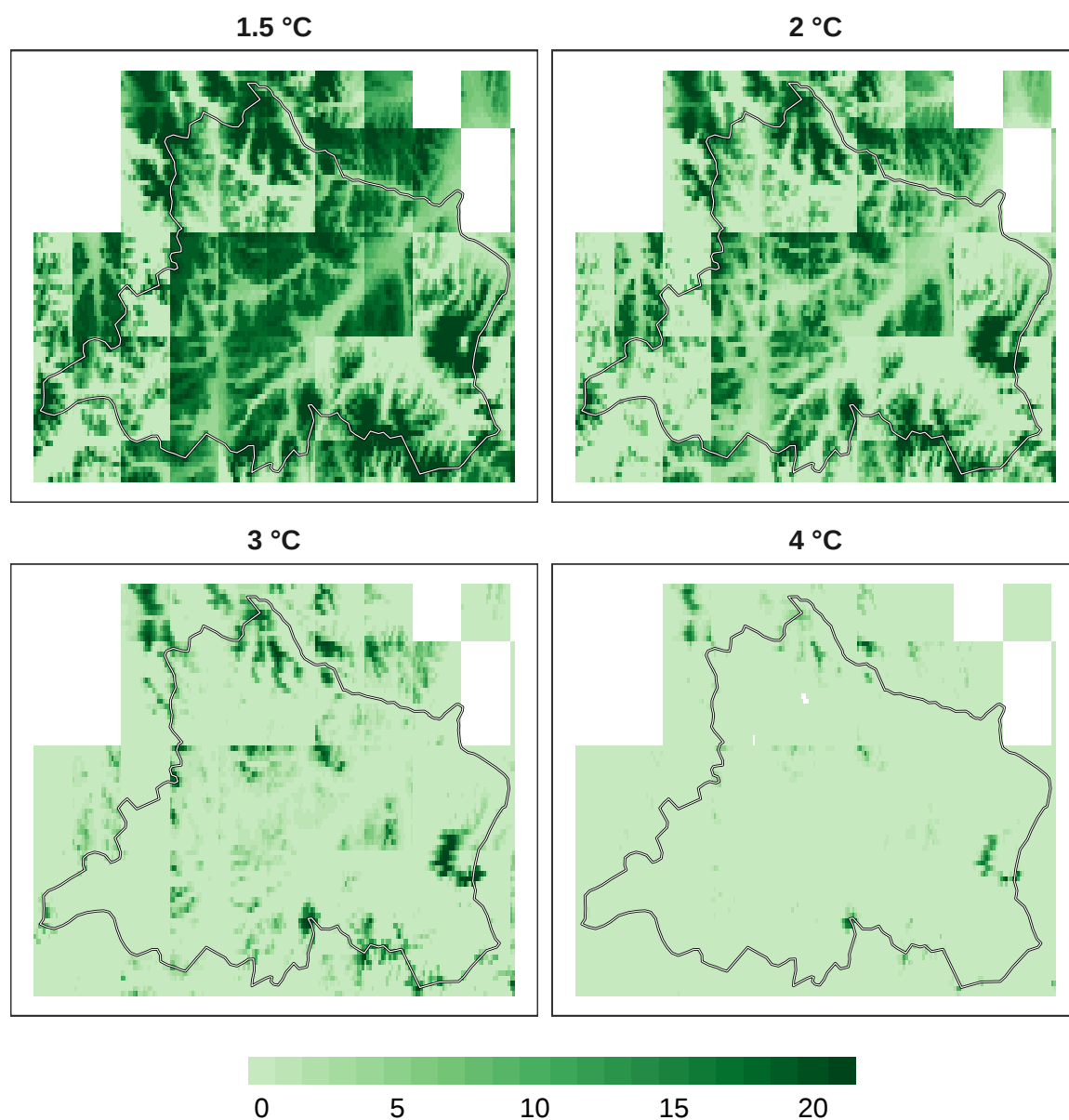
Figure 5: Number of models in agreement for plant refugia at 1 km resolution.
