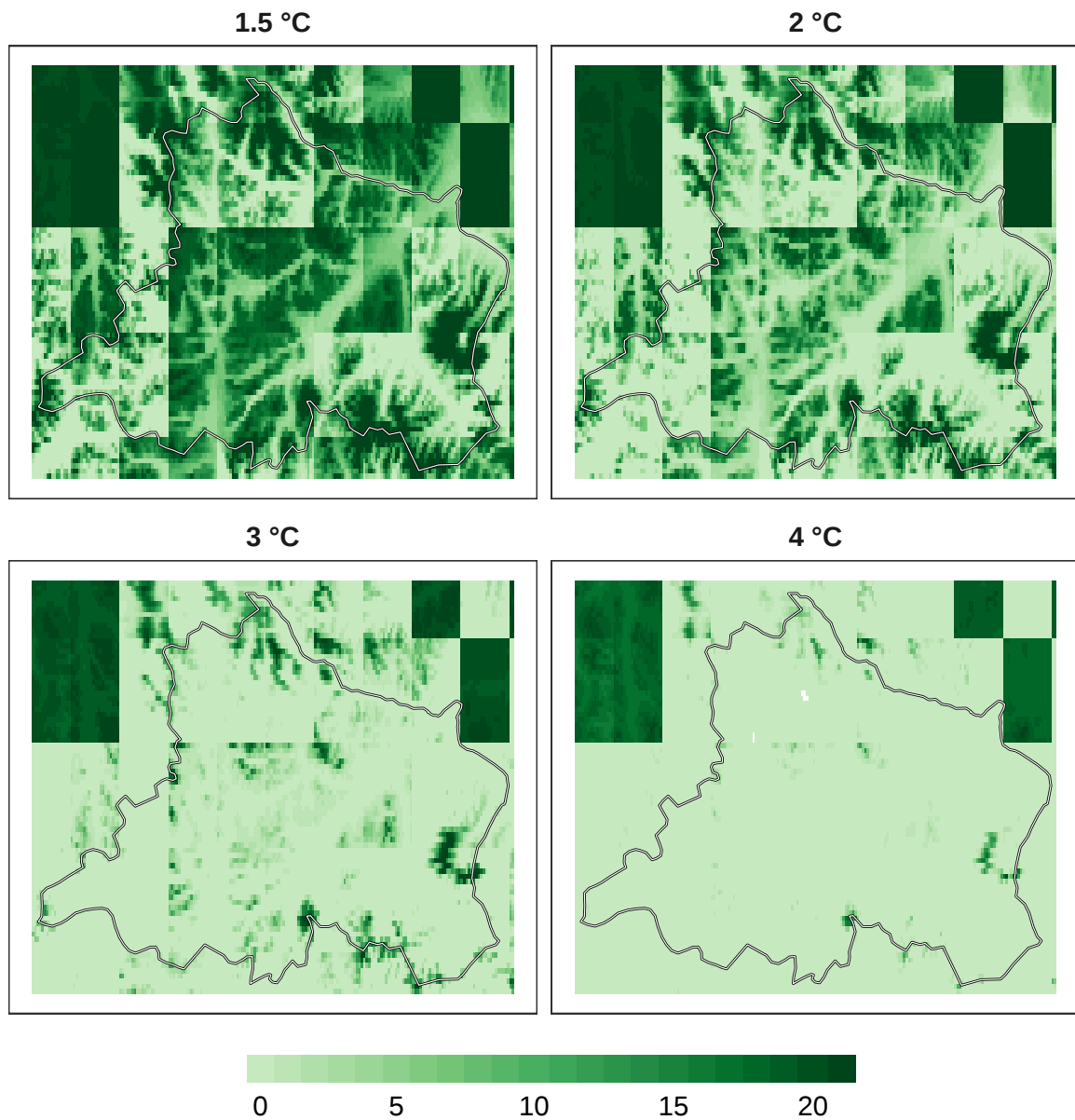
Figure 4: Number of models in agreement for overall biodiversity refugia at 1 km resolution.
