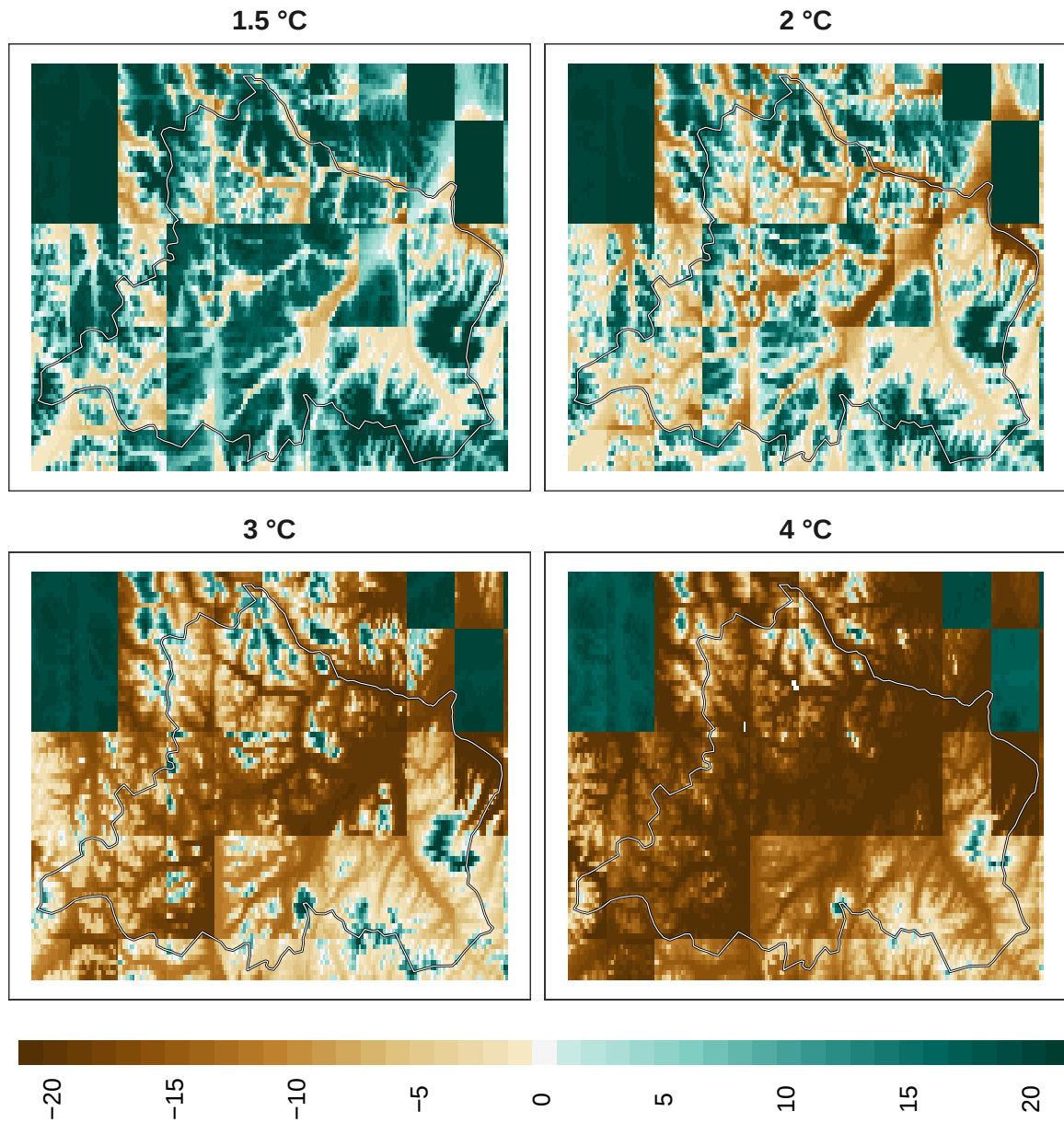
Figure 7: Adaptation effort for overall biodiversity at 1 km resolution.
