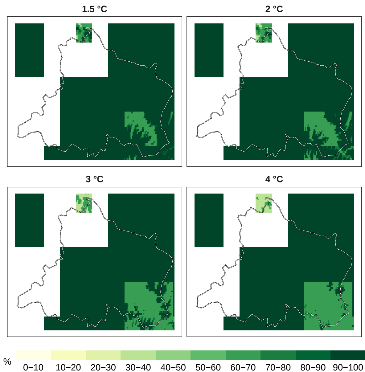
Figure 3: Percent mammals remaining at 1 km resolution.
