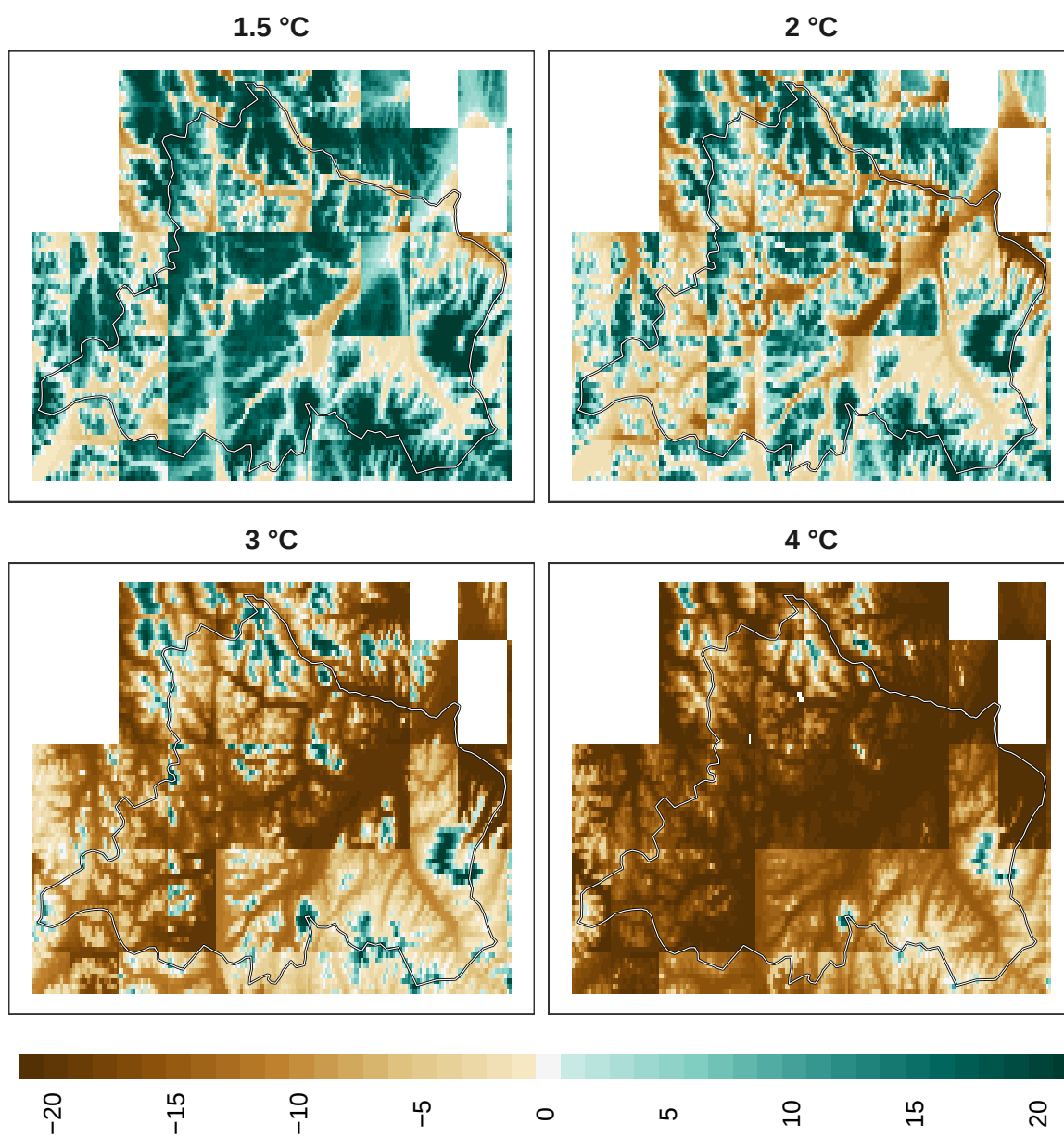
Figure 8: Adaptation effort for plants at 1 km resolution.
