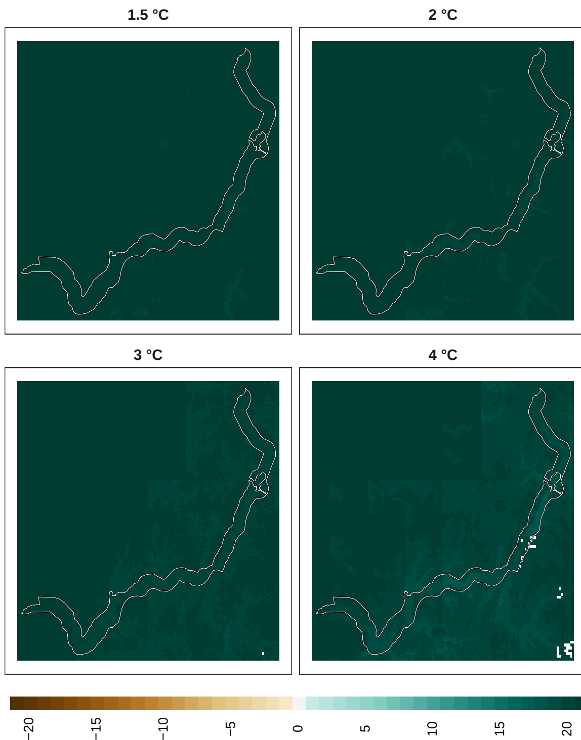
Figure 12: Adaptation effort for plants at 1 km resolution.
