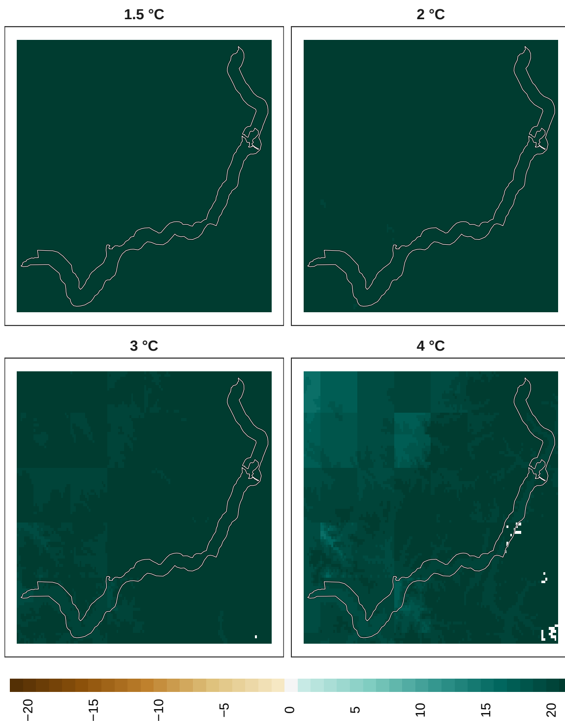
Figure 15: Adaptation effort for insects at 1 km resolution.
