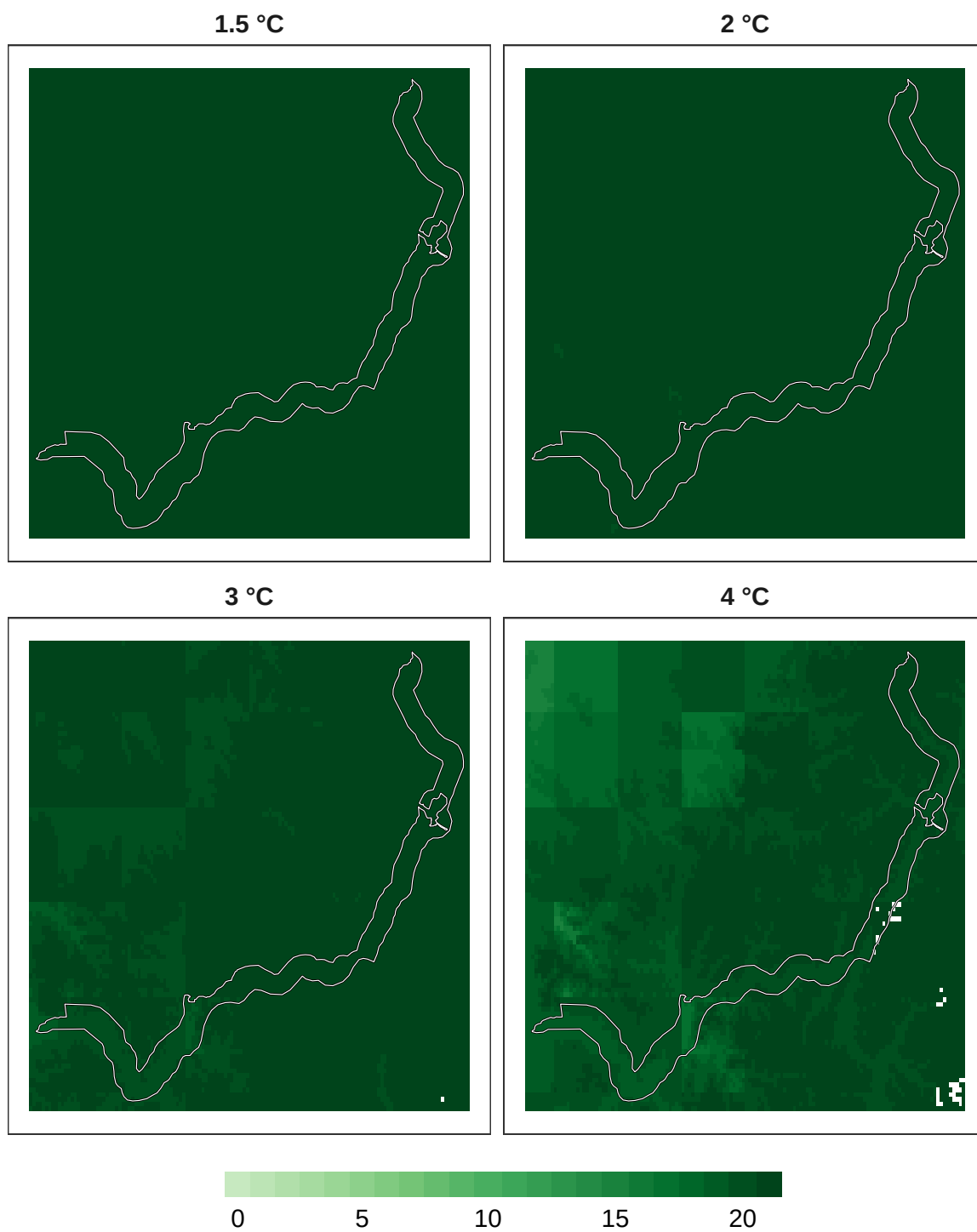
Figure 10: Number of models in agreement for insect refugia at 1 km resolution.
