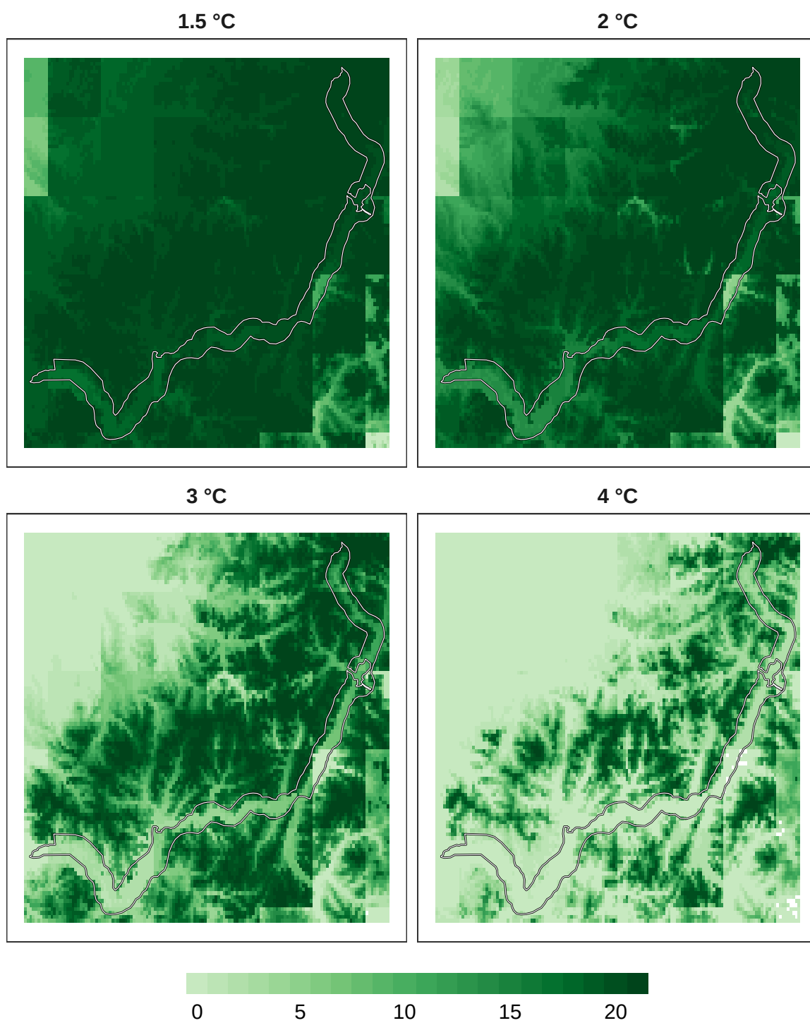
Figure 9: Number of models in agreement for mammal refugia at 1 km resolution.
