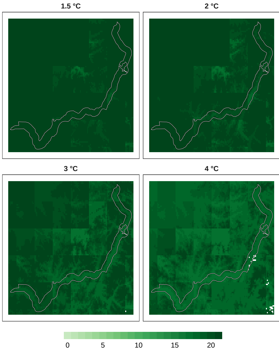
Figure 8: Number of models in agreement for bird refugia.
