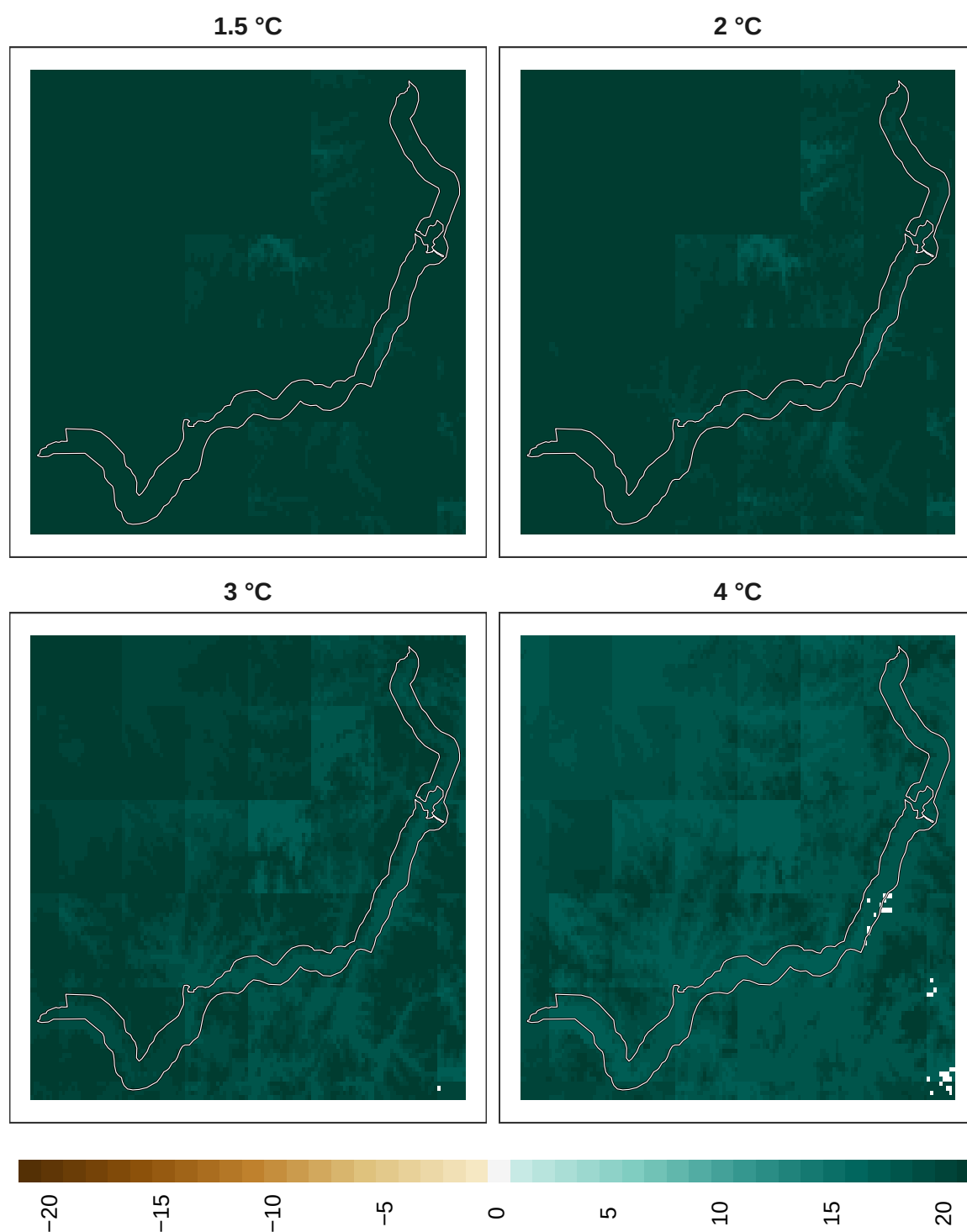
Figure 13: Adaptation effort for birds at 1 km resolution.
