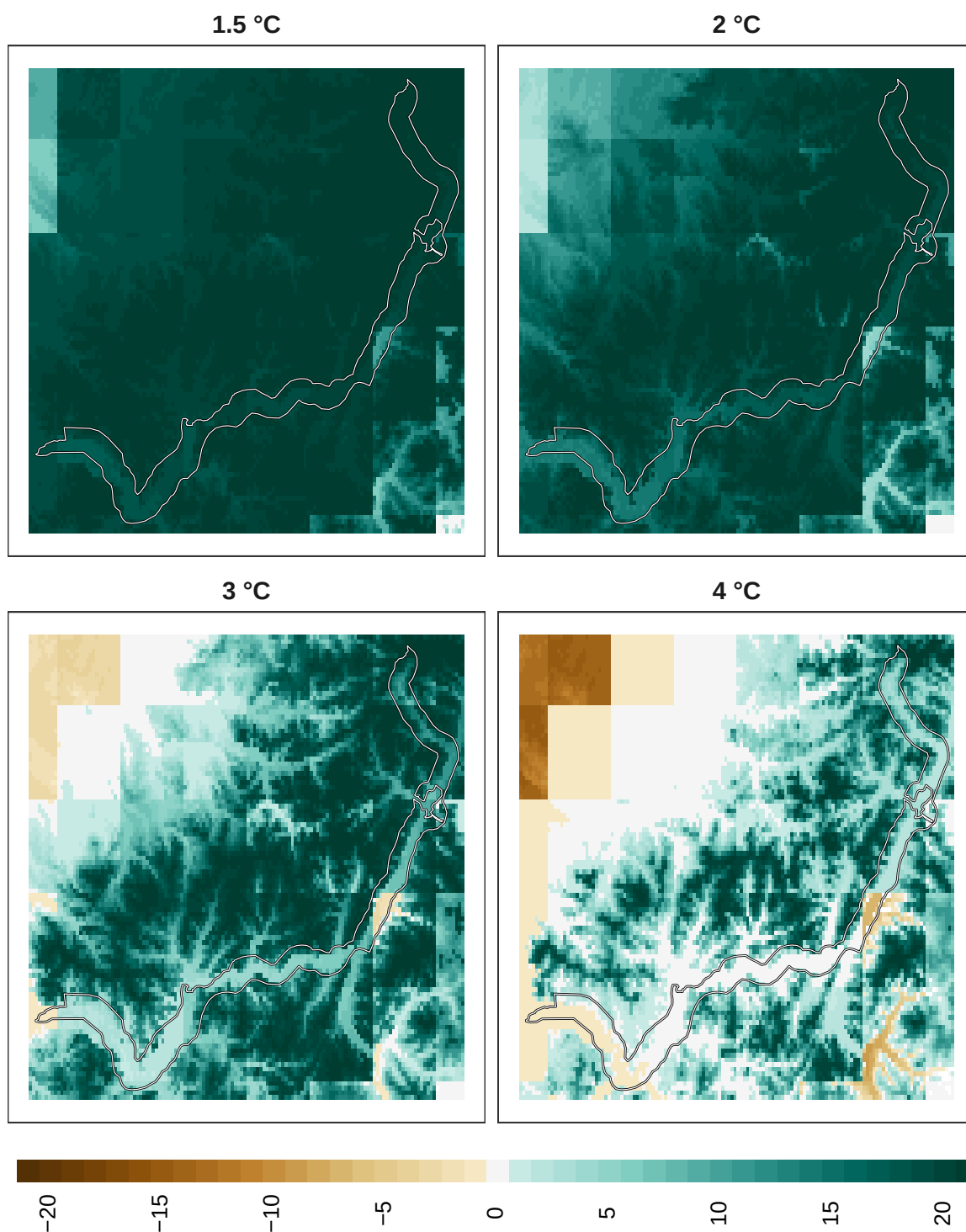
Figure 14: Adaptation effort for mammals at 1 km resolution.
