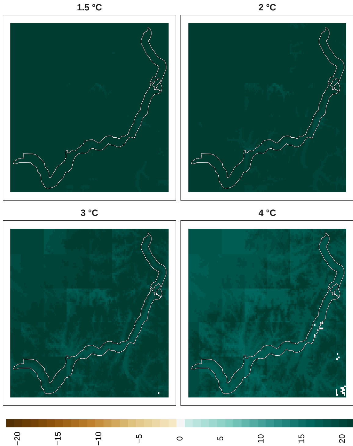
Figure 11: Adaptation effort for overall biodiversity at 1 km resolution.
