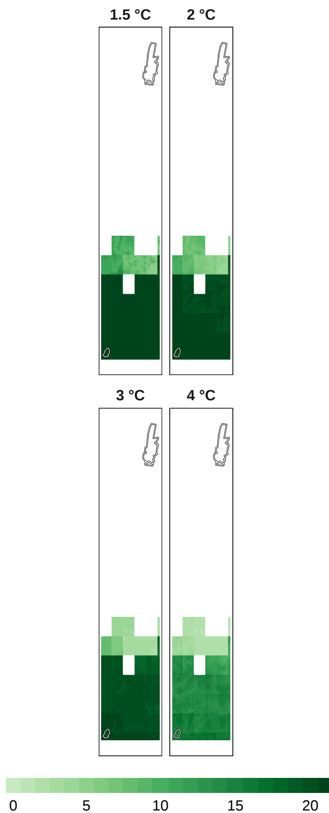
Figure 11: Number of models in agreement for reptile refugia at 1 km resolution.
