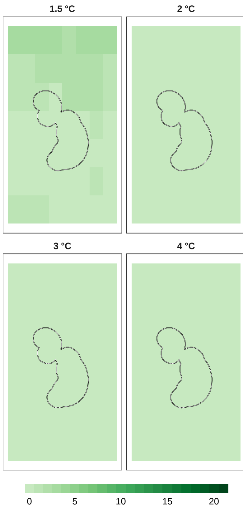
Figure 9: Number of models in agreement for insect refugia at 1 km resolution.
