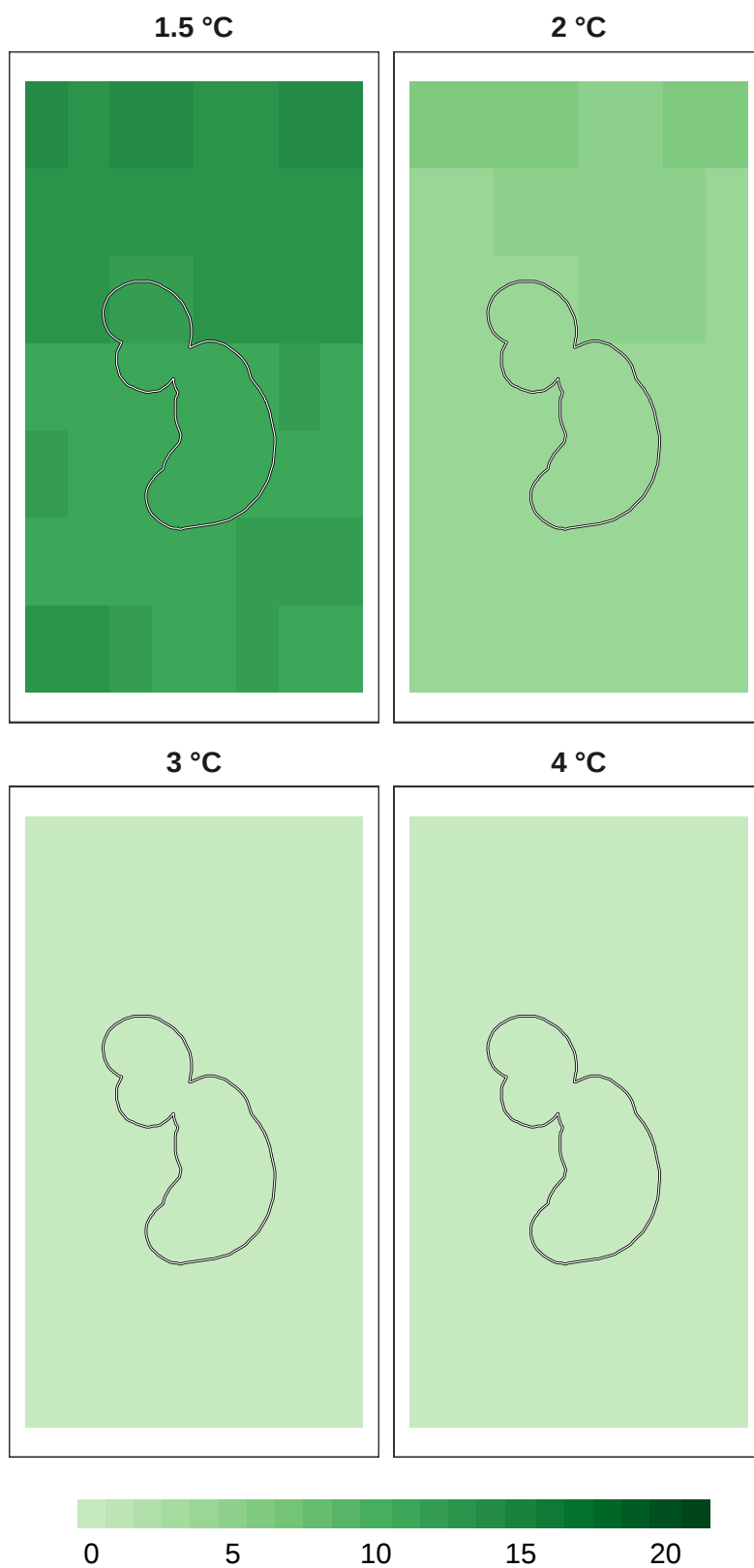
Figure 10: Number of models in agreement for pollinator refugia at 1 km resolution.
