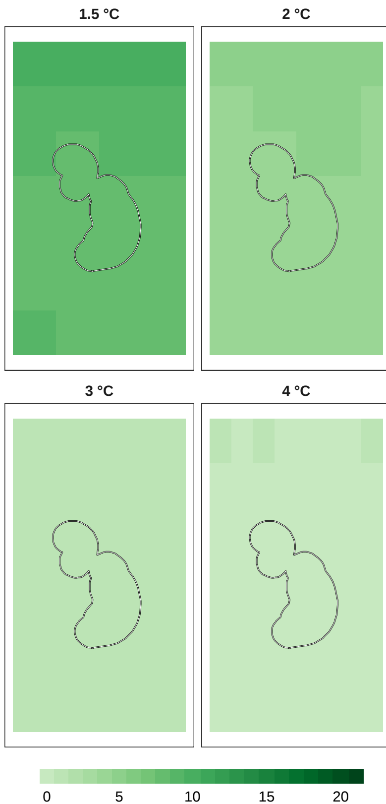
Figure 7: Number of models in agreement for plant refugia at 1 km resolution.
