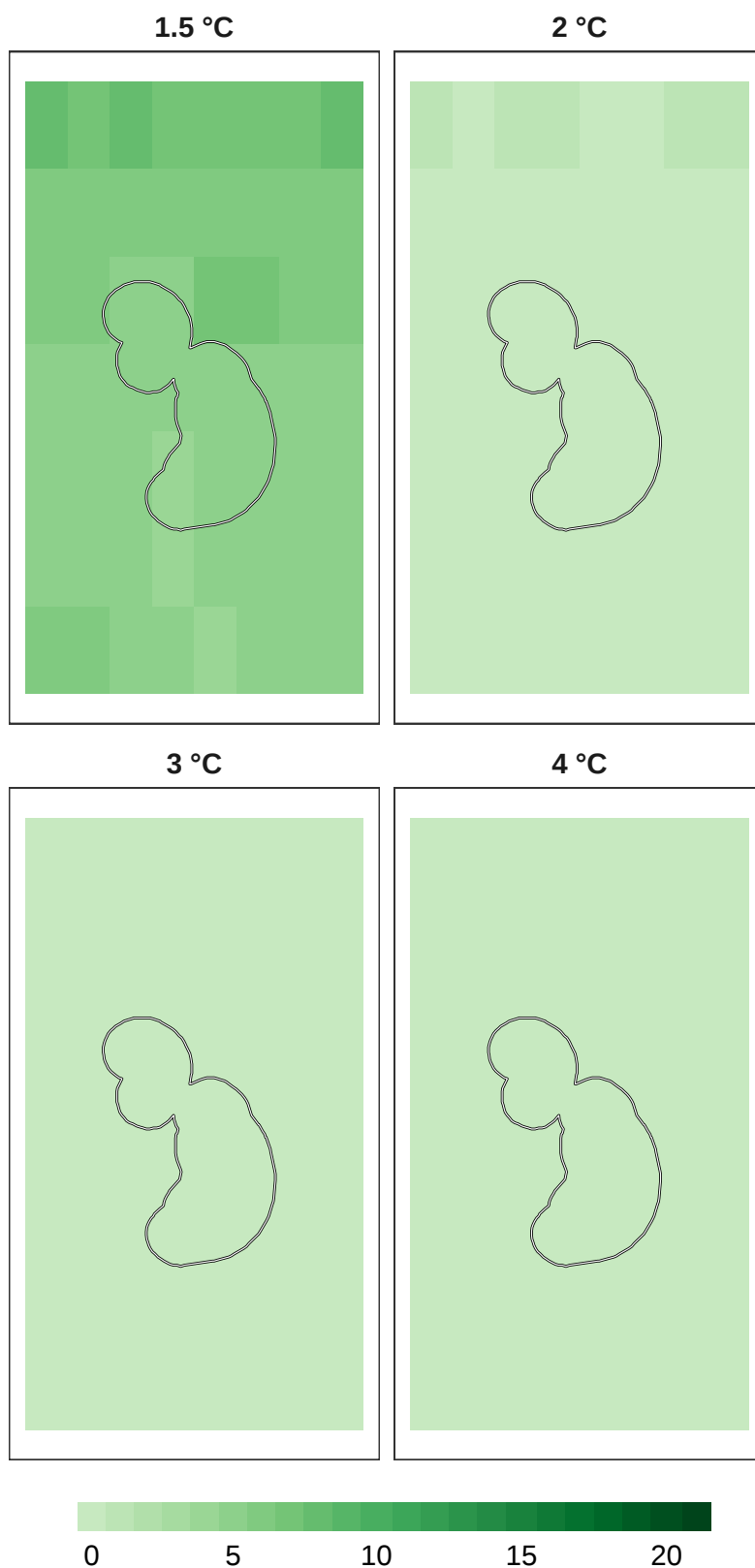
Figure 6: Number of models in agreement for overall biodiversity refugia at 1 km resolution.
