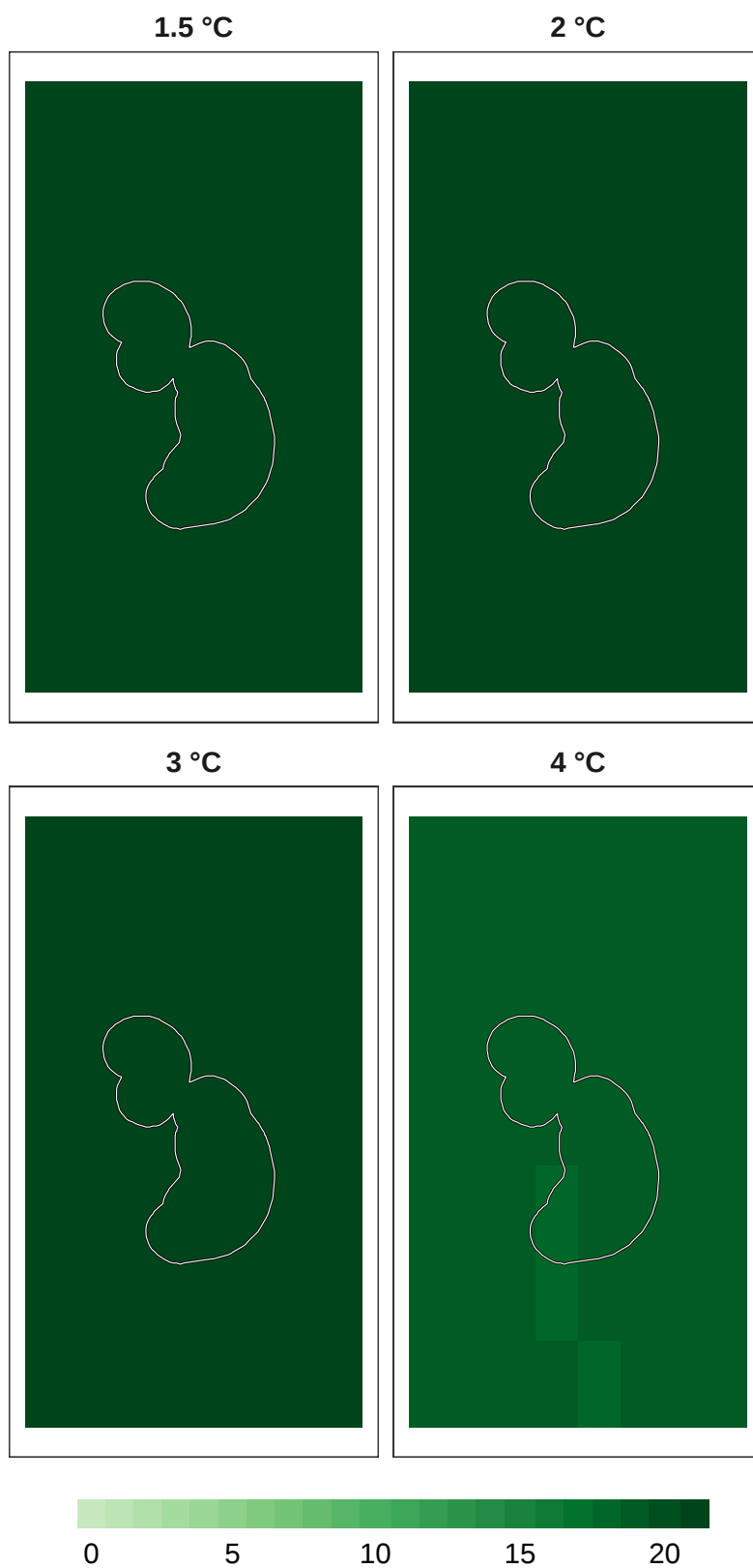
Figure 8: Number of models in agreement for bird refugia.
