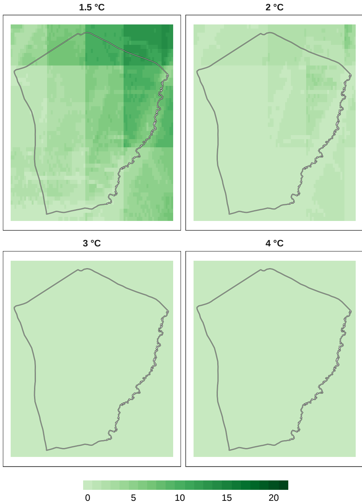
Figure 5: Number of models in agreement for plant refugia at 1 km resolution.
