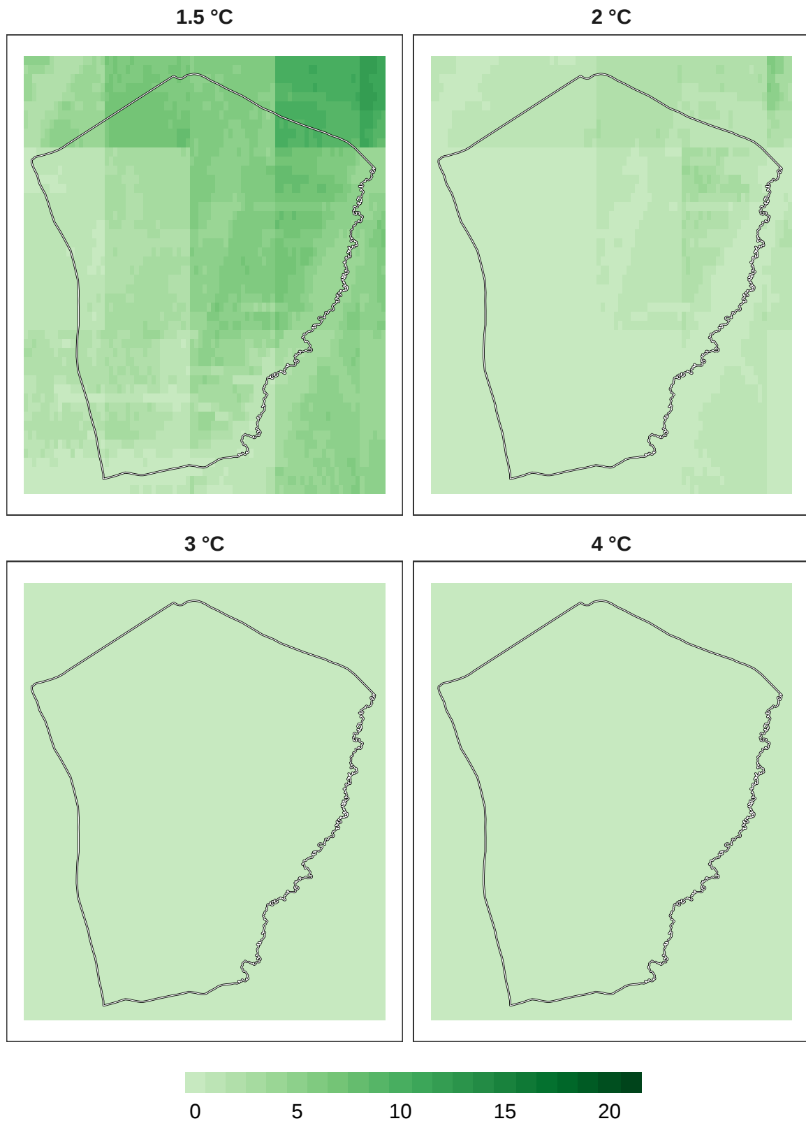
Figure 4: Number of models in agreement for overall biodiversity refugia at 1 km resolution.
