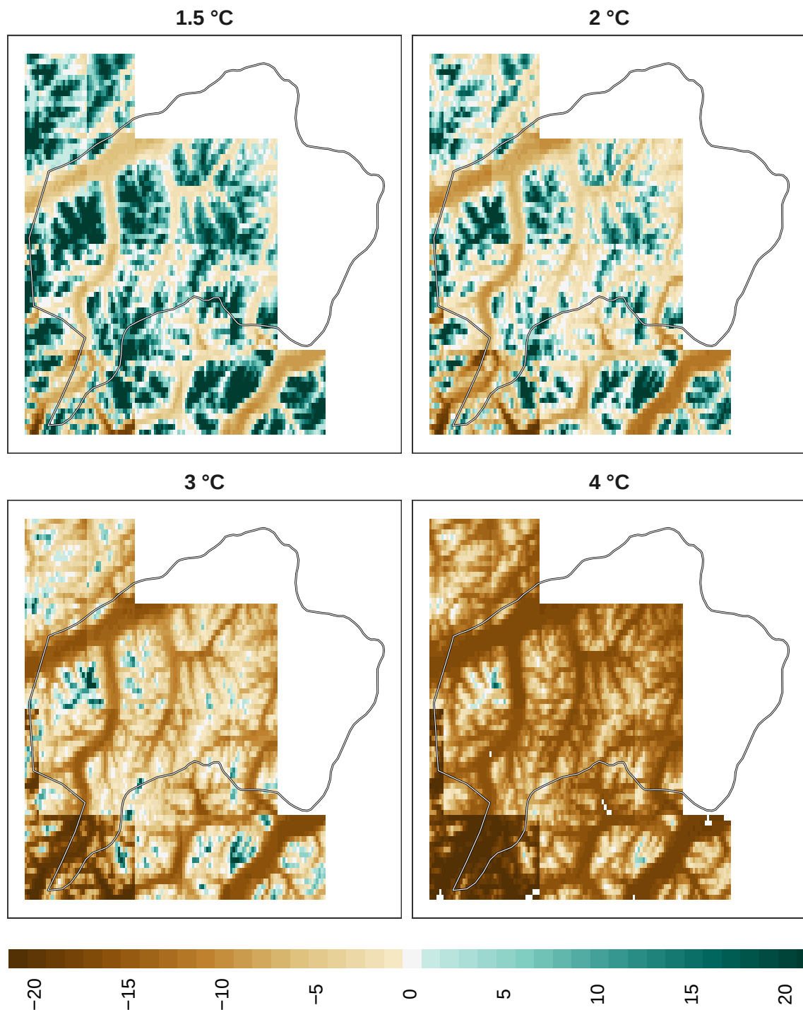
Figure 8: Adaptation effort for plants at 1 km resolution.
