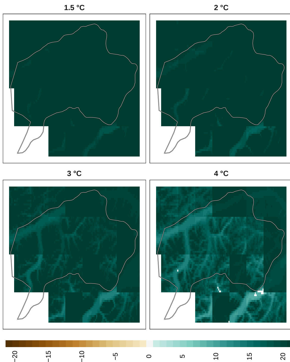
Figure 9: Adaptation effort for mammals at 1 km resolution.
