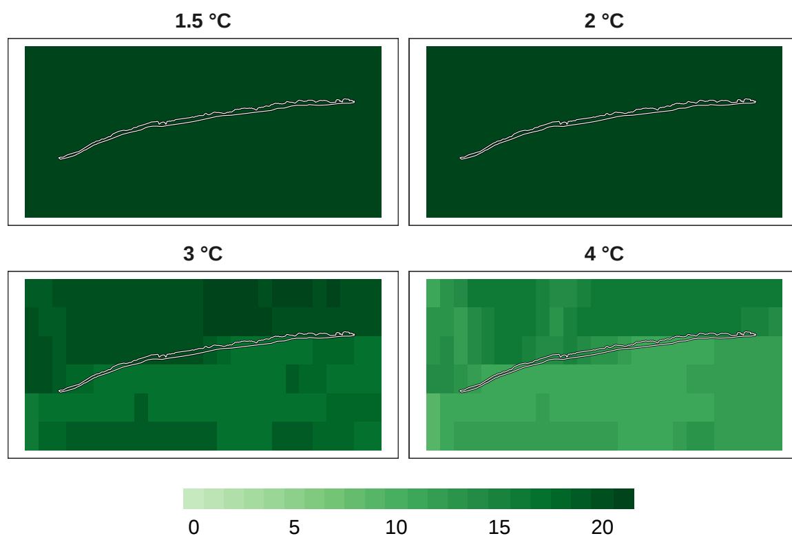
Figure 6: Number of models in agreement for mammal refugia at 1 km resolution.
