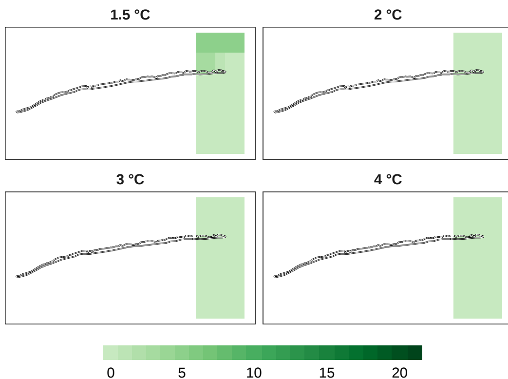
Figure 5: Number of models in agreement for plant refugia at 1 km resolution.
