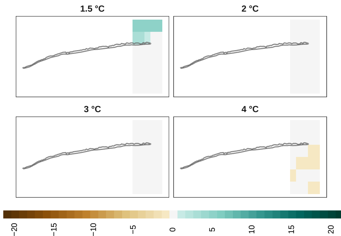
Figure 8: Adaptation effort for plants at 1 km resolution.
