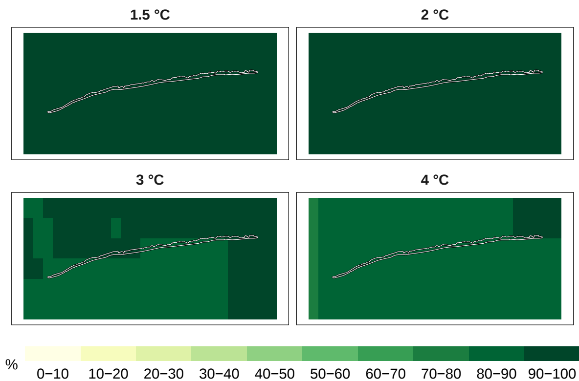
Figure 3: Percent mammals remaining at 1 km resolution.
