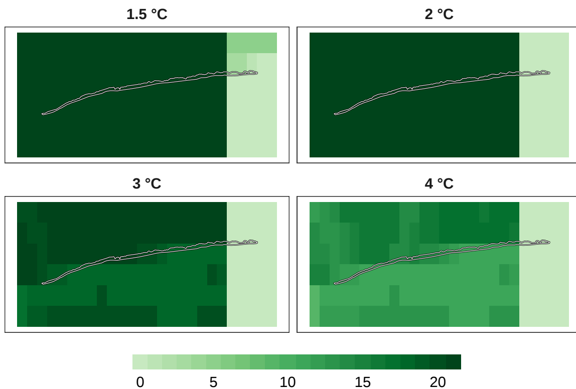
Figure 4: Number of models in agreement for overall biodiversity refugia at 1 km resolution.
