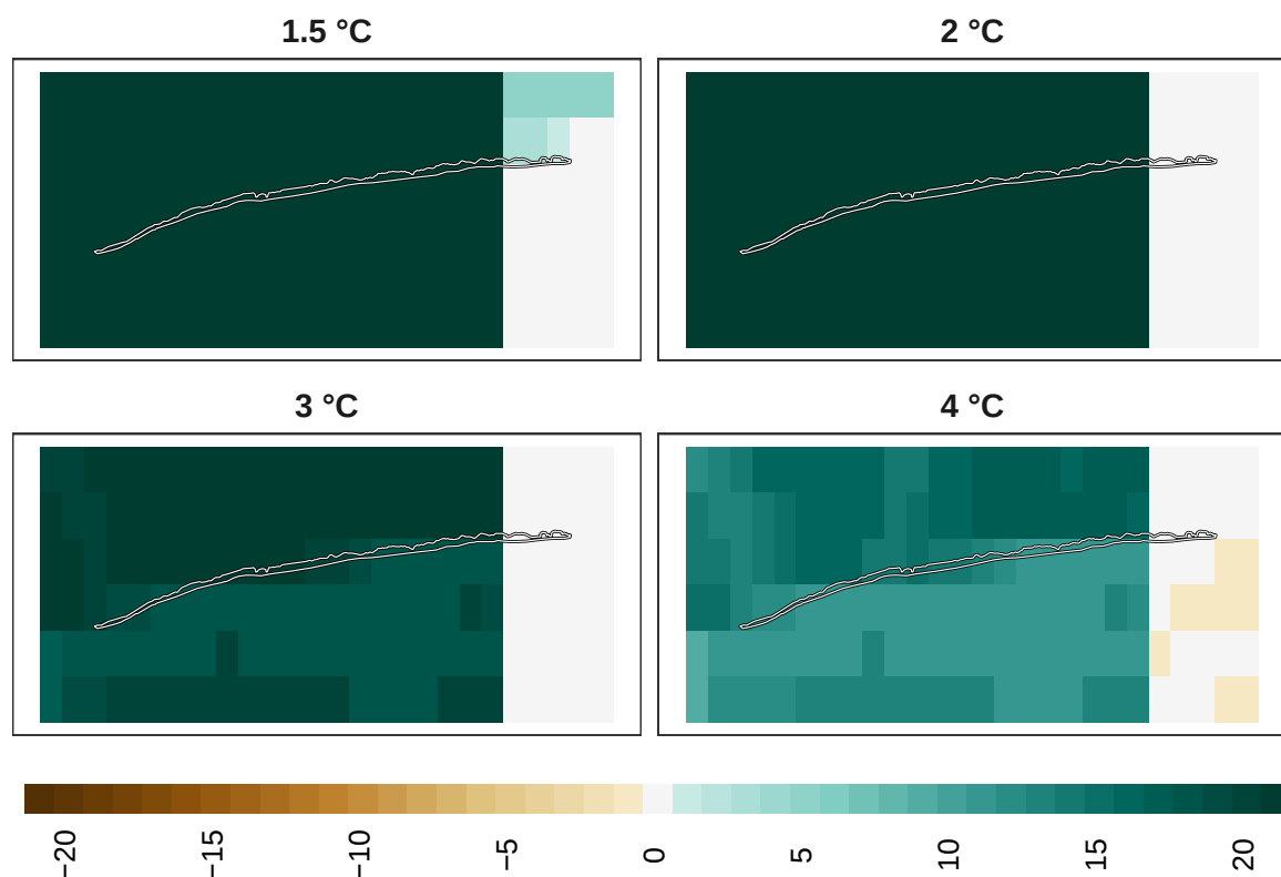
Figure 7: Adaptation effort for overall biodiversity at 1 km resolution.
