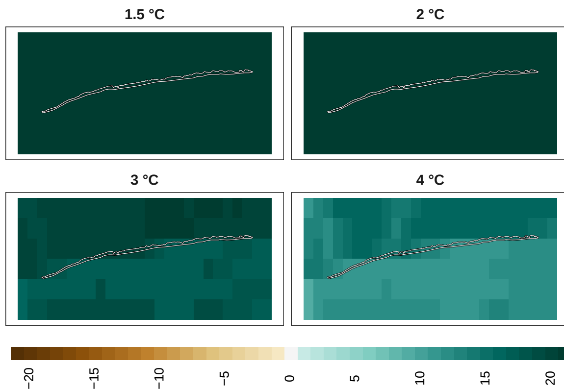
Figure 9: Adaptation effort for mammals at 1 km resolution.
