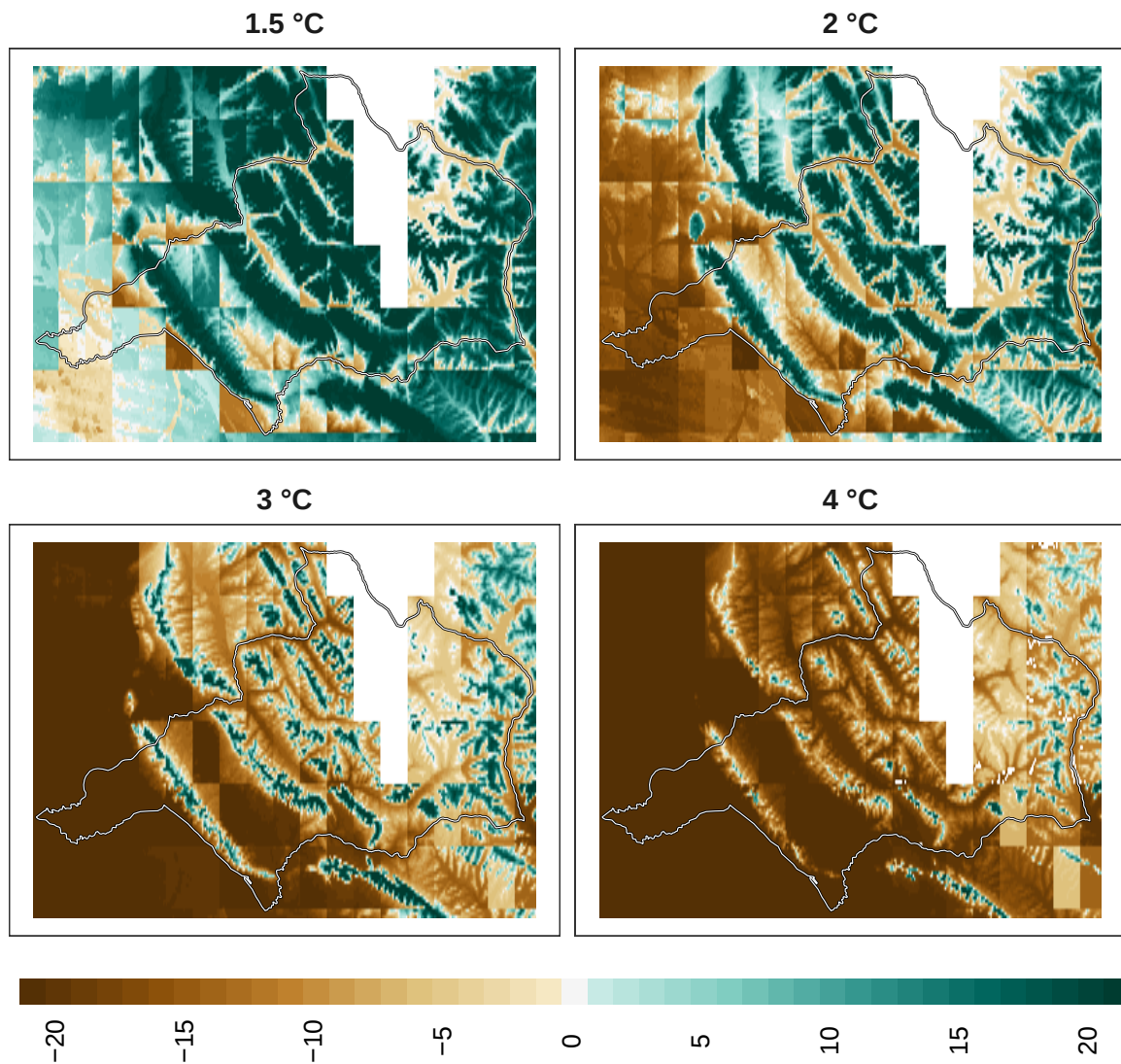
Figure 8: Adaptation effort for plants at 1 km resolution.
