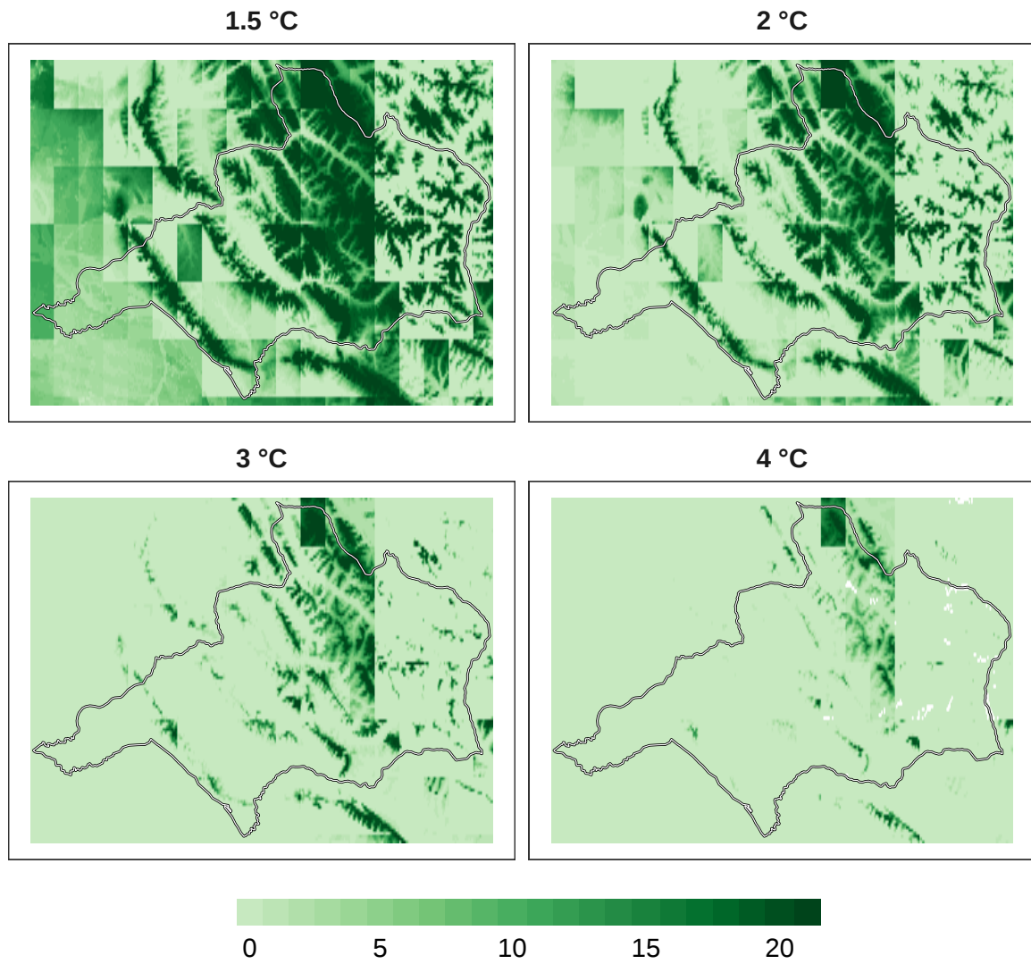
Figure 4: Number of models in agreement for overall biodiversity refugia at 1 km resolution.
