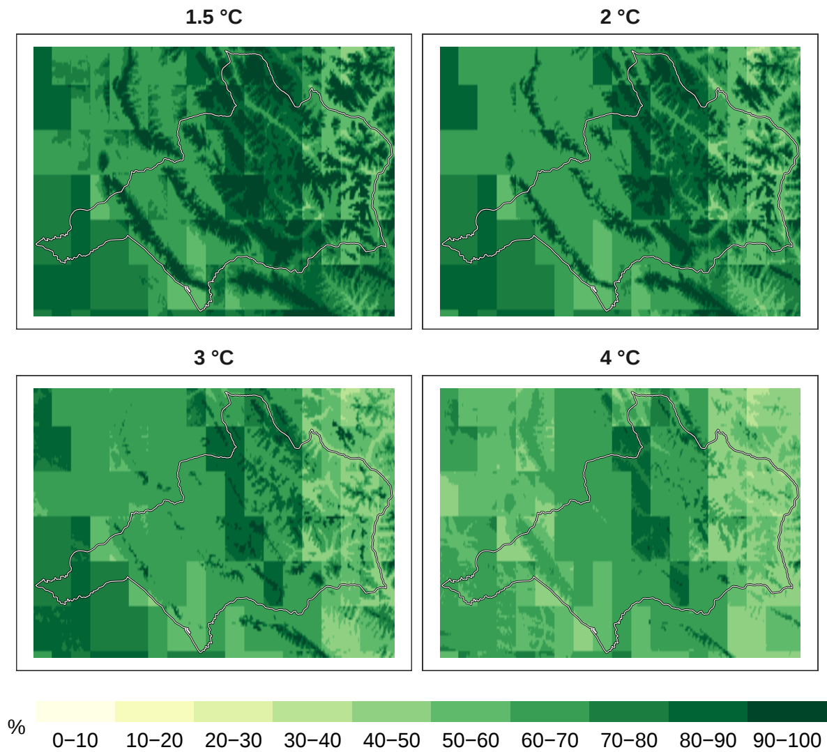
Figure 3: Percent mammals remaining at 1 km resolution.
