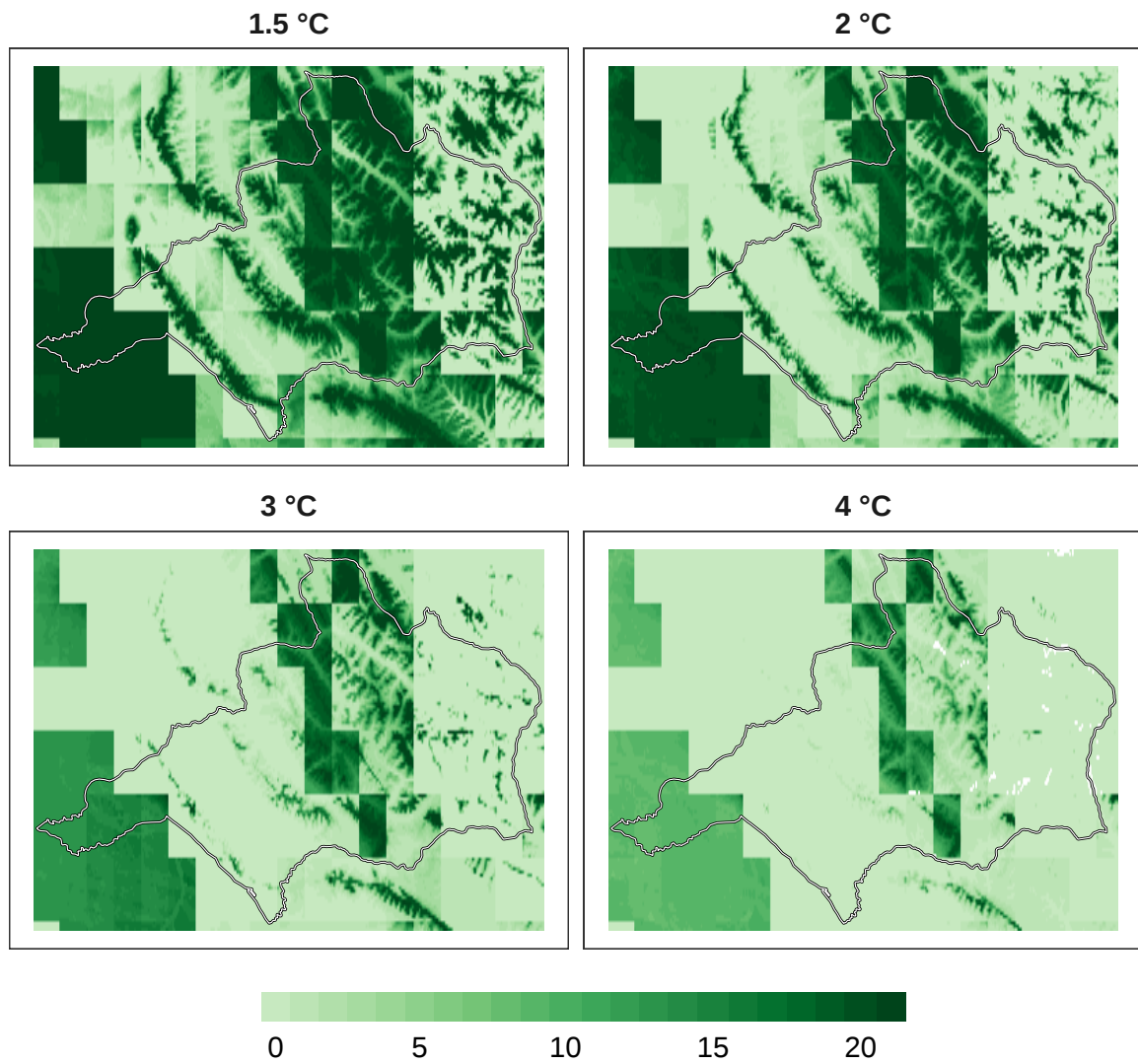
Figure 6: Number of models in agreement for mammal refugia at 1 km resolution.
