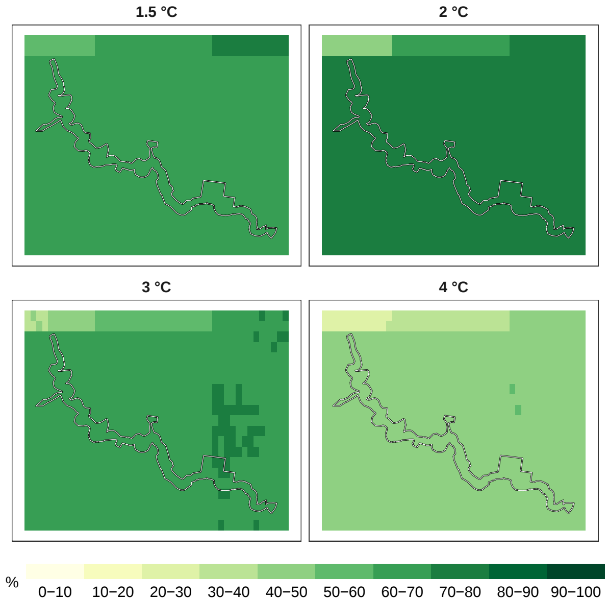
Figure 7: Percent timber species remaining at 1 km resolution.
