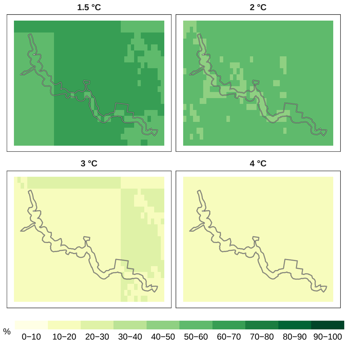
Figure 6: Percent pollinators remaining at 1 km resolution.
