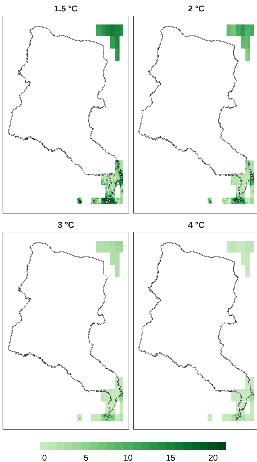
Figure 7: Number of models in agreement for mammal refugia at 1 km resolution.
