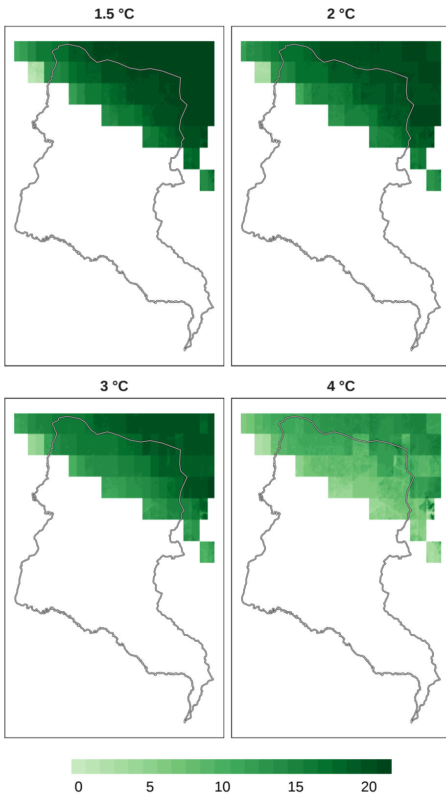
Figure 8: Number of models in agreement for insect refugia at 1 km resolution.
