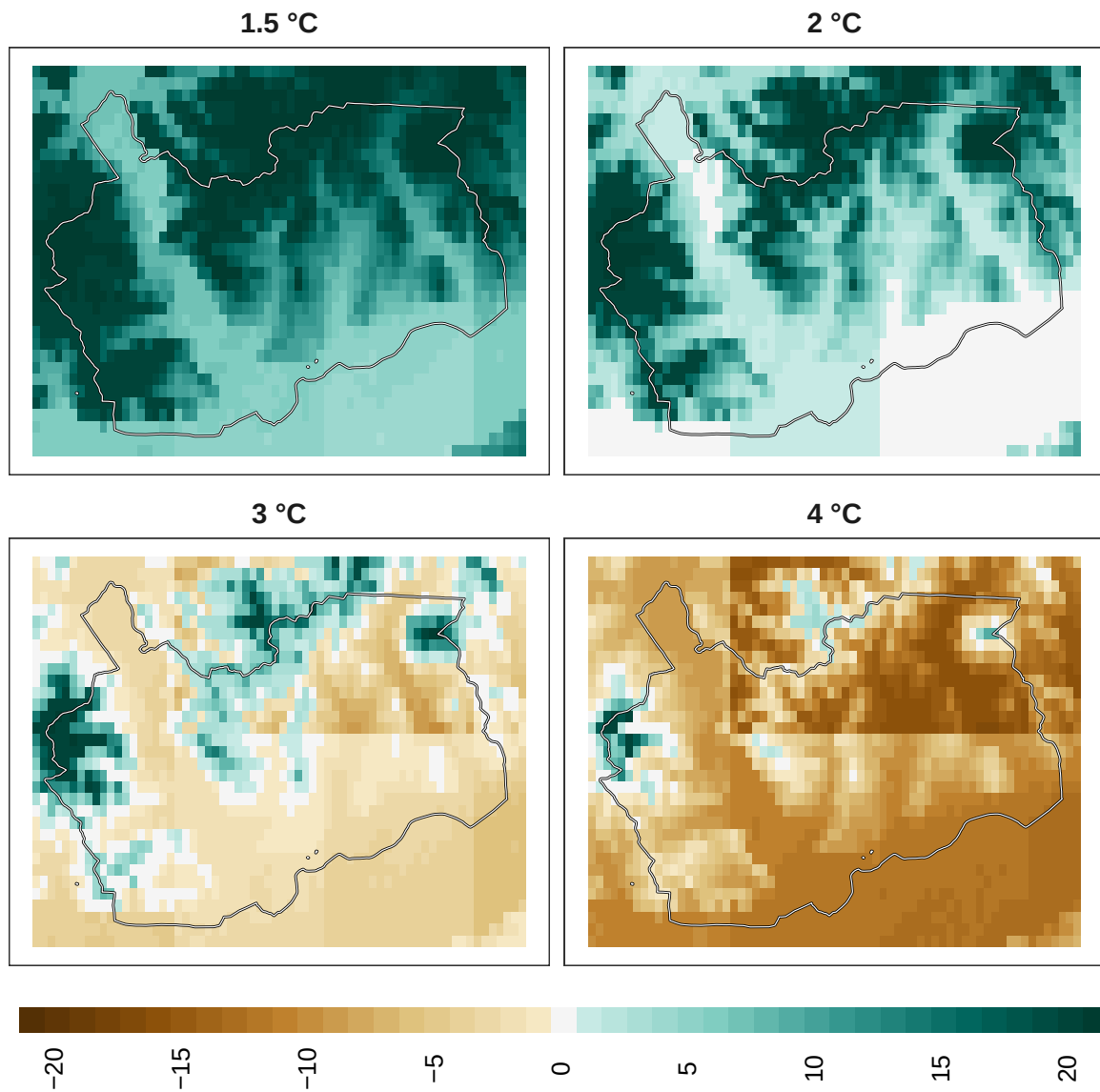
Figure 12: Adaptation effort for mammals at 1 km resolution.
