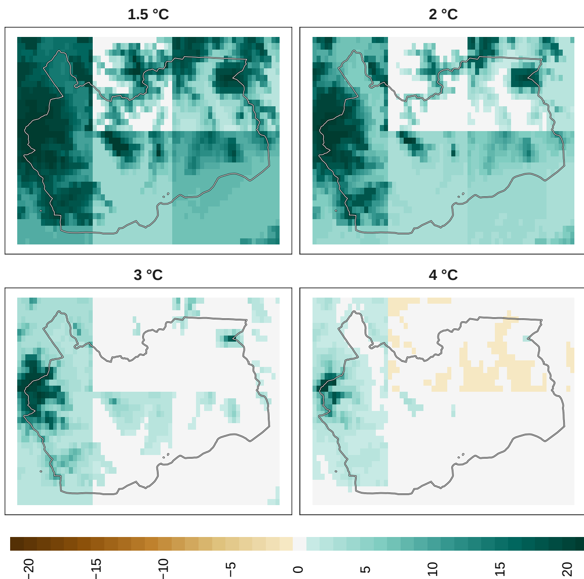
Figure 9: Adaptation effort for overall biodiversity at 1 km resolution.
