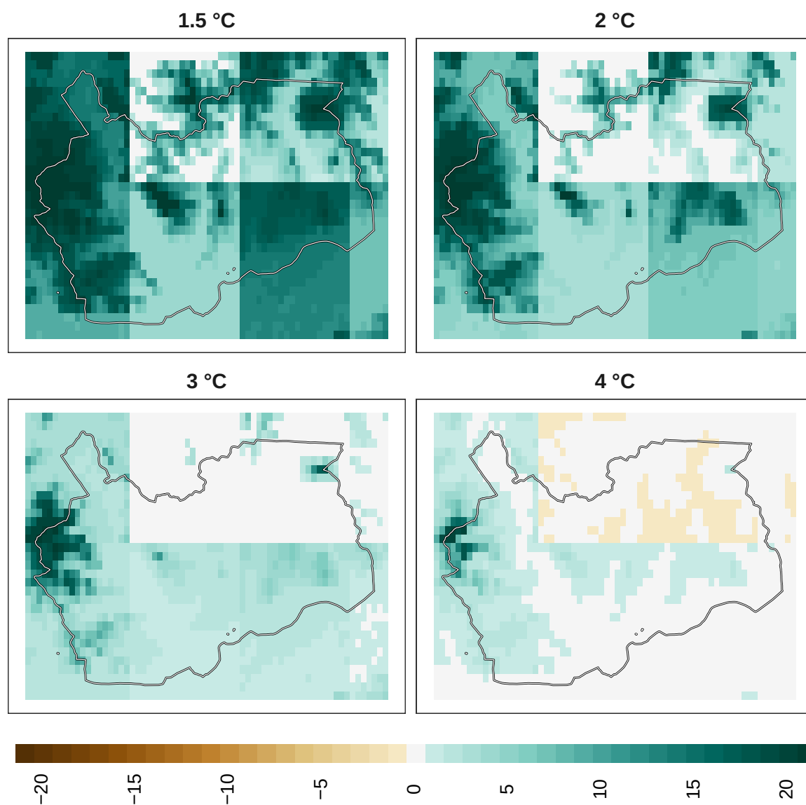
Figure 10: Adaptation effort for plants at 1 km resolution.
