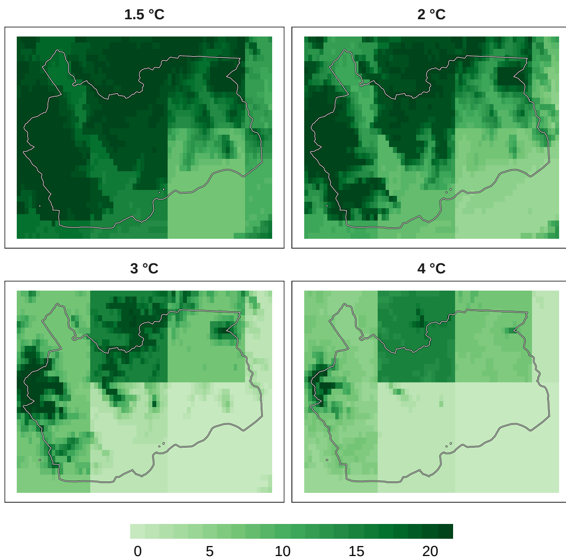
Figure 7: Number of models in agreement for bird refugia.
