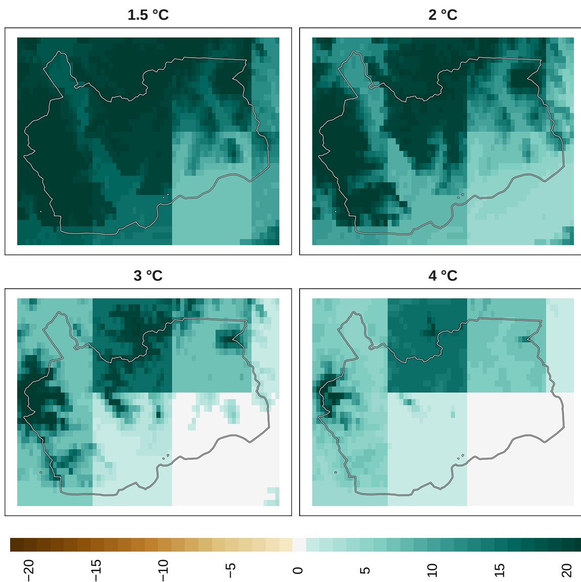
Figure 11: Adaptation effort for birds at 1 km resolution.
