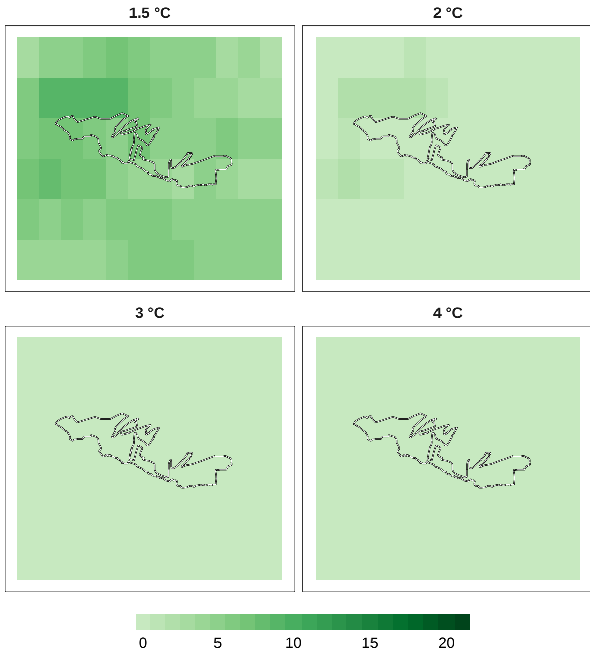
Figure 10: Number of models in agreement for insect refugia at 1 km resolution.
