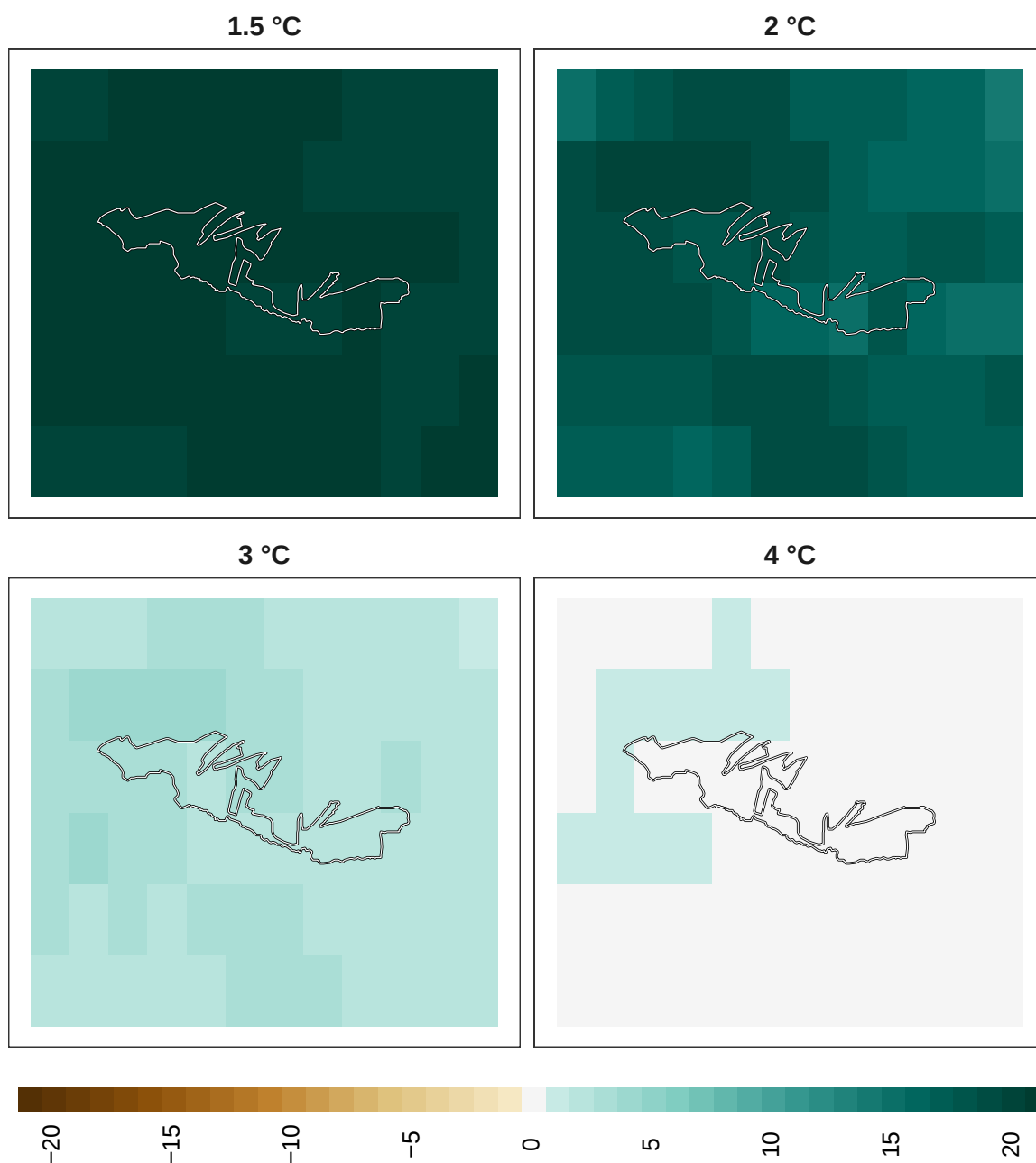
Figure 14: Adaptation effort for mammals at 1 km resolution.
