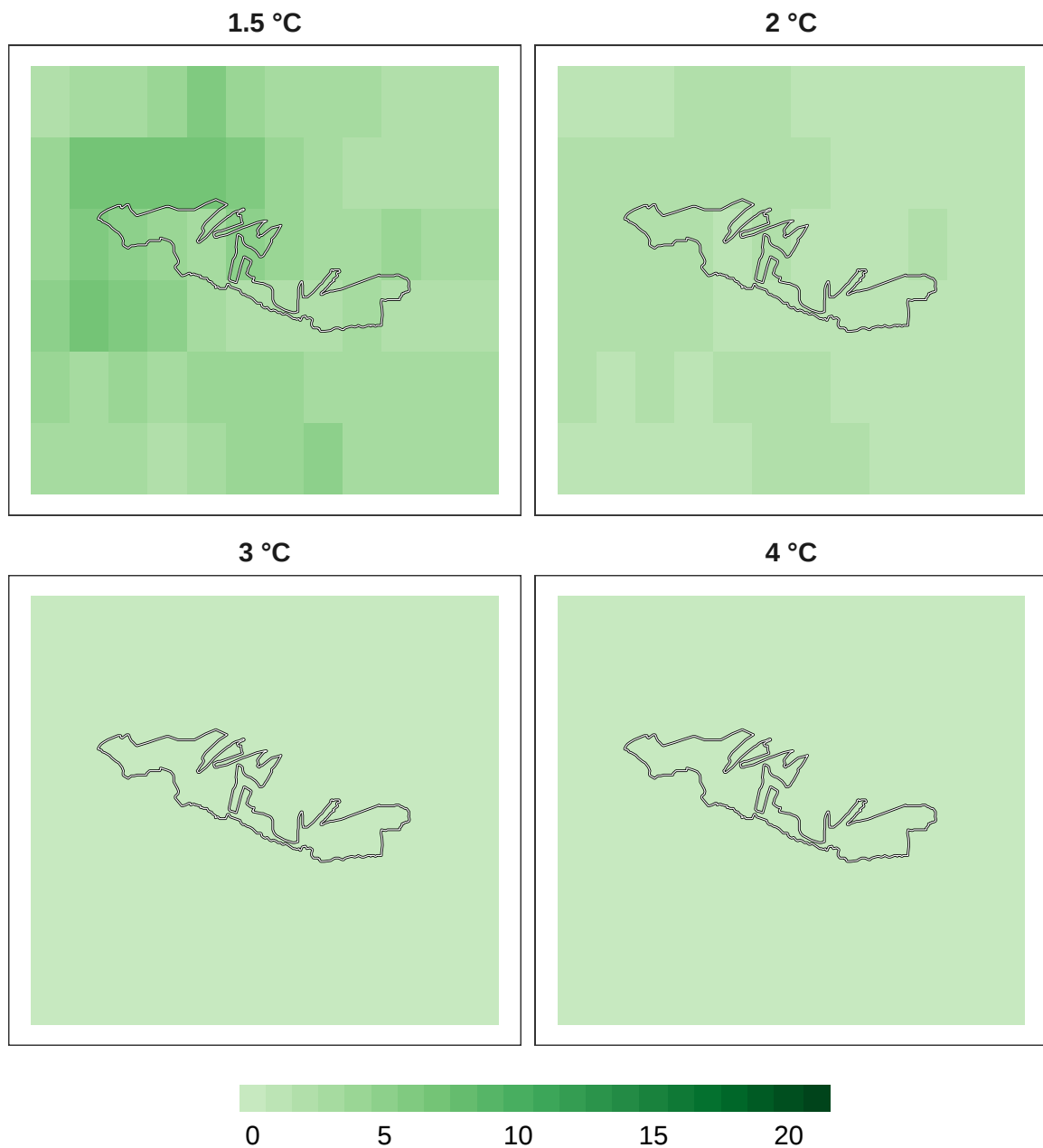
Figure 7: Number of models in agreement for plant refugia at 1 km resolution.
