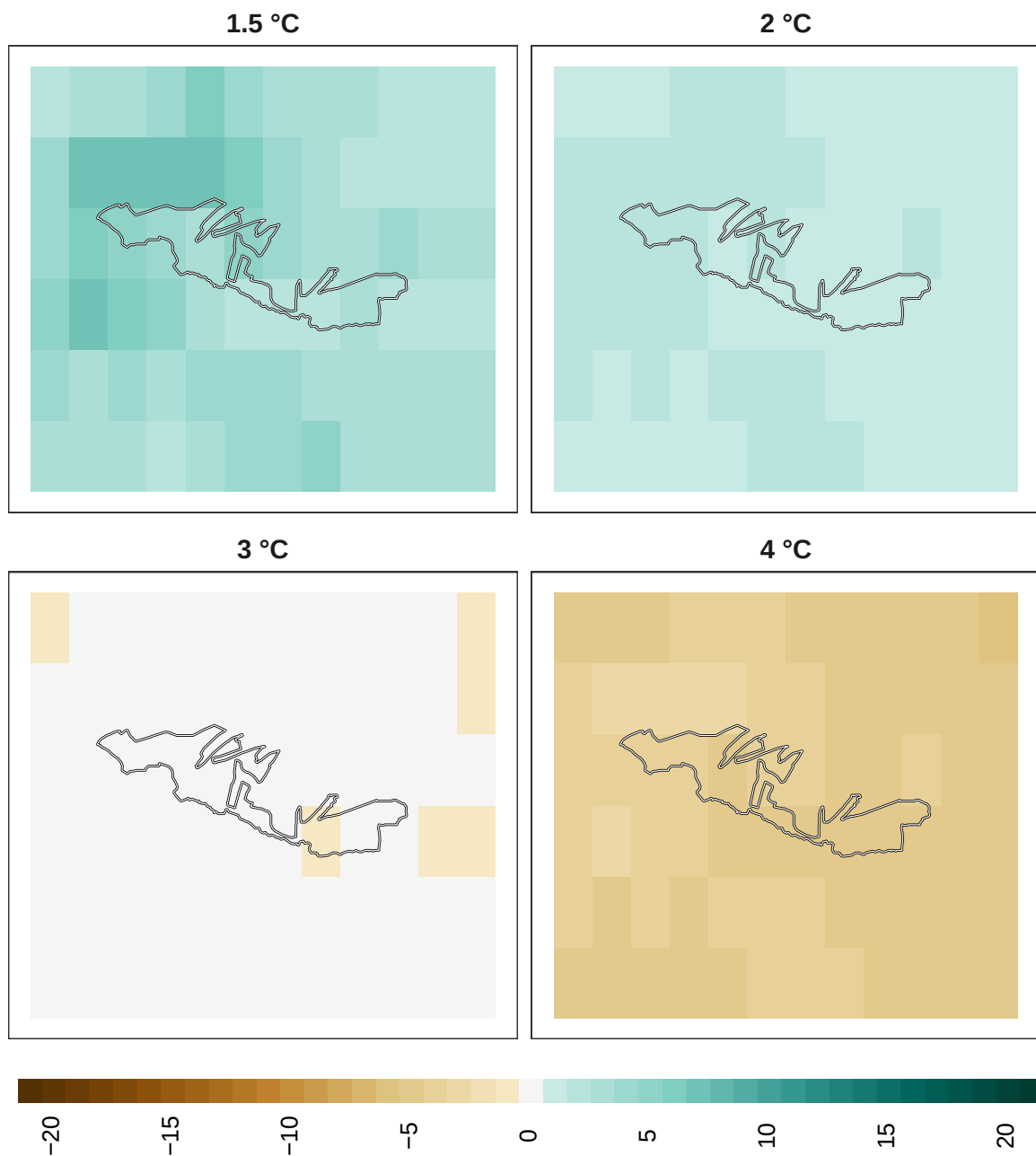
Figure 12: Adaptation effort for plants at 1 km resolution.
