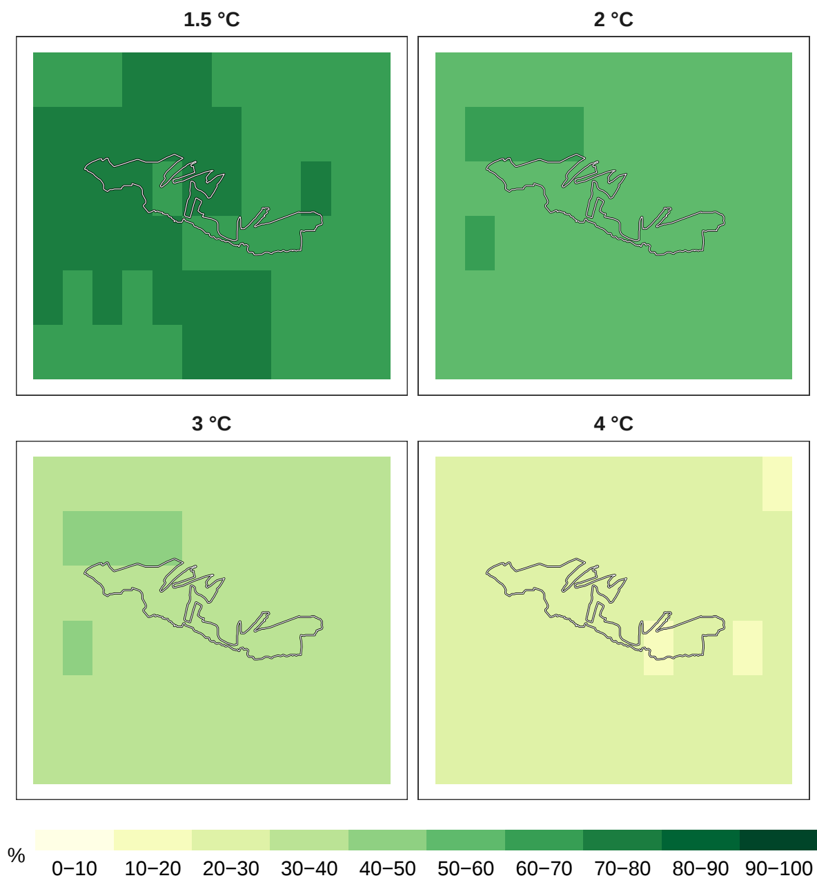
Figure 5: Percent insects remaining at 1 km resolution.
