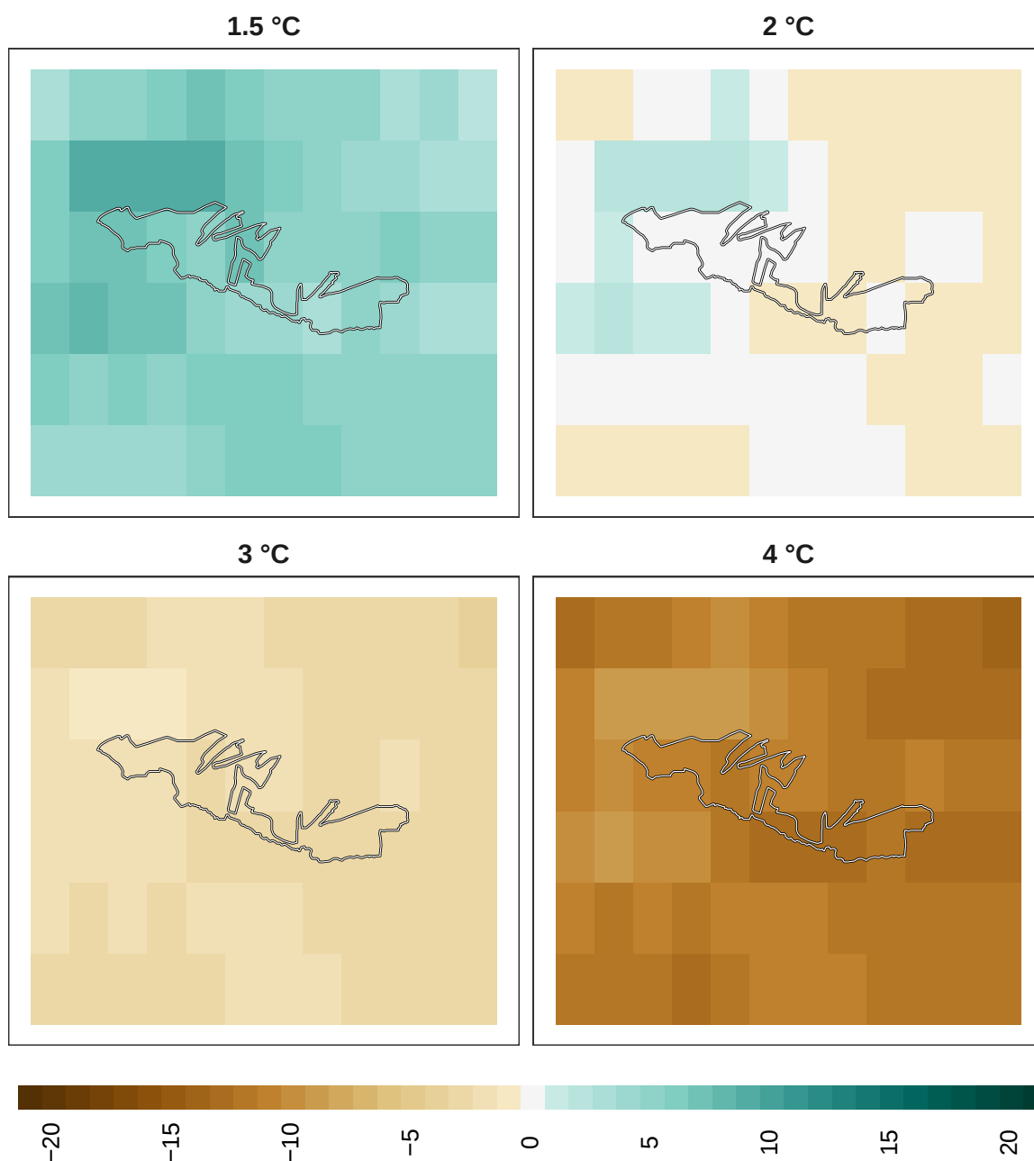
Figure 15: Adaptation effort for insects at 1 km resolution.
