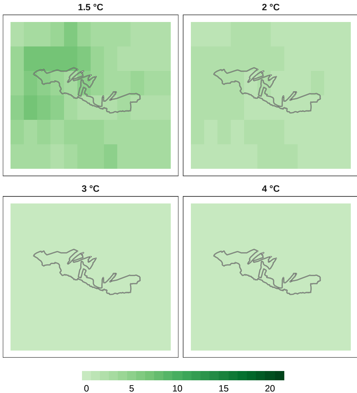
Figure 6: Number of models in agreement for overall biodiversity refugia at 1 km resolution.
