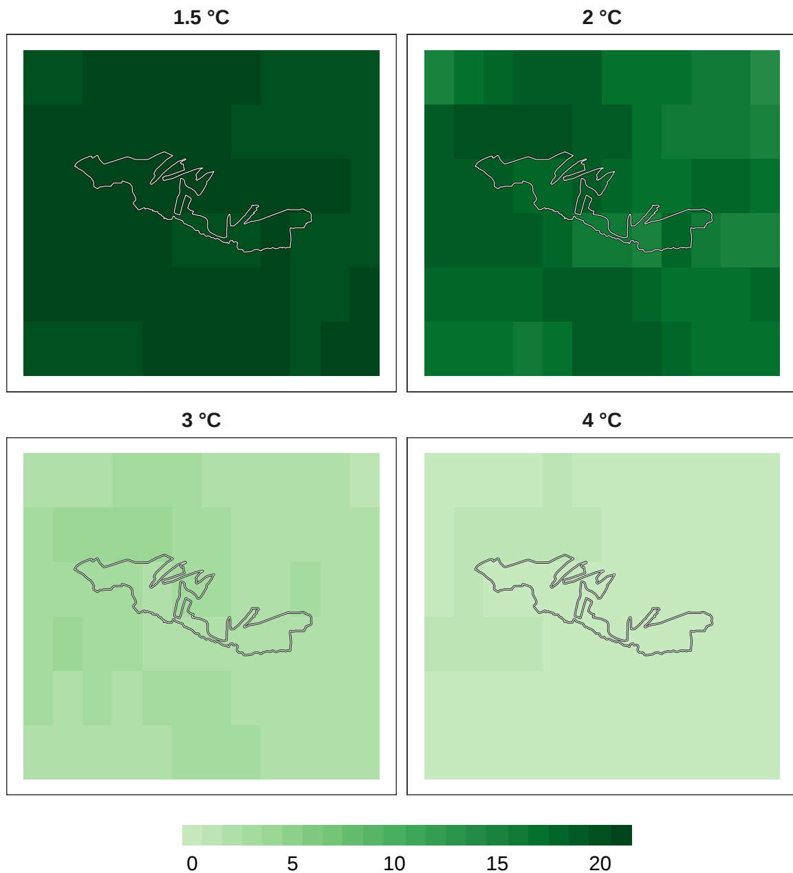
Figure 9: Number of models in agreement for mammal refugia at 1 km resolution.
