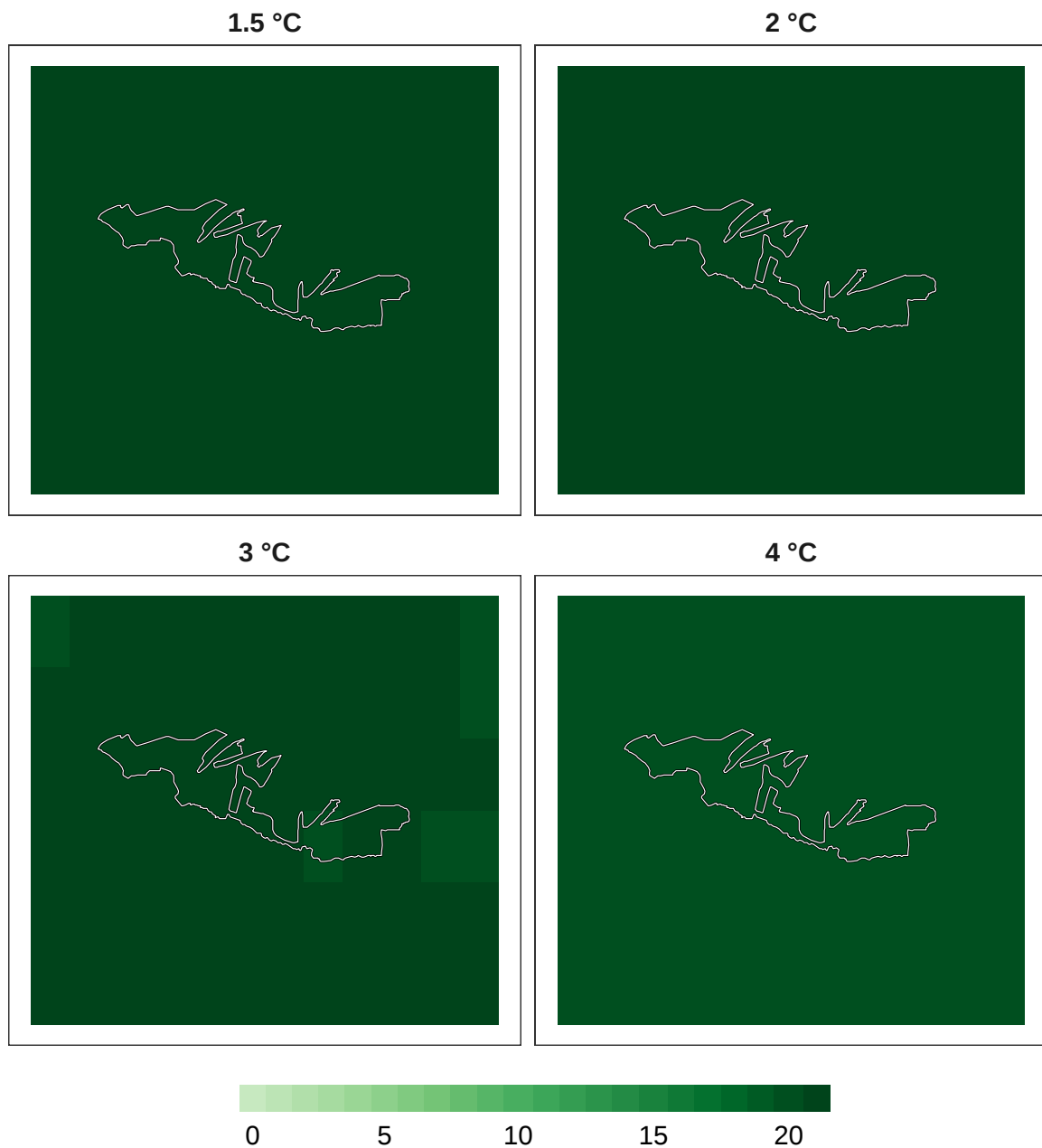
Figure 8: Number of models in agreement for bird refugia.
