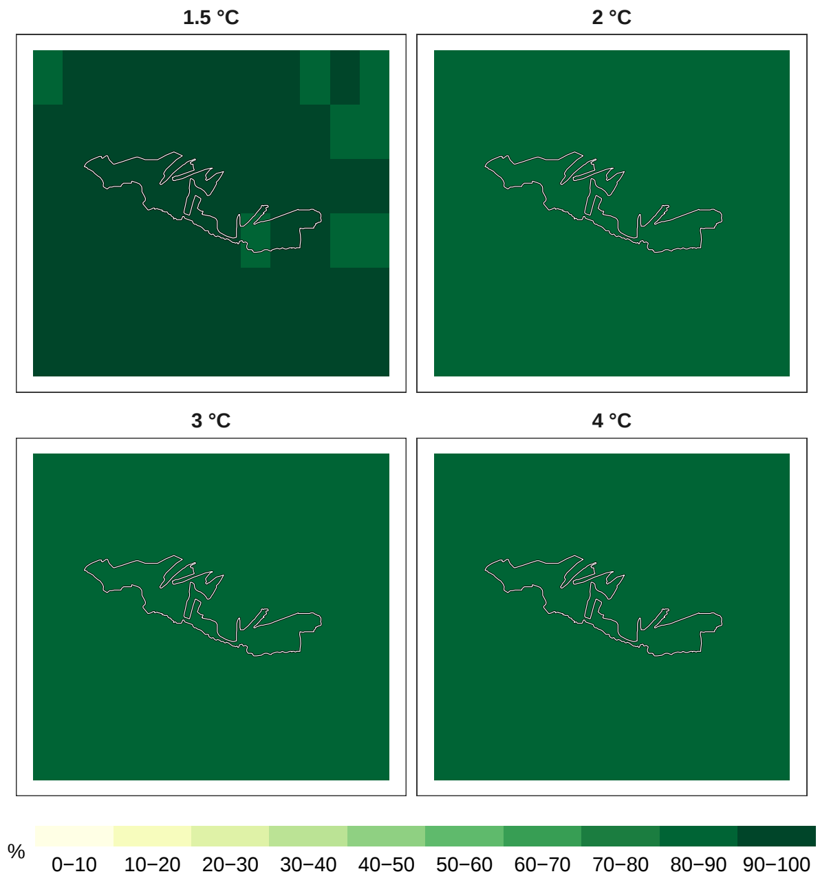
Figure 3: Percent birds remaining at 1 km resolution.
