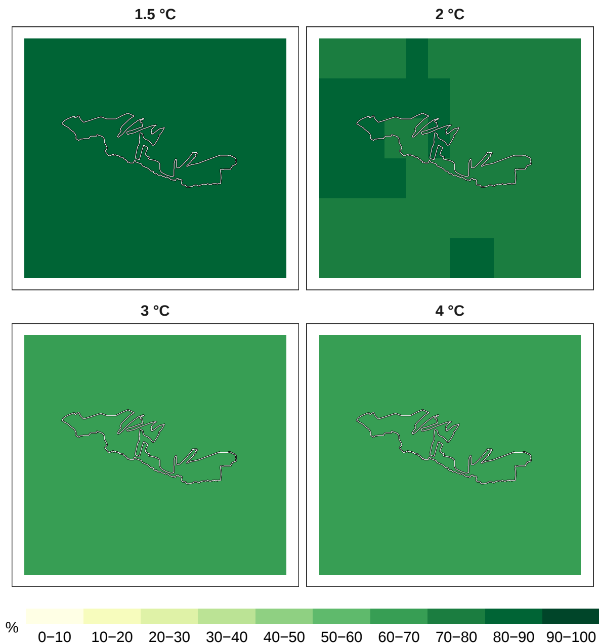
Figure 4: Percent mammals remaining at 1 km resolution.
