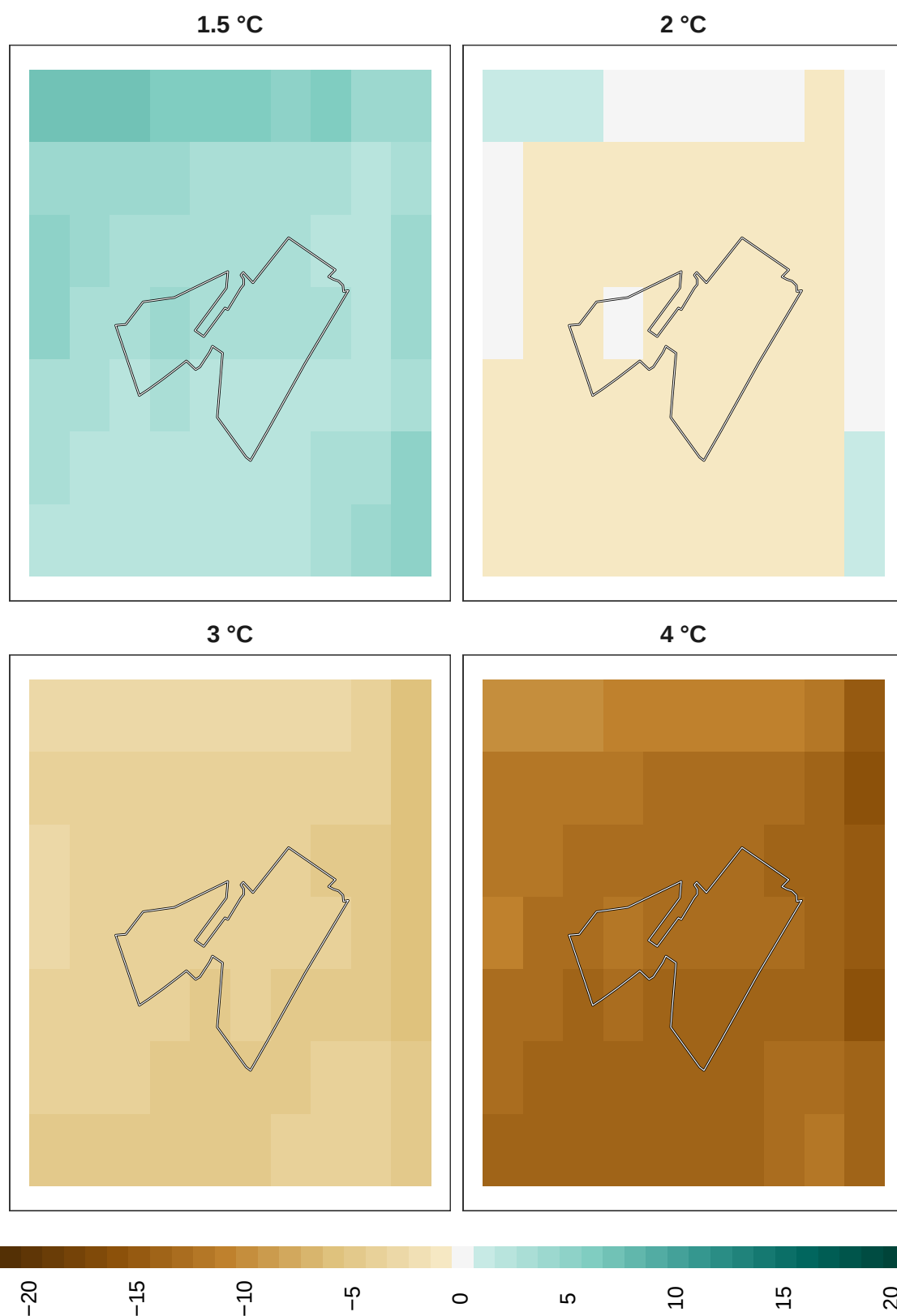
Figure 16: Adaptation effort for insects at 1 km resolution.
