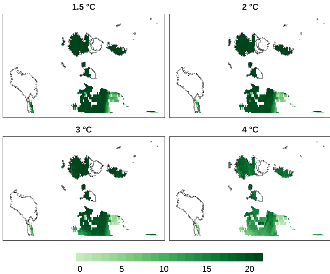
Figure 10: Number of models in agreement for mammal refugia at 1 km resolution.
