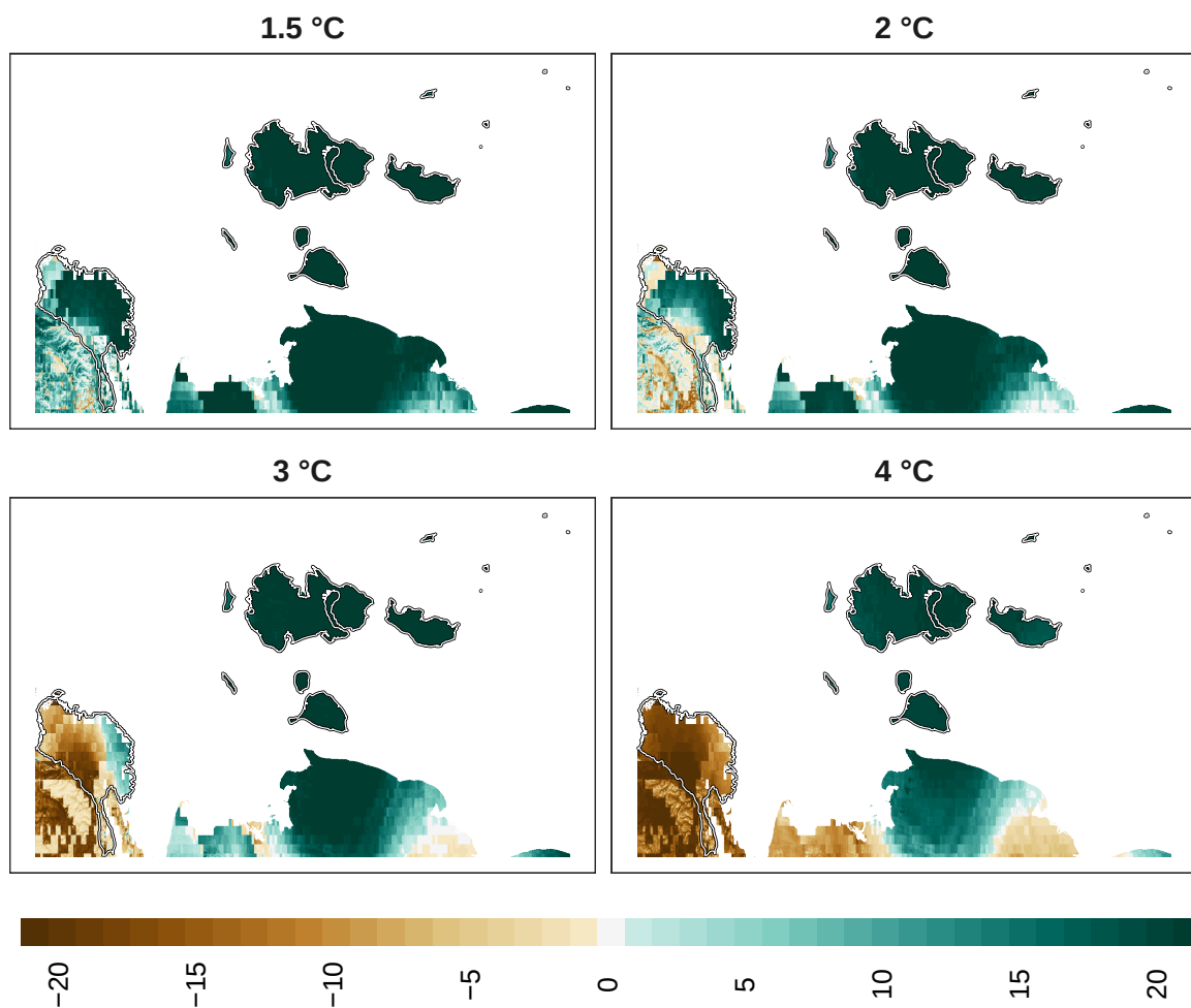
Figure 14: Adaptation effort for plants at 1 km resolution.
