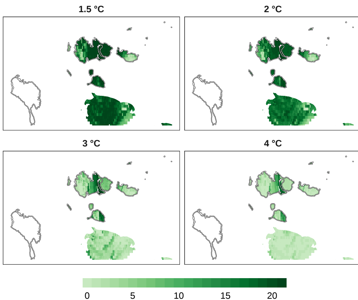
Figure 9: Number of models in agreement for bird refugia.
