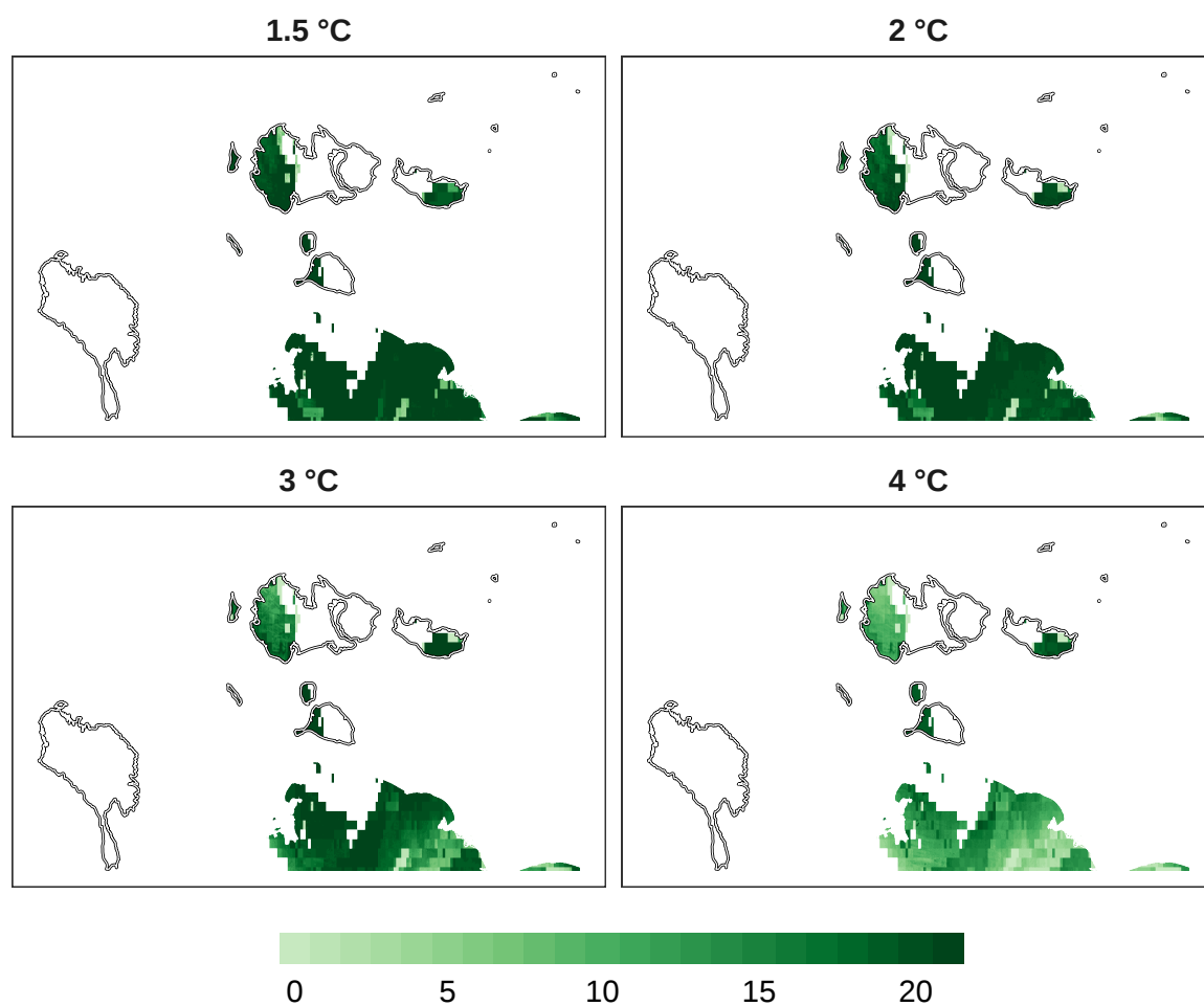
Figure 11: Number of models in agreement for insect refugia at 1 km resolution.
