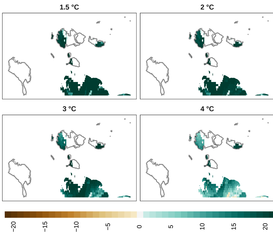
Figure 17: Adaptation effort for insects at 1 km resolution.
