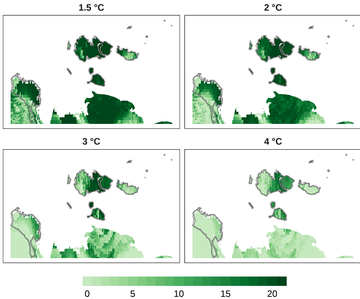
Figure 7: Number of models in agreement for overall biodiversity refugia at 1 km resolution.
