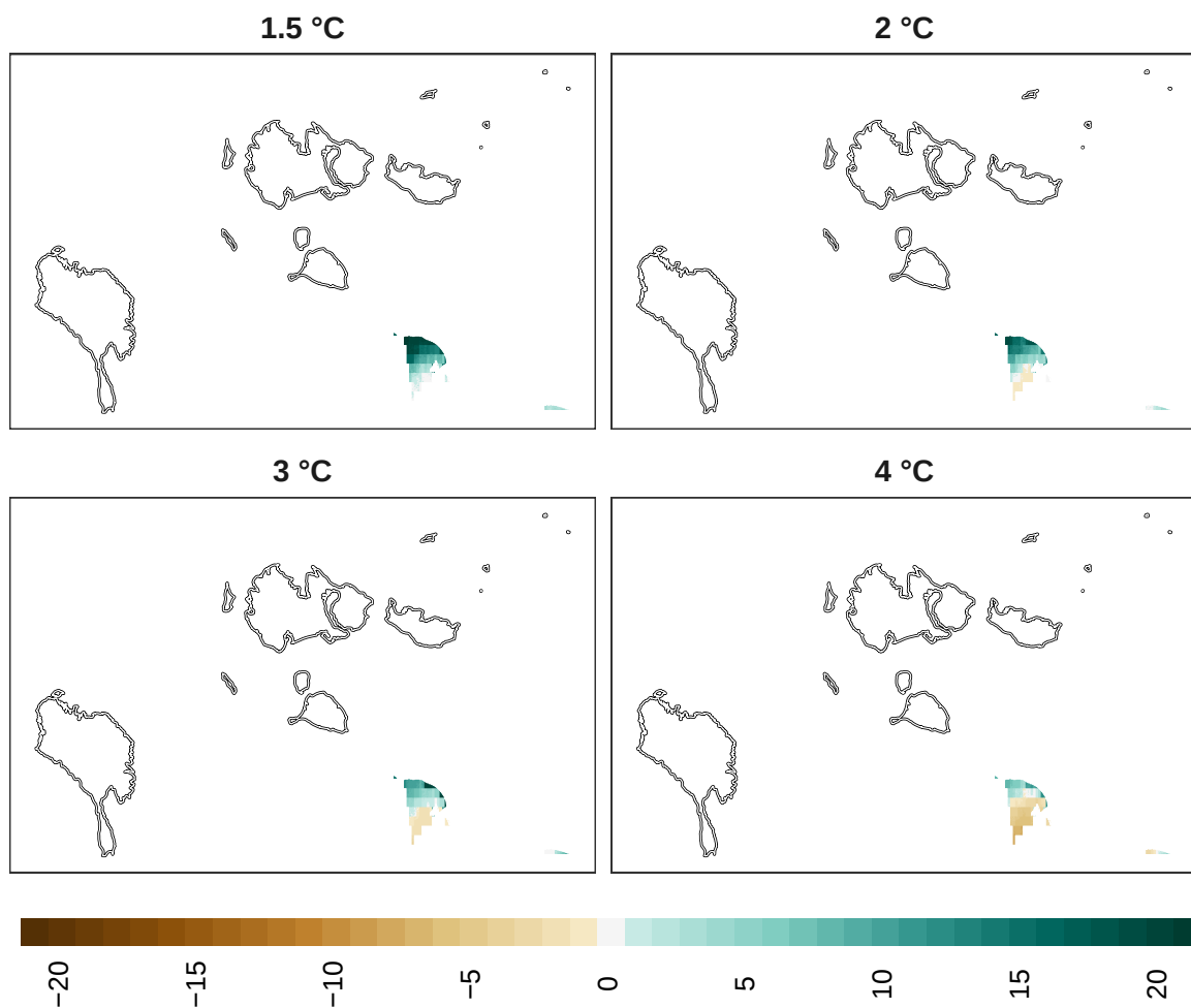
Figure 18: Adaptation effort for pollinators at 1 km resolution.
