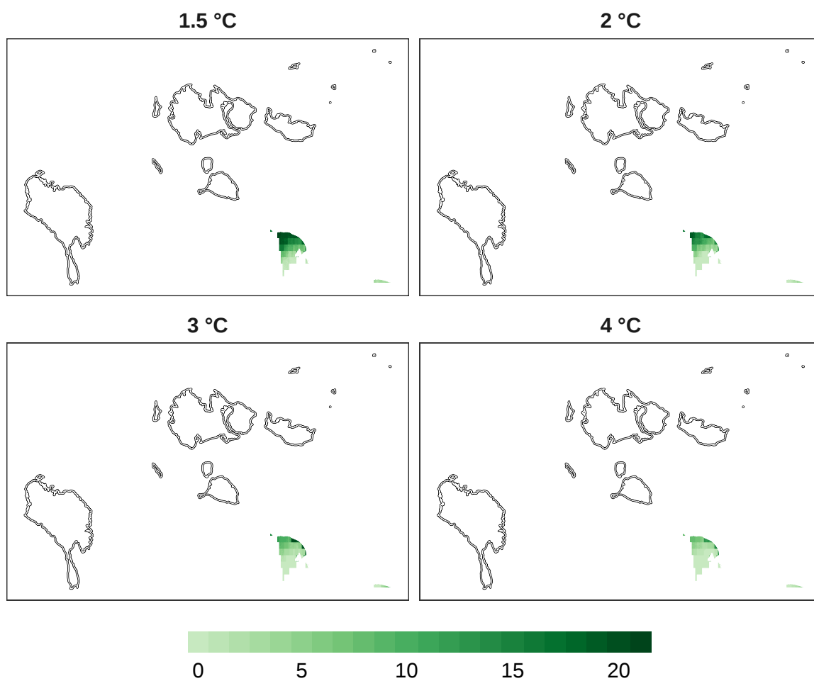
Figure 12: Number of models in agreement for pollinator refugia at 1 km resolution.
