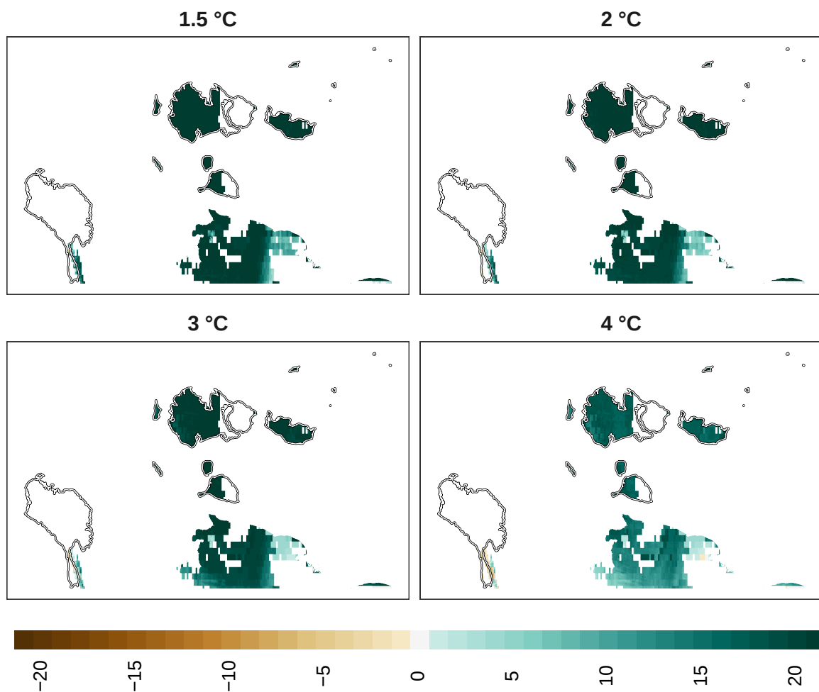
Figure 16: Adaptation effort for mammals at 1 km resolution.
