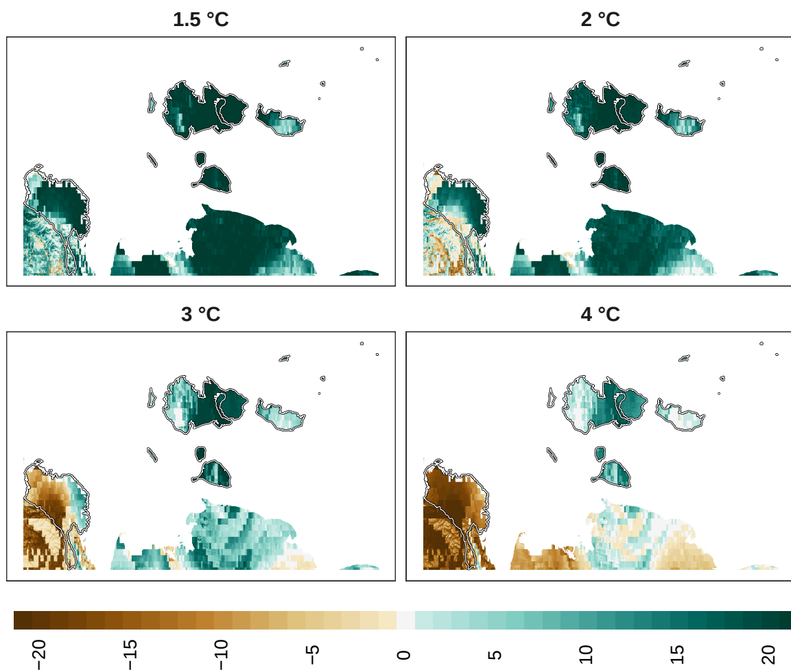
Figure 13: Adaptation effort for overall biodiversity at 1 km resolution.
