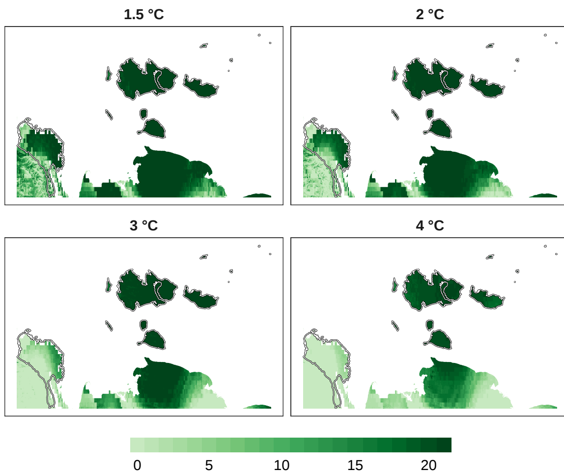
Figure 8: Number of models in agreement for plant refugia at 1 km resolution.
