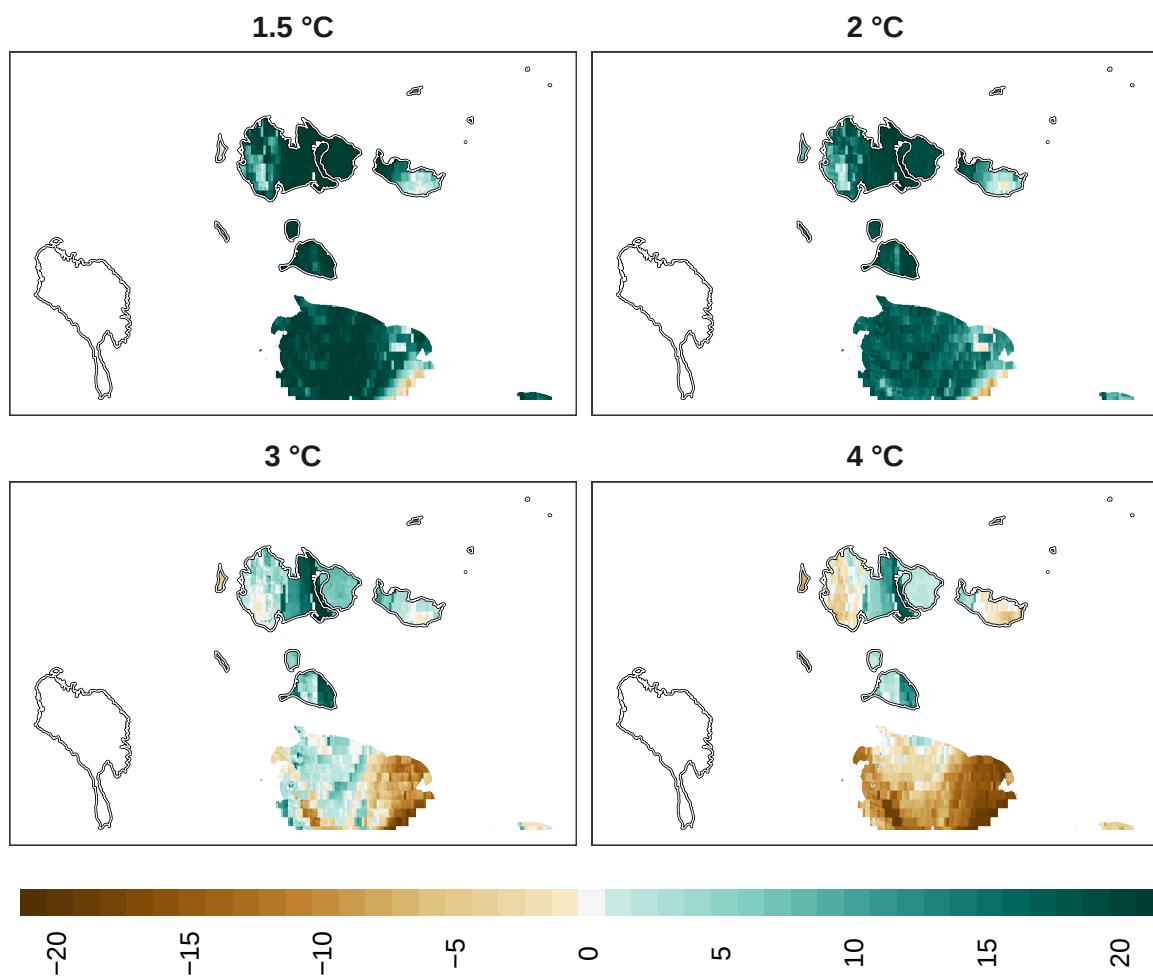
Figure 15: Adaptation effort for birds at 1 km resolution.
