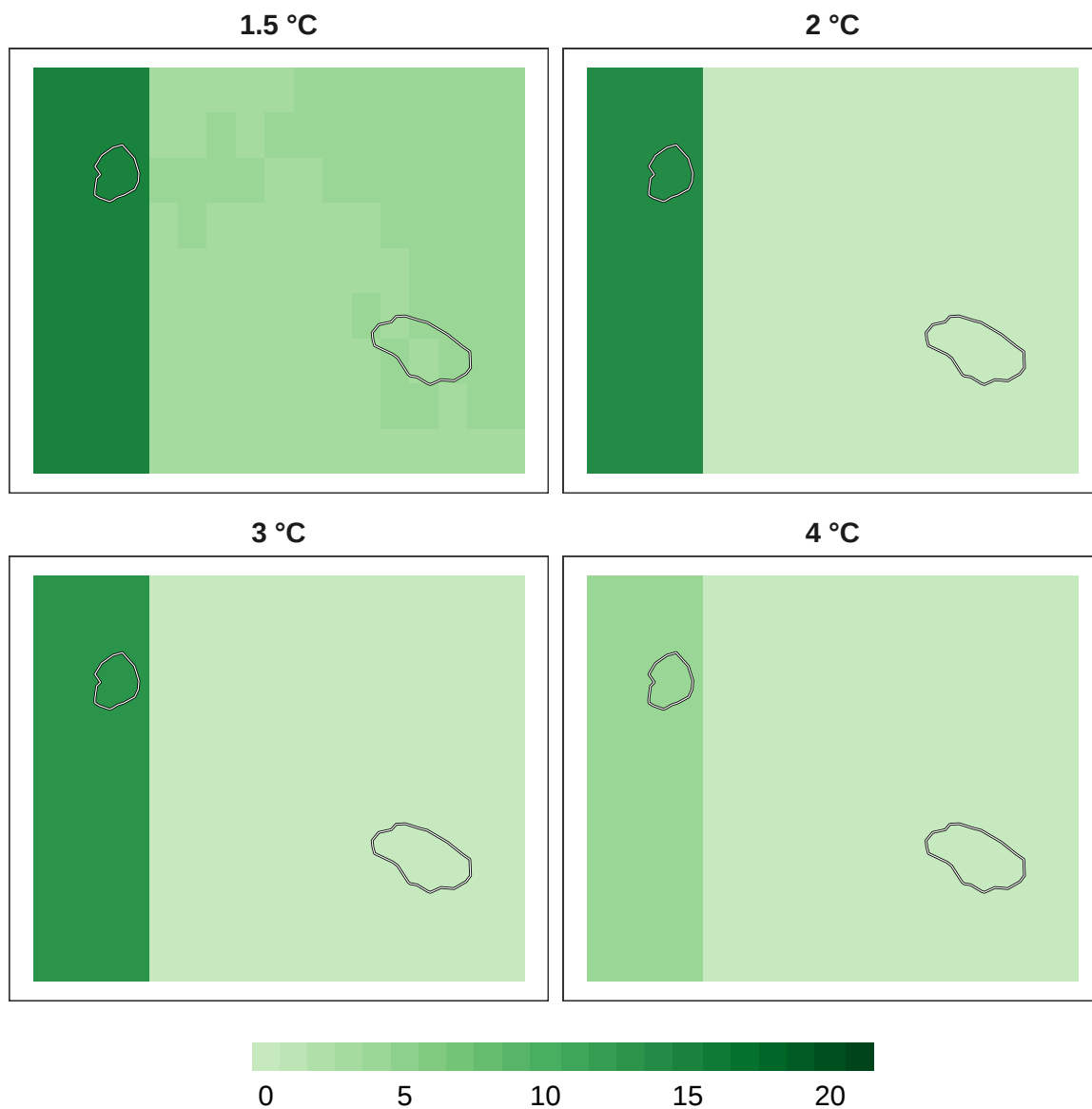
Figure 7: Number of models in agreement for overall biodiversity refugia at 1 km resolution.
