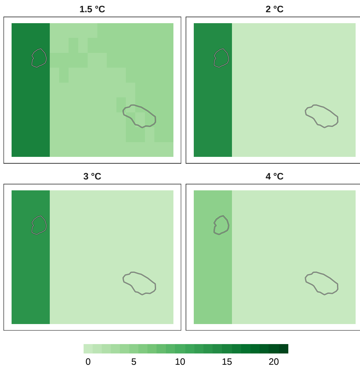
Figure 8: Number of models in agreement for plant refugia at 1 km resolution.
