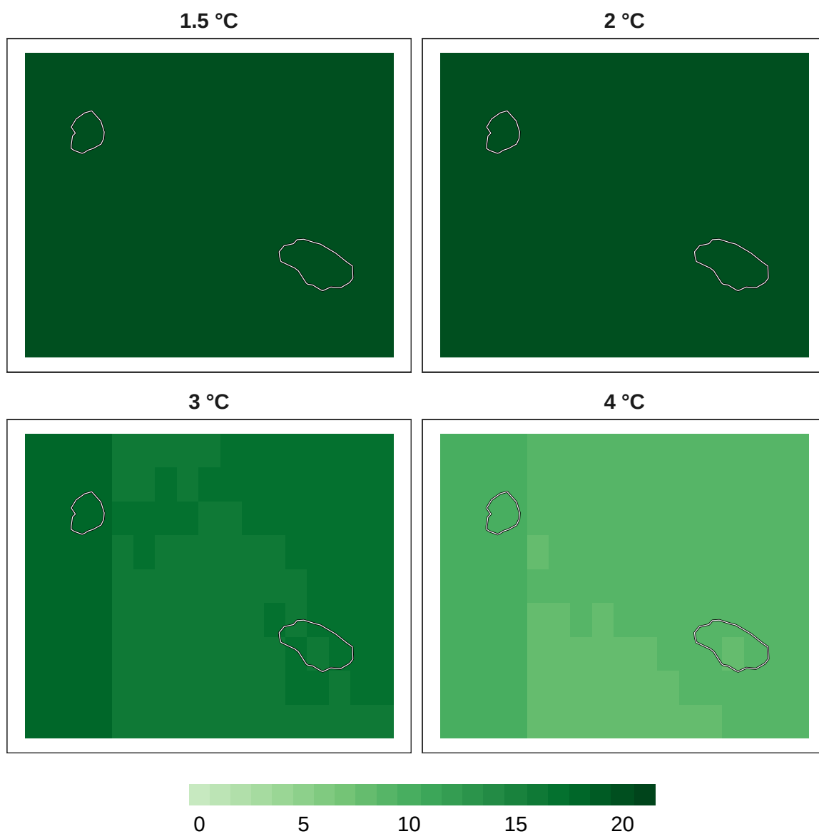
Figure 9: Number of models in agreement for bird refugia.
