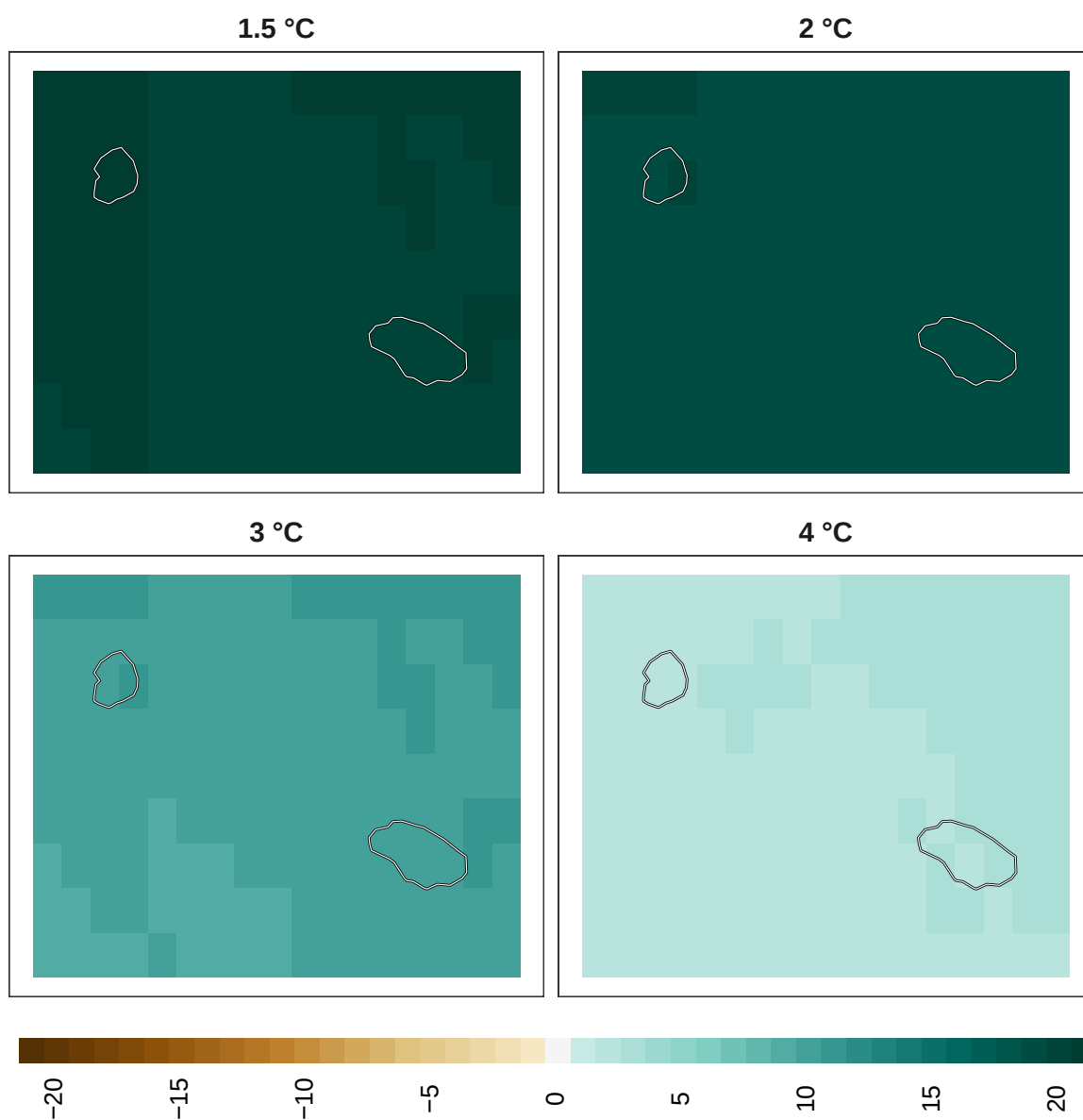
Figure 16: Adaptation effort for mammals at 1 km resolution.
