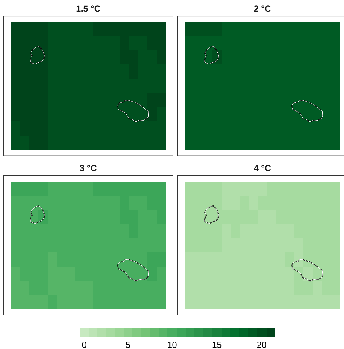
Figure 10: Number of models in agreement for mammal refugia at 1 km resolution.
