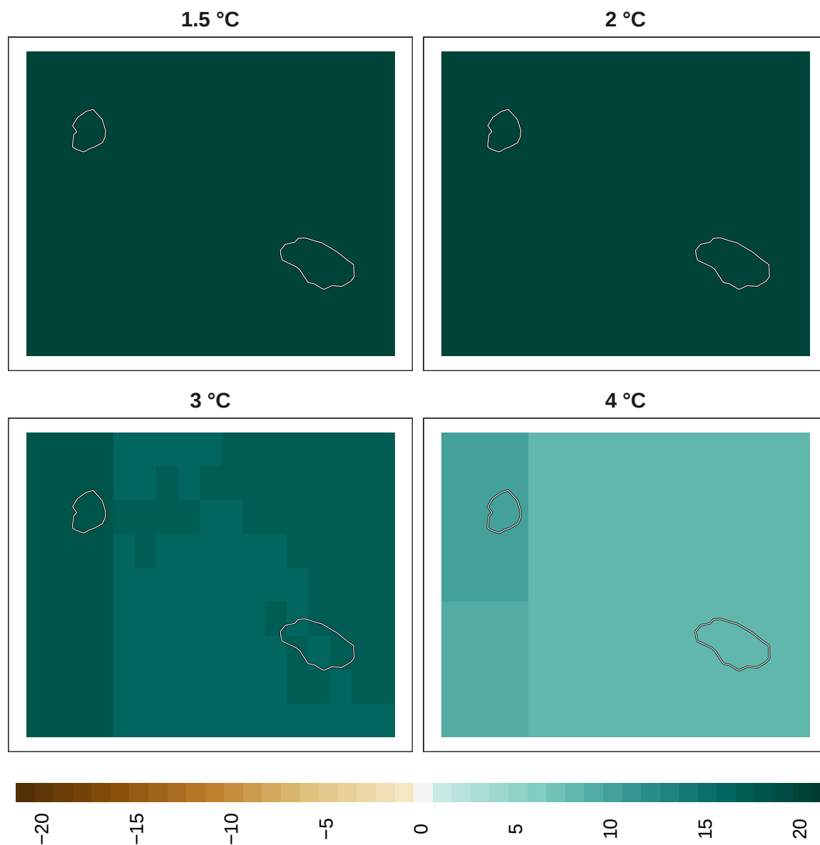
Figure 15: Adaptation effort for birds at 1 km resolution.
