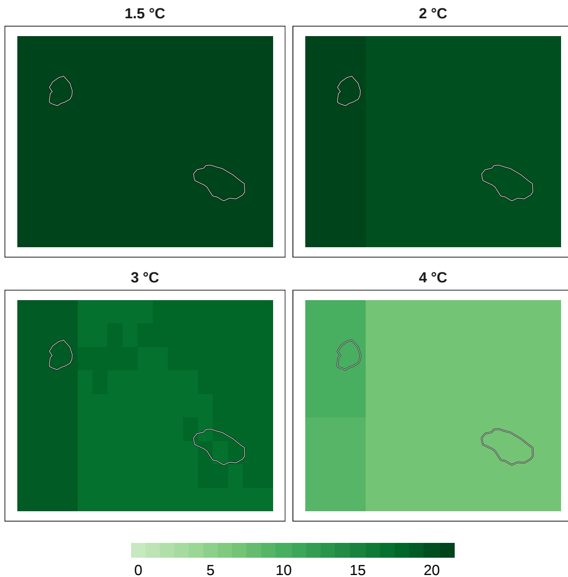
Figure 11: Number of models in agreement for reptile refugia at 1 km resolution.
