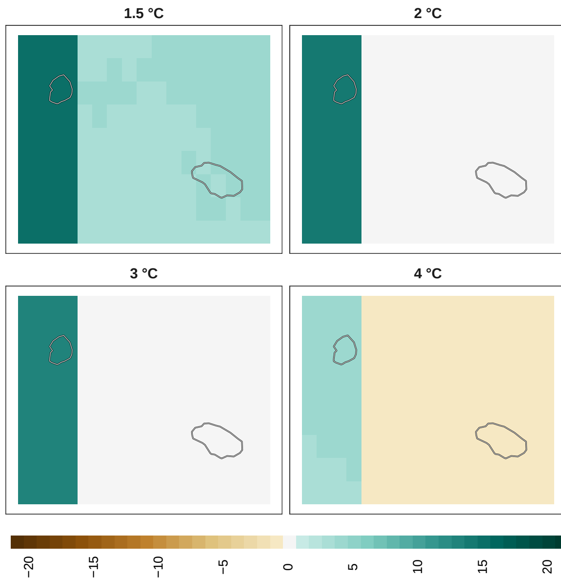
Figure 13: Adaptation effort for overall biodiversity at 1 km resolution.
