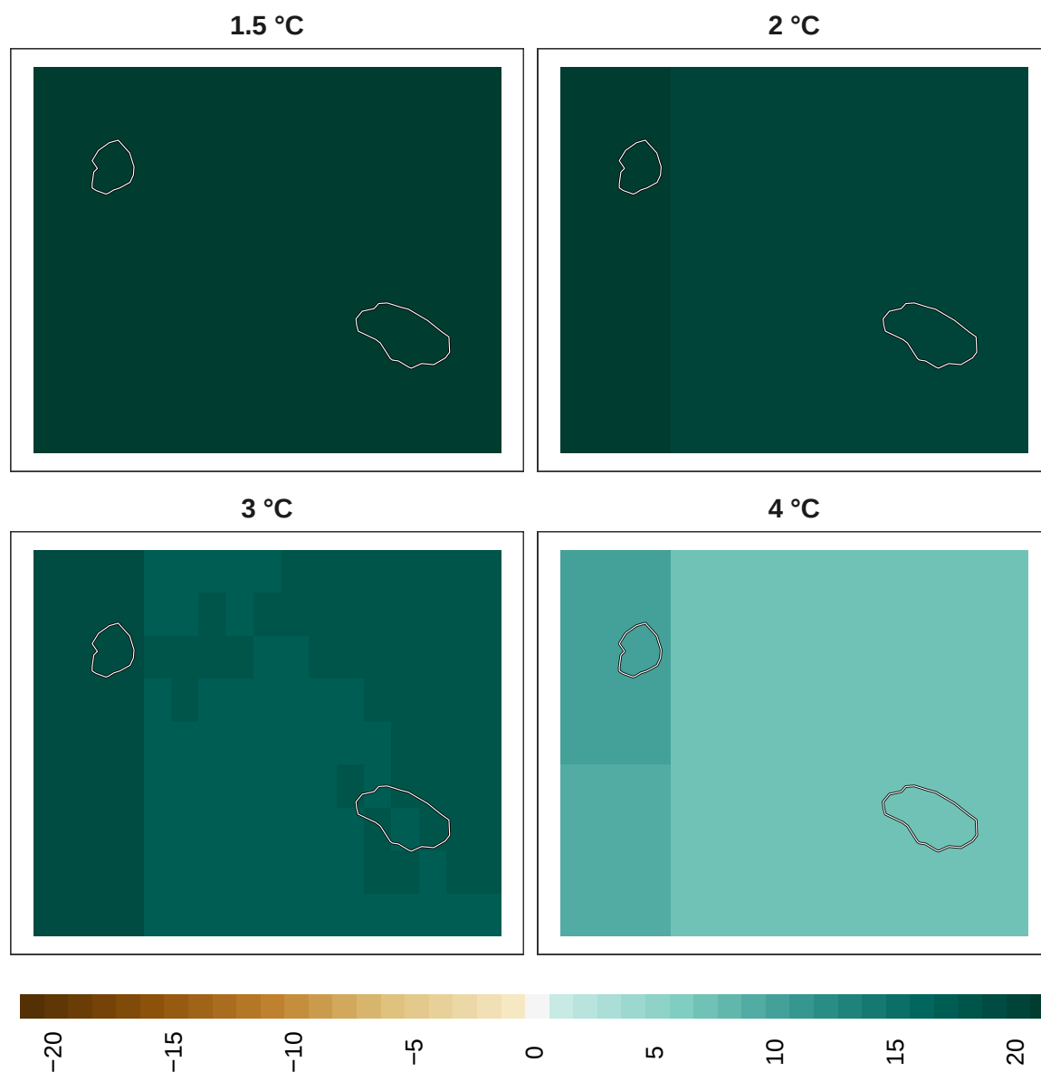
Figure 17: Adaptation effort for reptiles at 1 km resolution.
