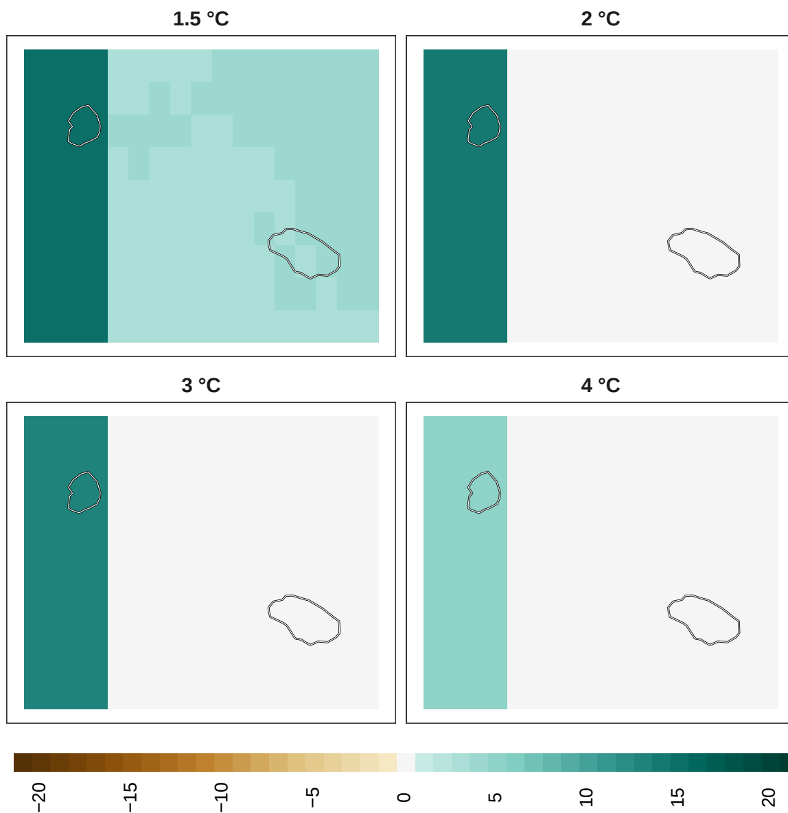
Figure 14: Adaptation effort for plants at 1 km resolution.
