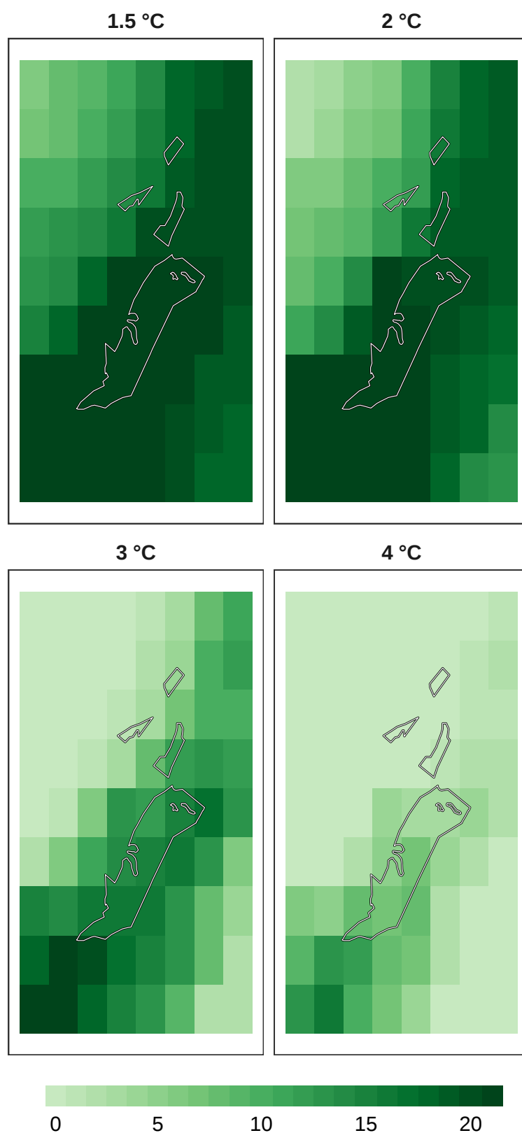
Figure 6: Number of models in agreement for overall biodiversity refugia at 1 km resolution.
