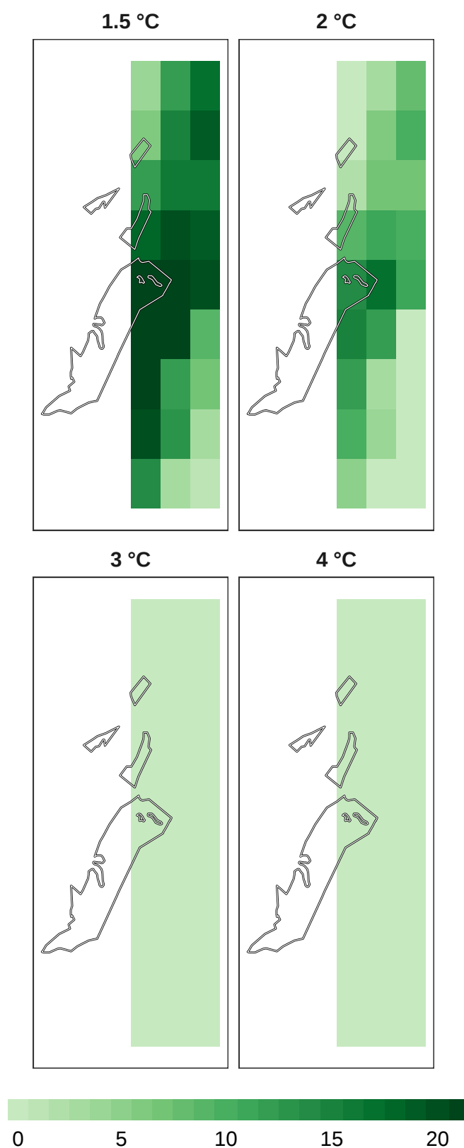
Figure 9: Number of models in agreement for mammal refugia at 1 km resolution.
