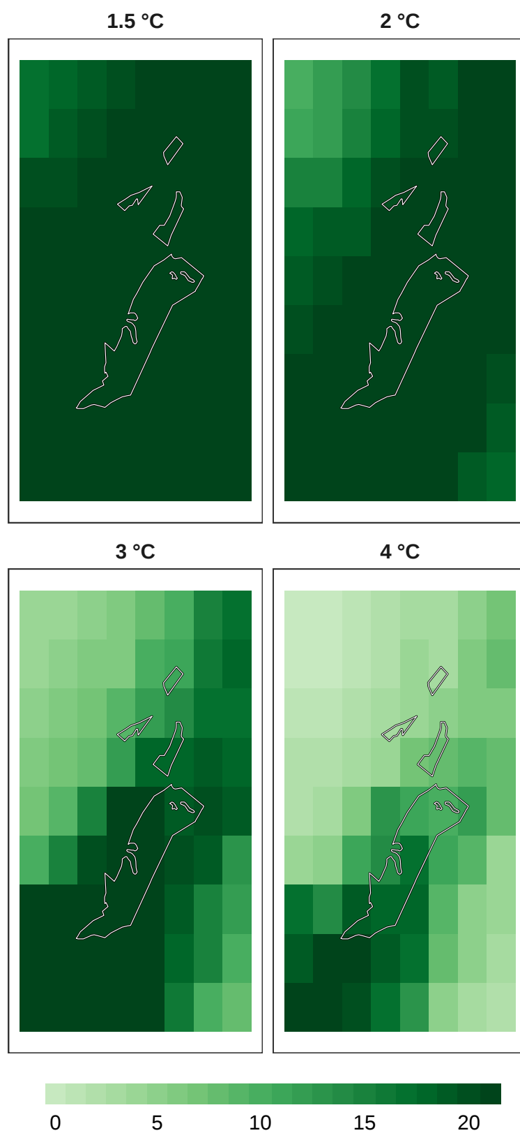
Figure 8: Number of models in agreement for bird refugia.
