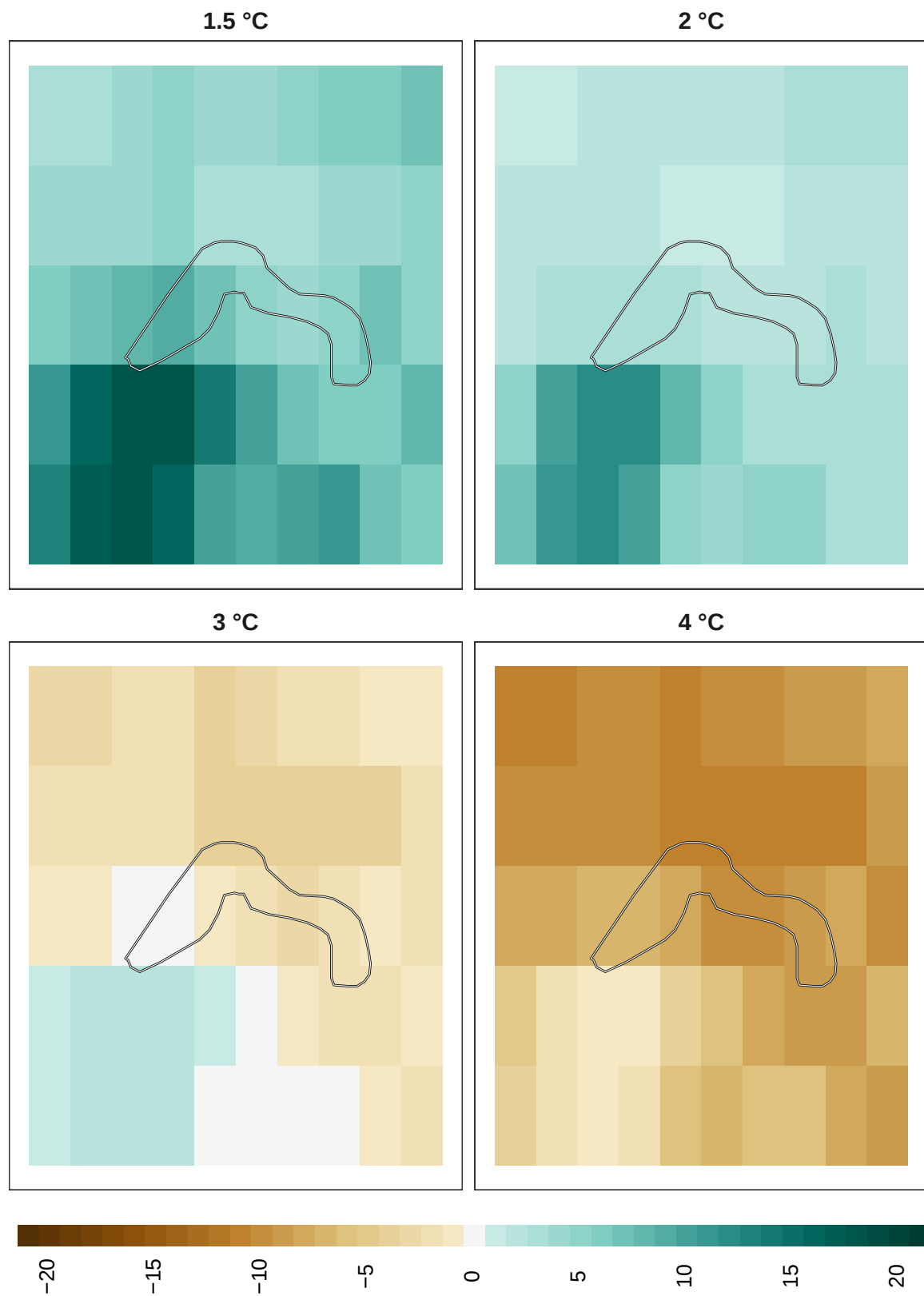
Figure 10: Adaptation effort for plants at 1 km resolution.
