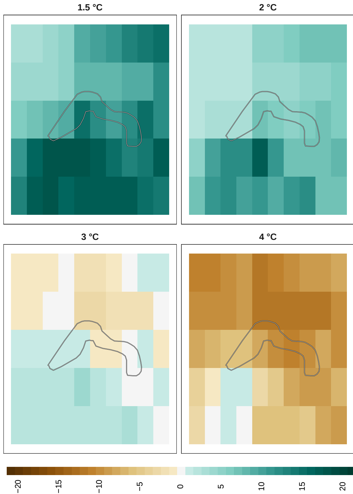
Figure 12: Adaptation effort for insects at 1 km resolution.
