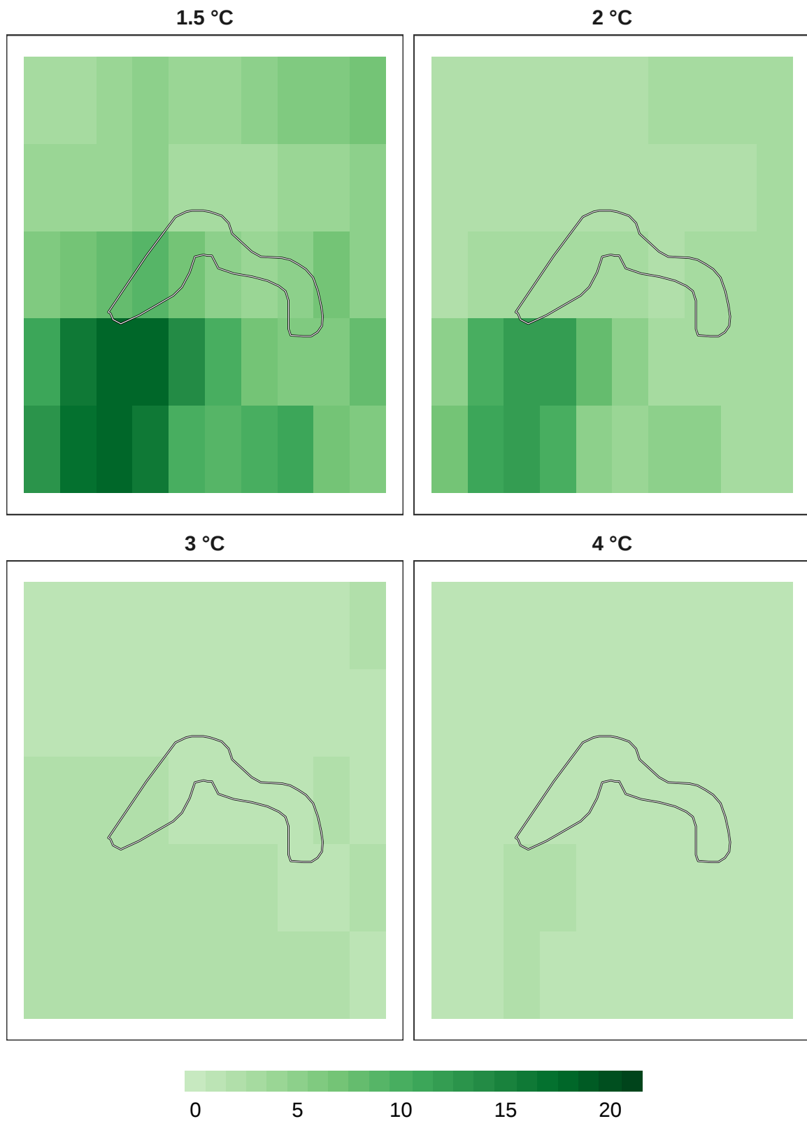
Figure 6: Number of models in agreement for plant refugia at 1 km resolution.
