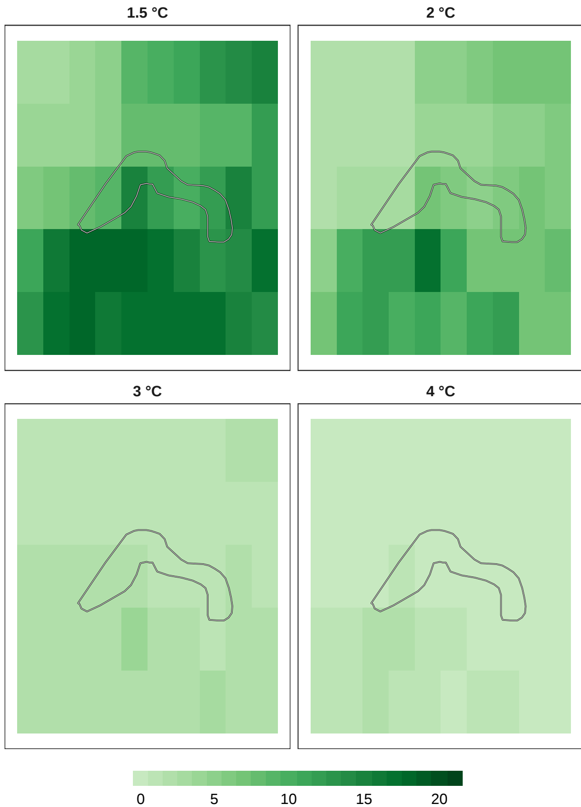
Figure 8: Number of models in agreement for insect refugia at 1 km resolution.
