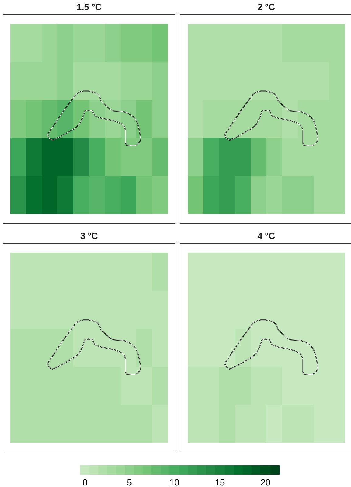
Figure 5: Number of models in agreement for overall biodiversity refugia at 1 km resolution.
