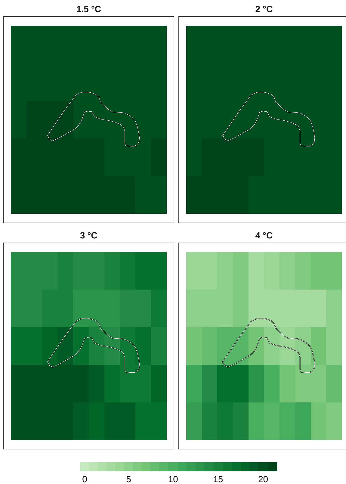
Figure 7: Number of models in agreement for mammal refugia at 1 km resolution.
