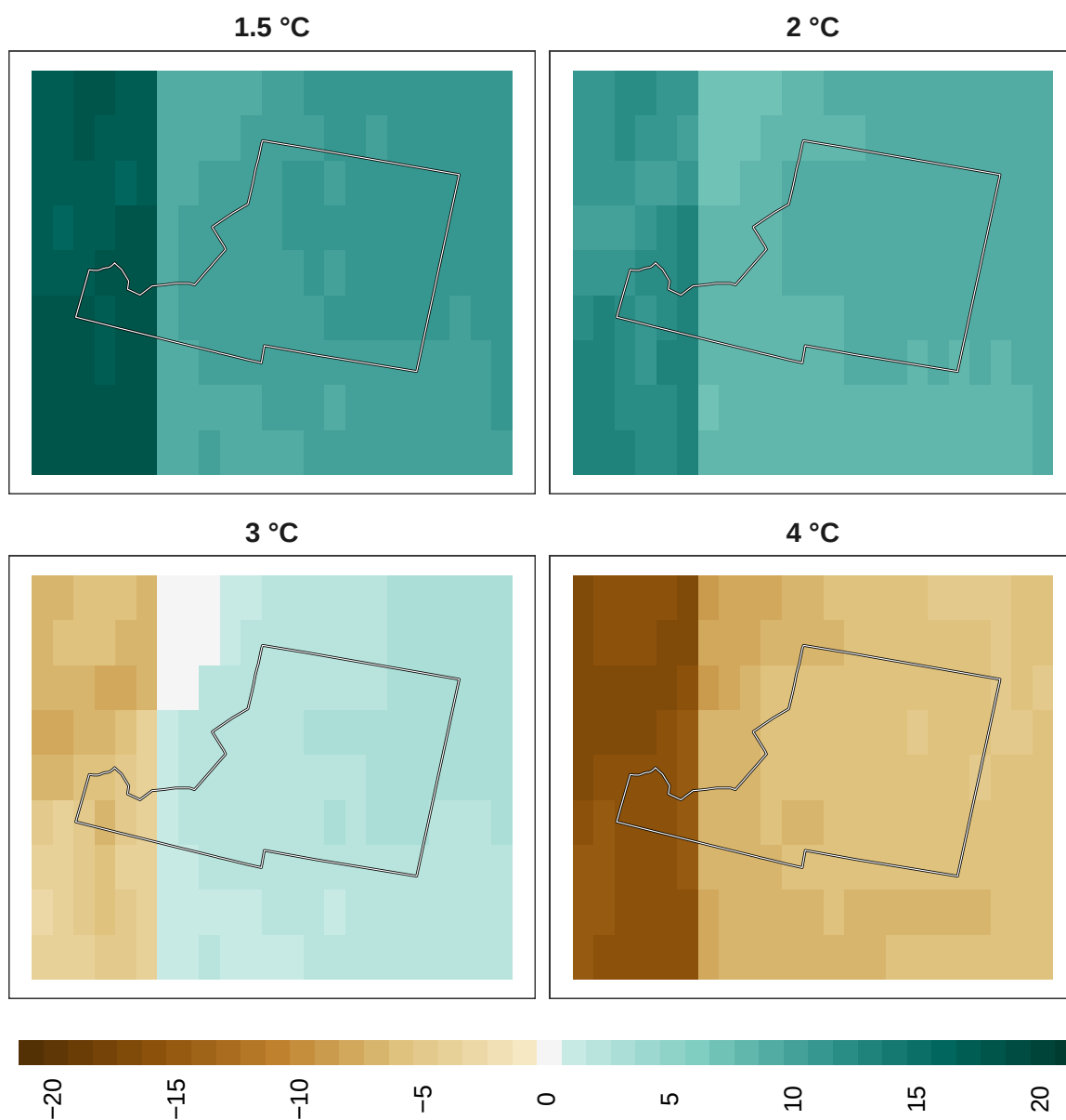
Figure 15: Adaptation effort for pollinators at 1 km resolution.
