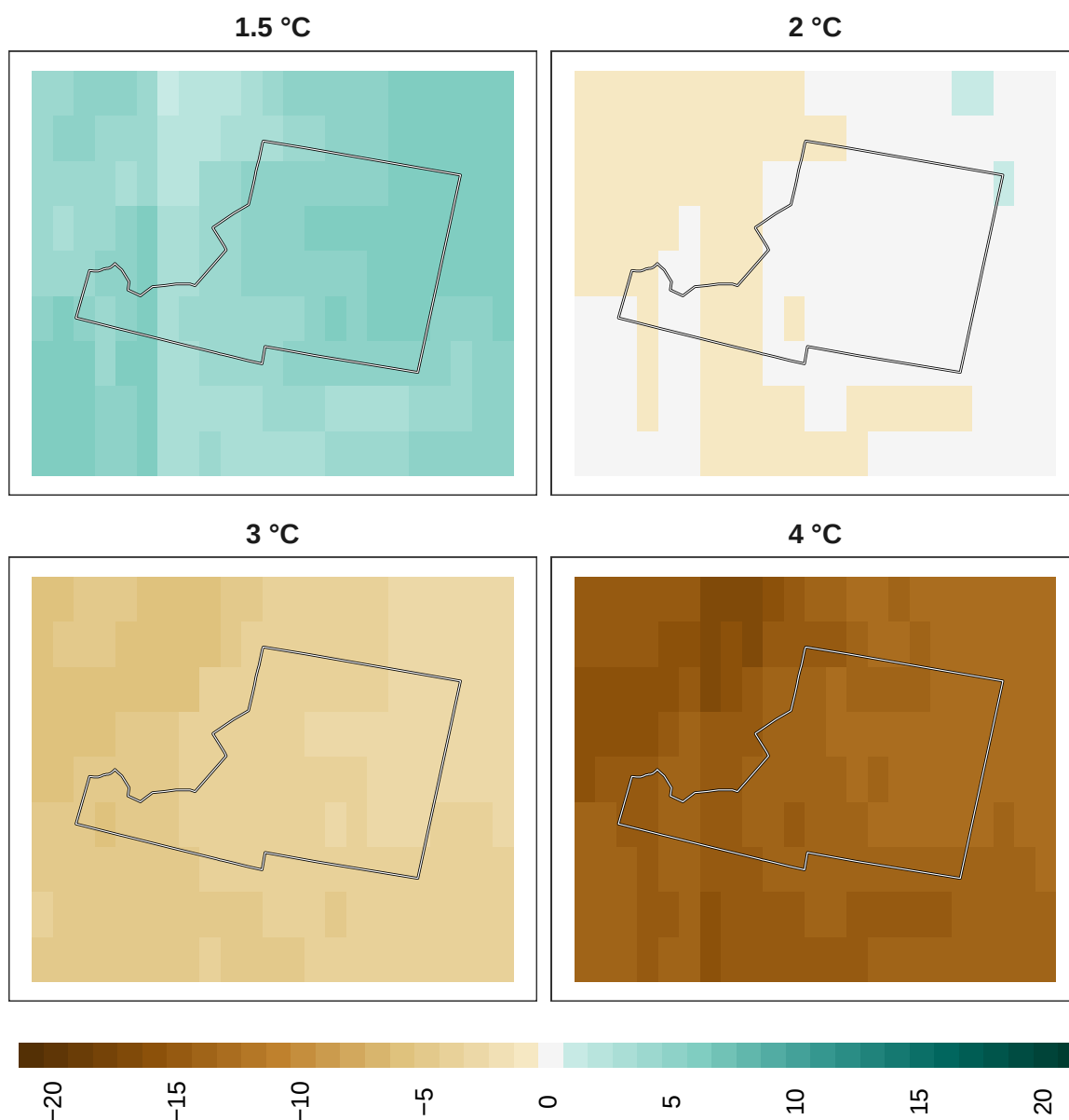
Figure 14: Adaptation effort for insects at 1 km resolution.
