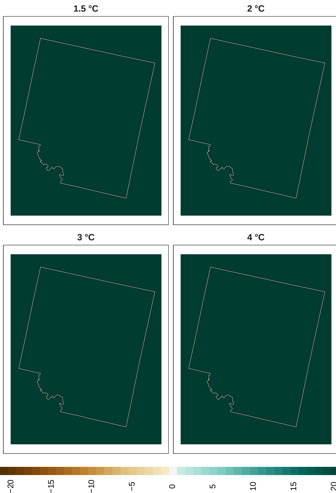
Figure 13: Adaptation effort for birds at 1 km resolution.
