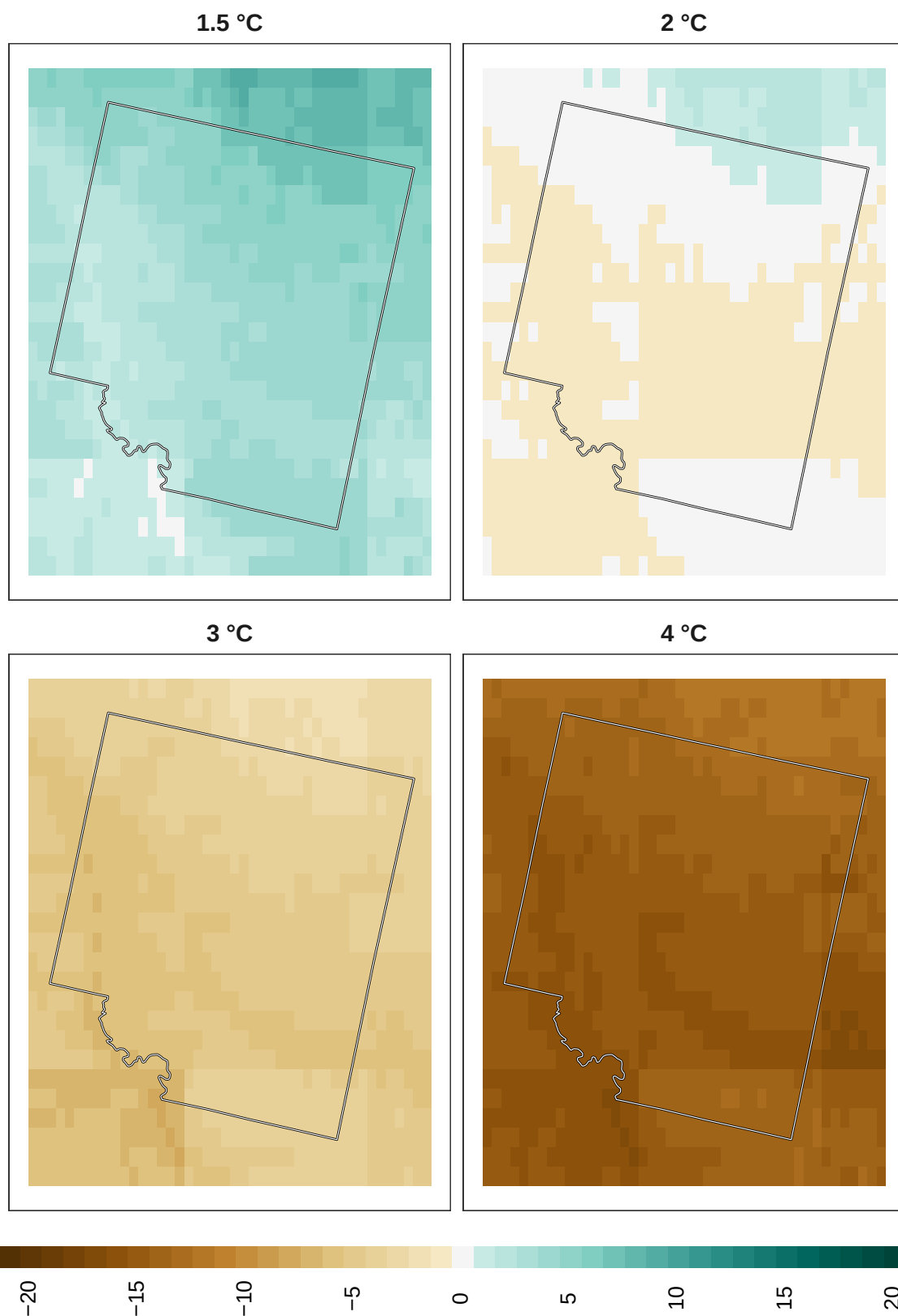
Figure 14: Adaptation effort for insects at 1 km resolution.
