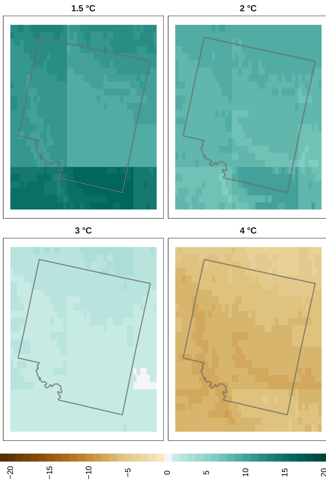
Figure 15: Adaptation effort for pollinators at 1 km resolution.
