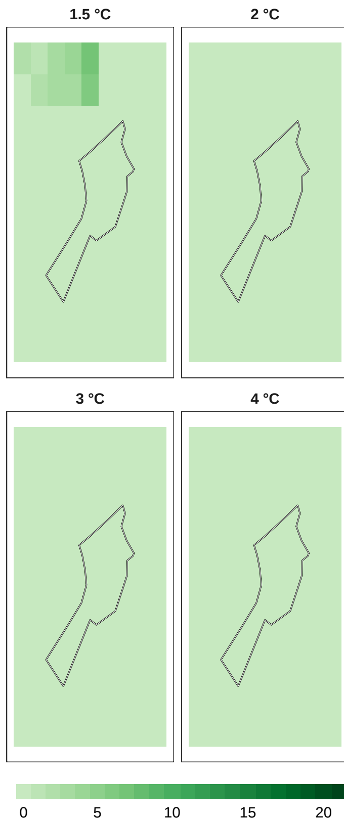
Figure 12: Number of models in agreement for pollinator refugia at 1 km resolution.
