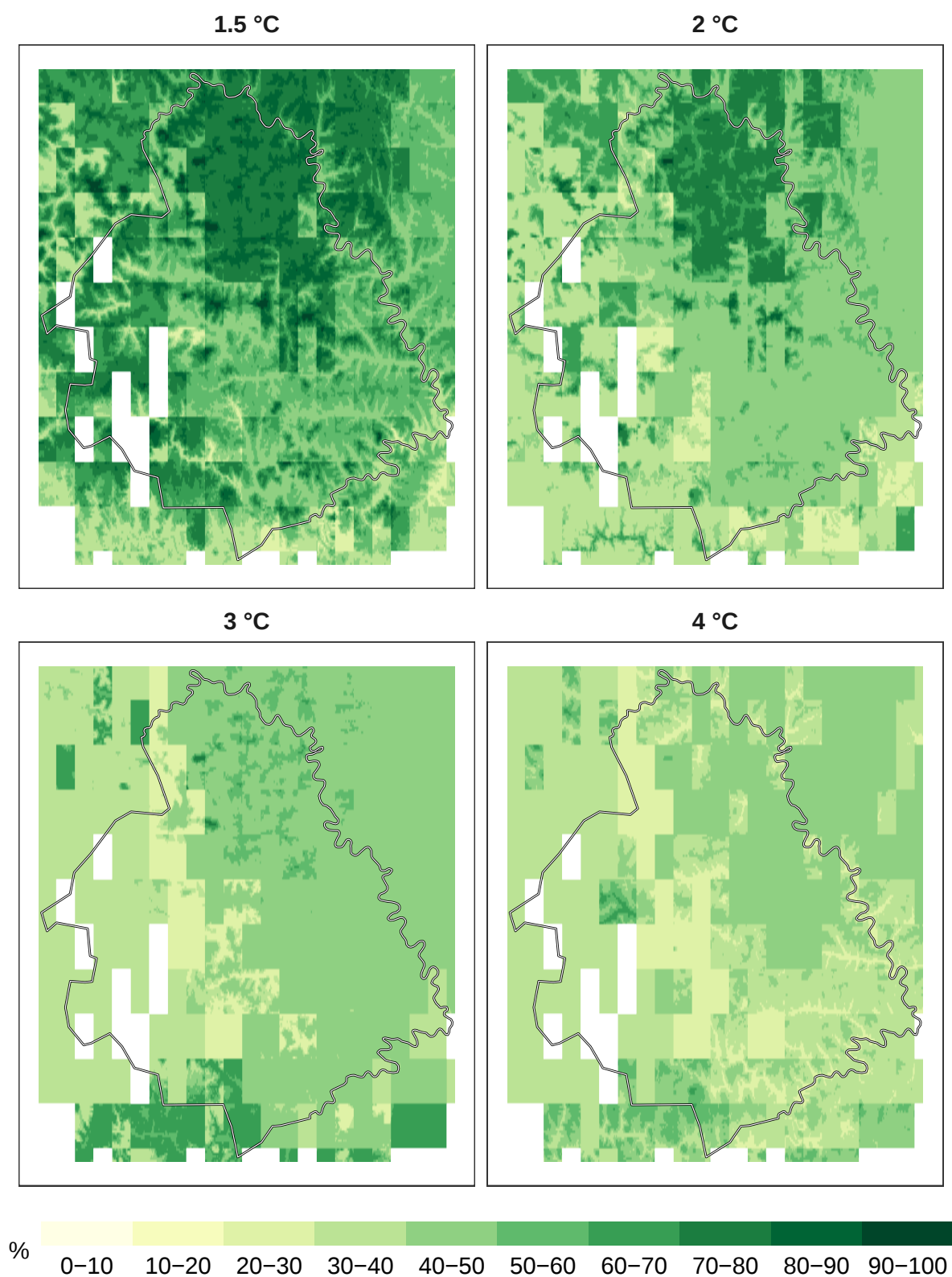
Figure 2: Percent mammals remaining at 1 km resolution.
