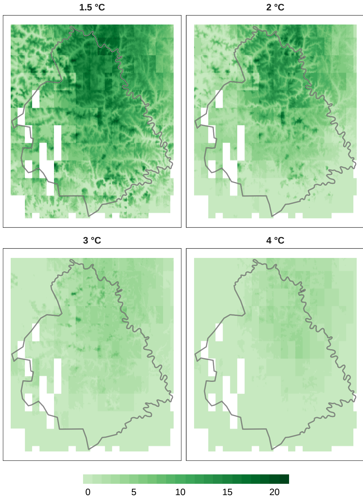
Figure 3: Number of models in agreement for overall biodiversity refugia at 1 km resolution.
