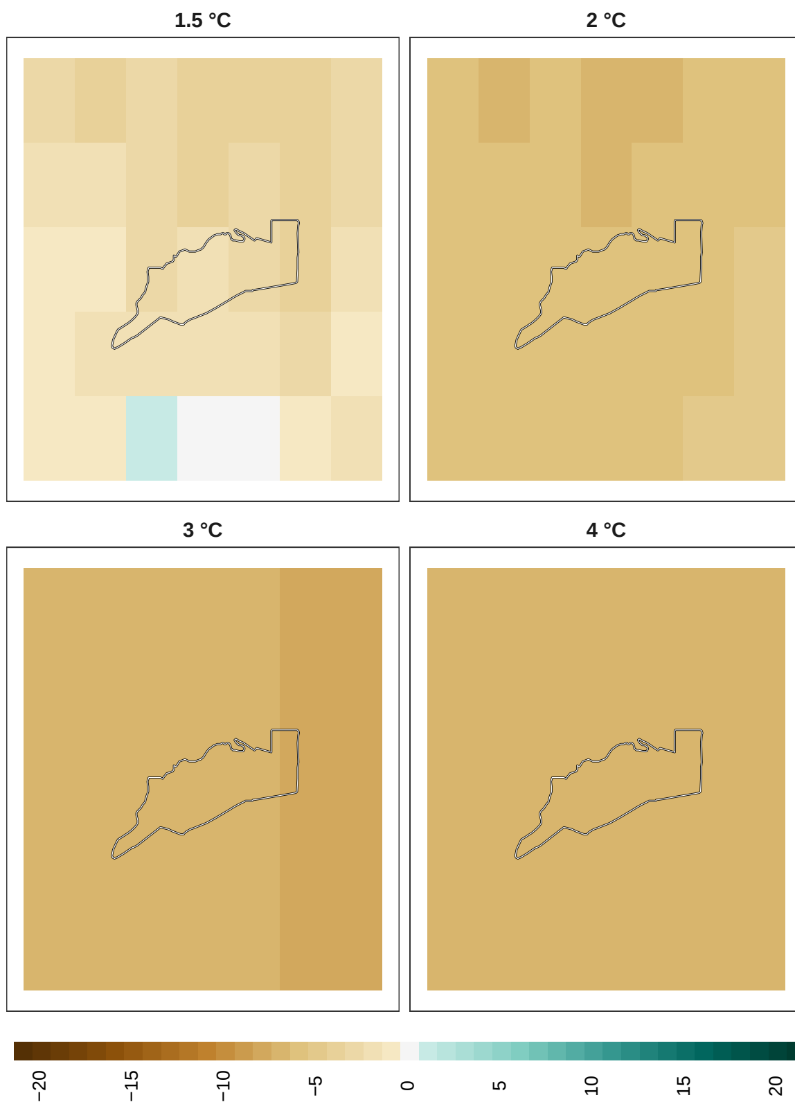
Figure 18: Adaptation effort for reptiles at 1 km resolution.
