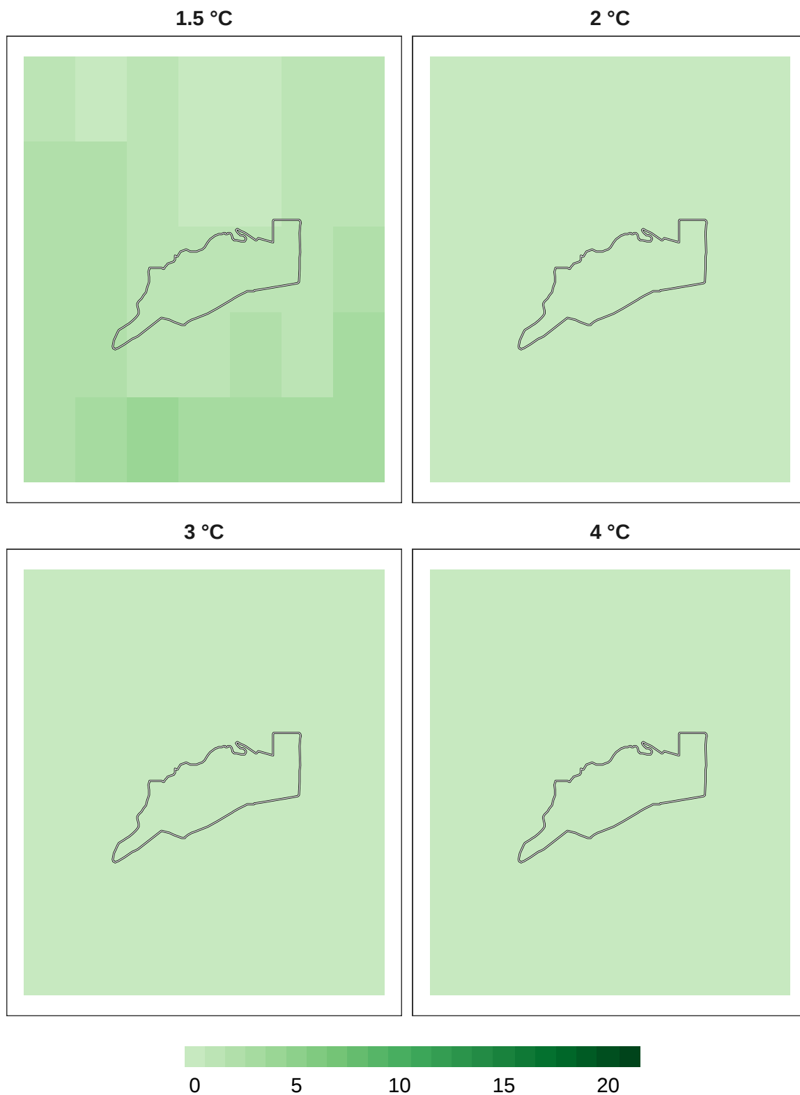
Figure 12: Number of models in agreement for reptile refugia at 1 km resolution.
