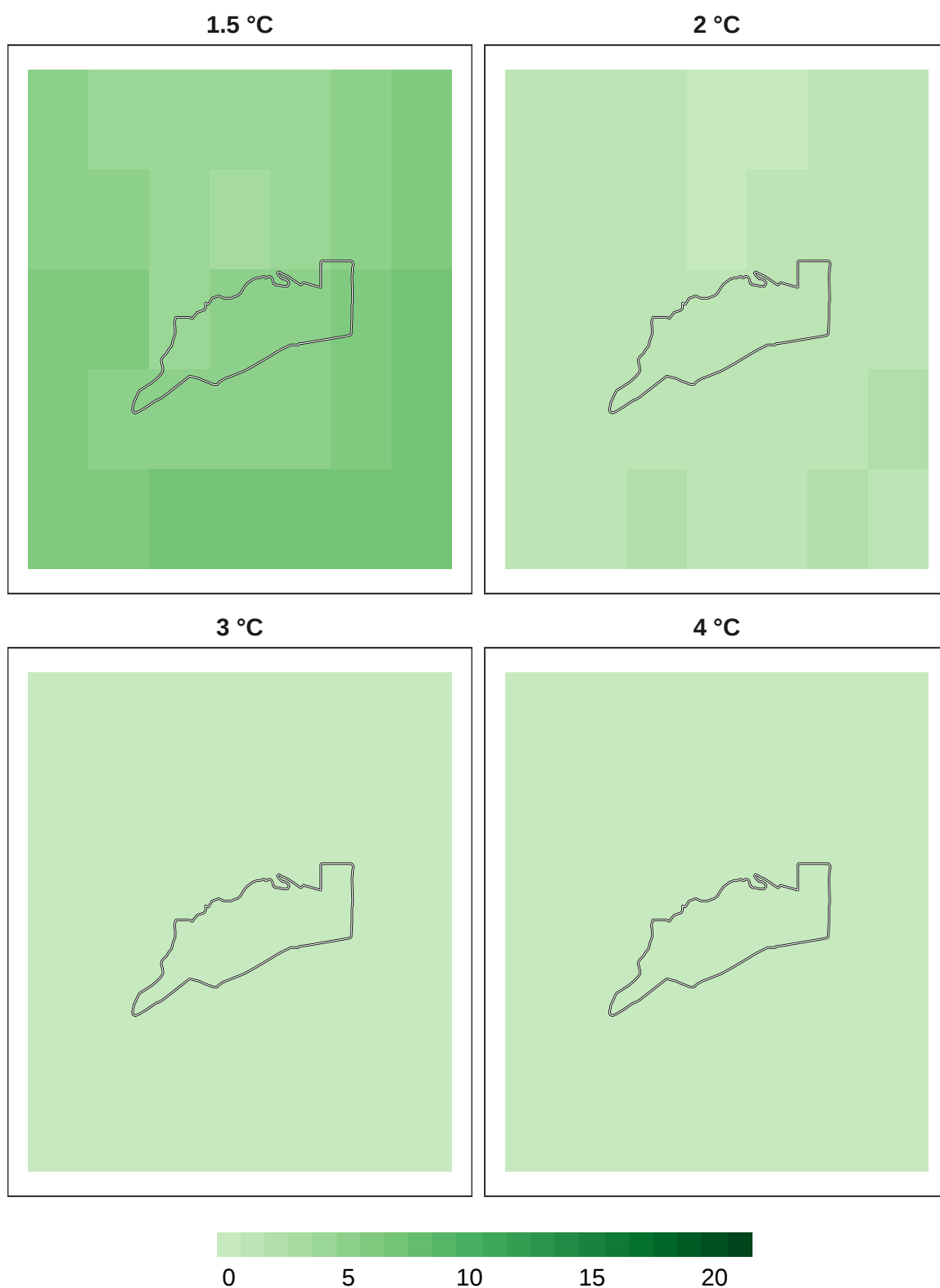
Figure 13: Number of models in agreement for insect refugia at 1 km resolution.
