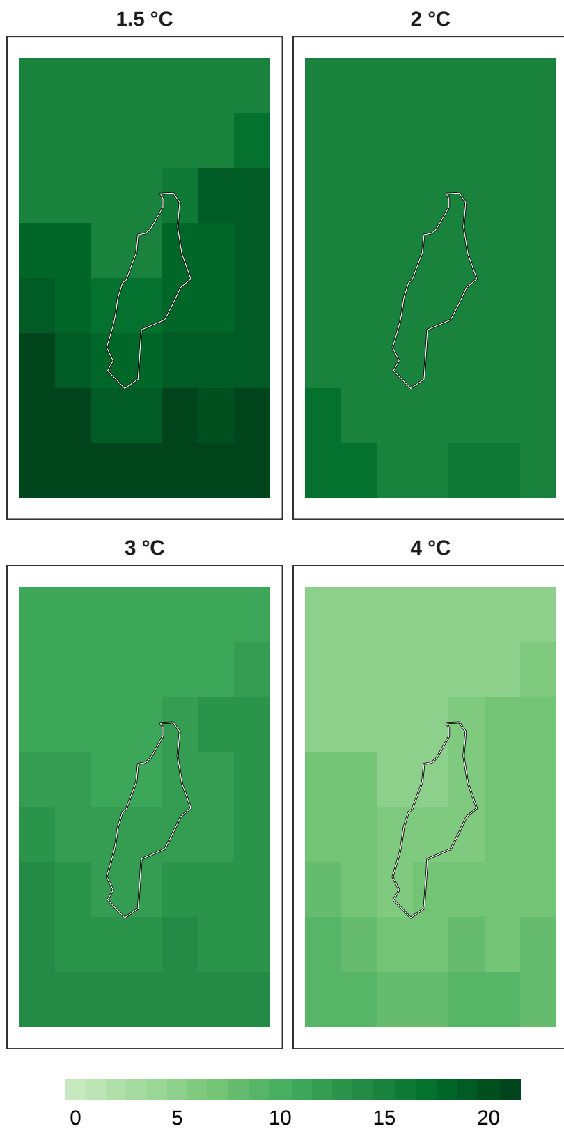
Figure 9: Number of models in agreement for reptile refugia at 1 km resolution.
