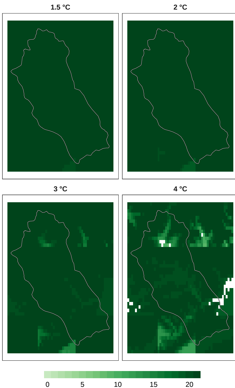
Figure 8: Number of models in agreement for mammal refugia at 1 km resolution.
