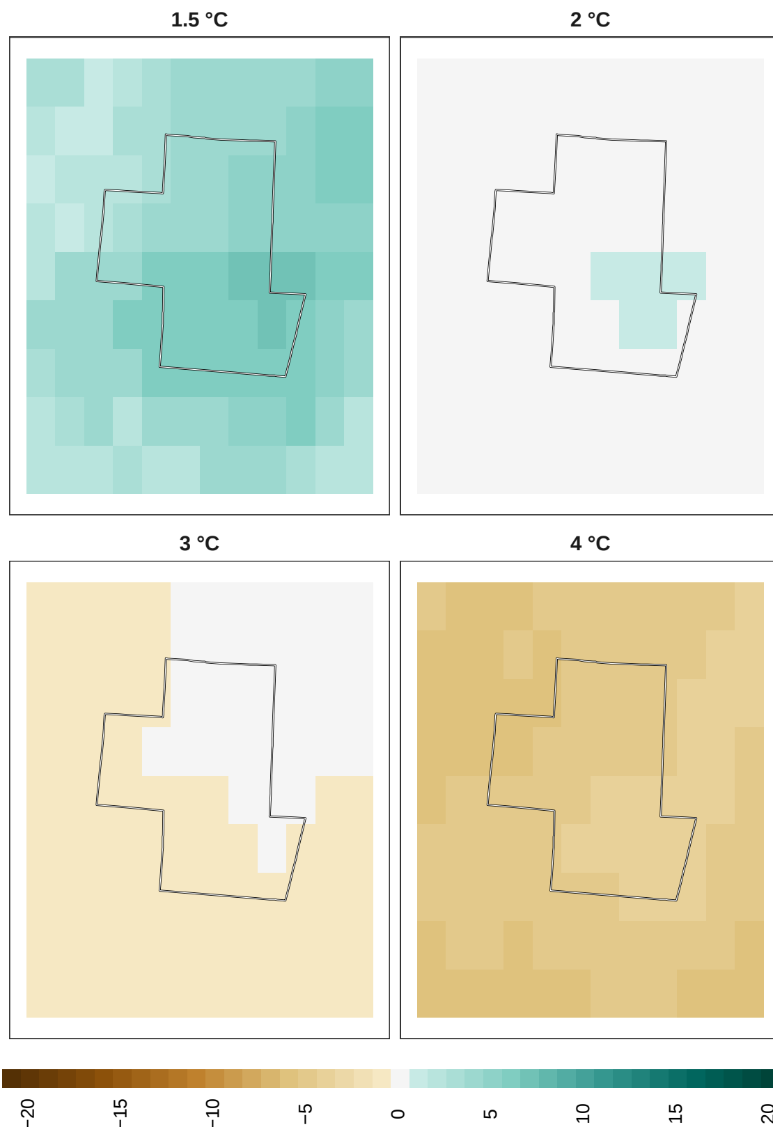
Figure 12: Adaptation effort for overall biodiversity at 1 km resolution.
