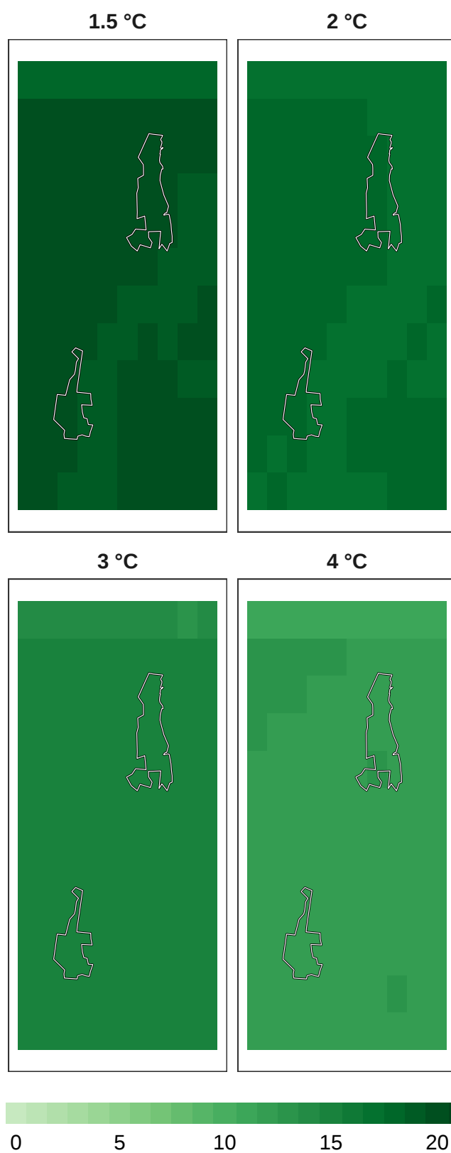
Figure 10: Number of models in agreement for bird refugia.
