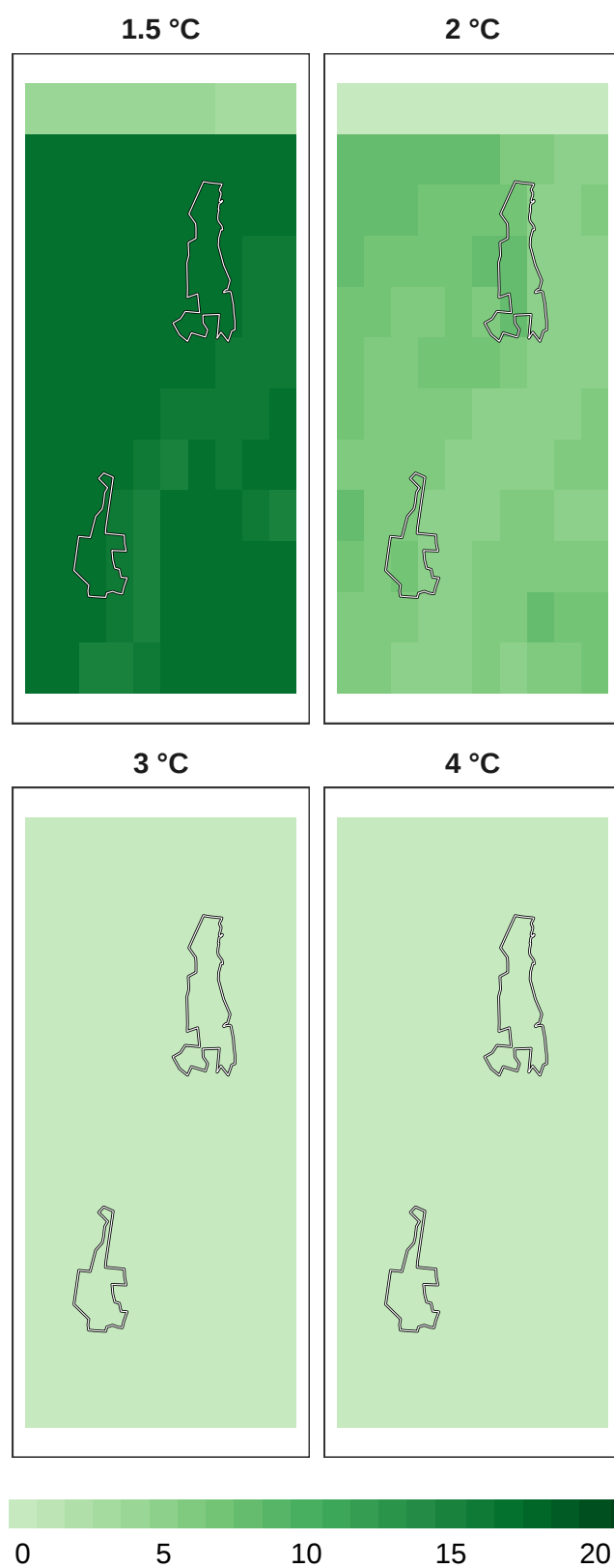
Figure 13: Number of models in agreement for pollinator refugia at 1 km resolution.
