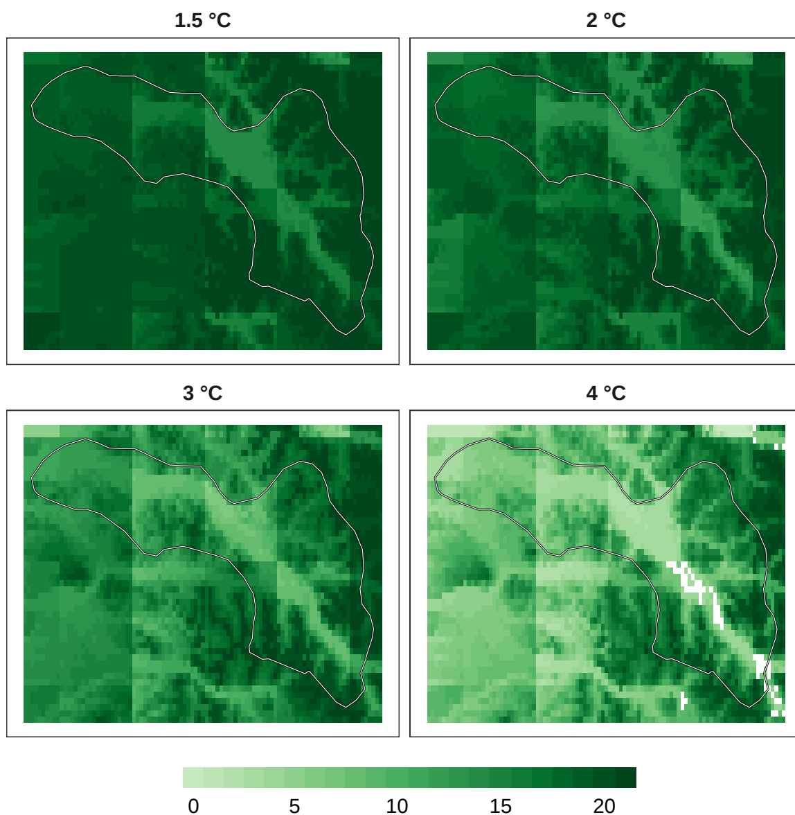
Figure 11: Number of models in agreement for insect refugia at 1 km resolution.
