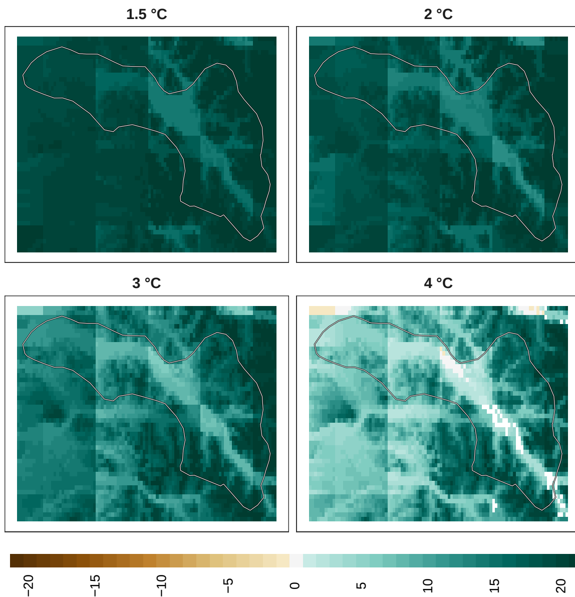
Figure 16: Adaptation effort for insects at 1 km resolution.
