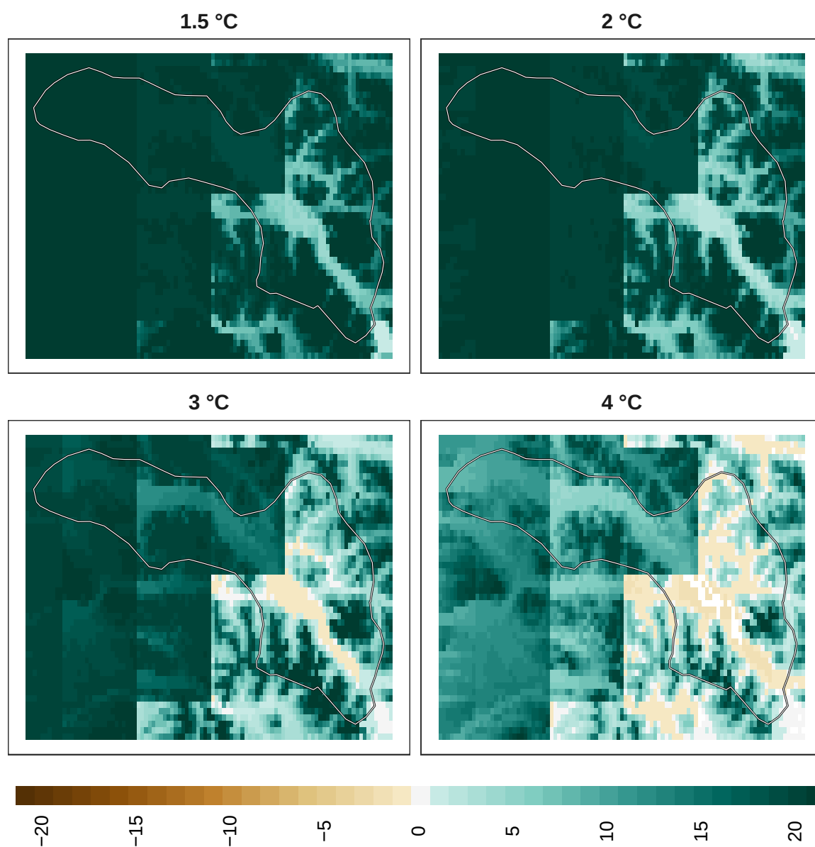
Figure 15: Adaptation effort for mammals at 1 km resolution.
