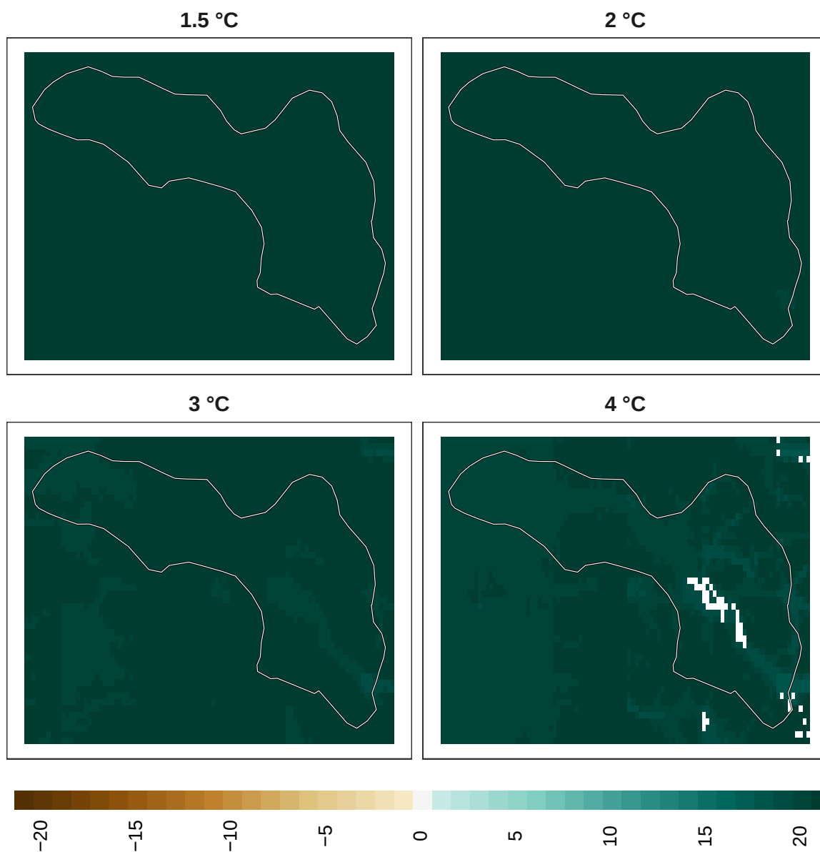
Figure 14: Adaptation effort for birds at 1 km resolution.
