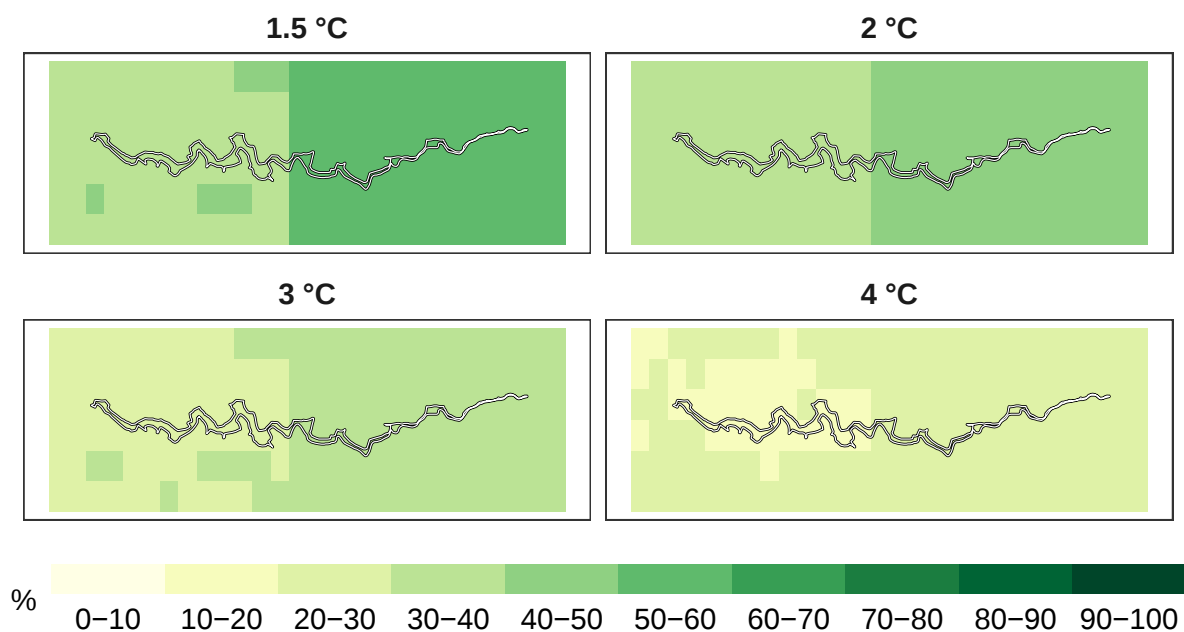
Figure 7: Percent timber species remaining at 1 km resolution.
