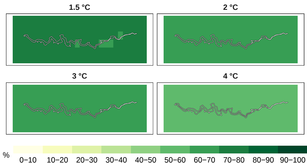
Figure 4: Percent mammals remaining at 1 km resolution.
