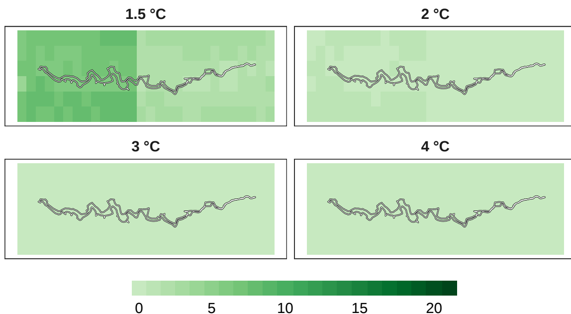
Figure 13: Number of models in agreement for pollinator refugia at 1 km resolution.
