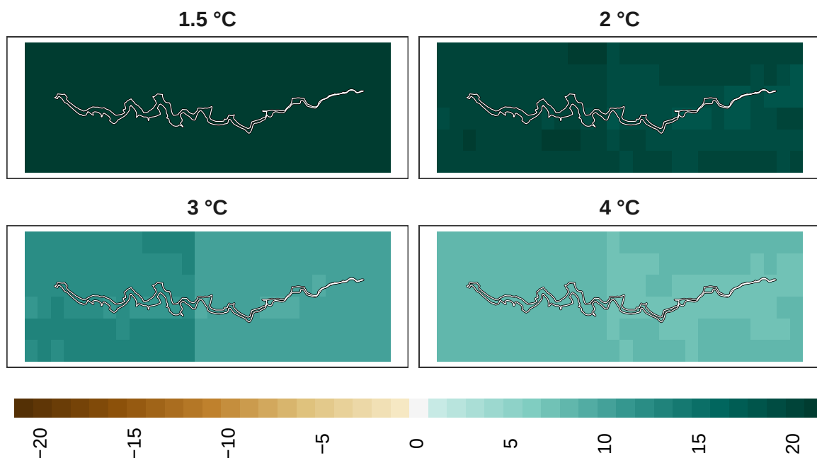
Figure 16: Adaptation effort for birds at 1 km resolution.
