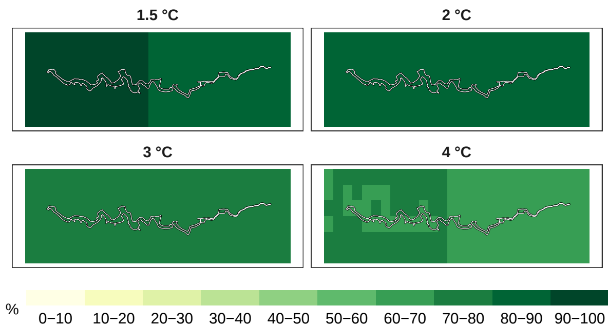
Figure 3: Percent birds remaining at 1 km resolution.
