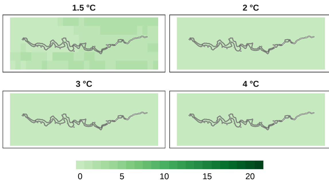
Figure 8: Number of models in agreement for overall biodiversity refugia at 1 km resolution.
