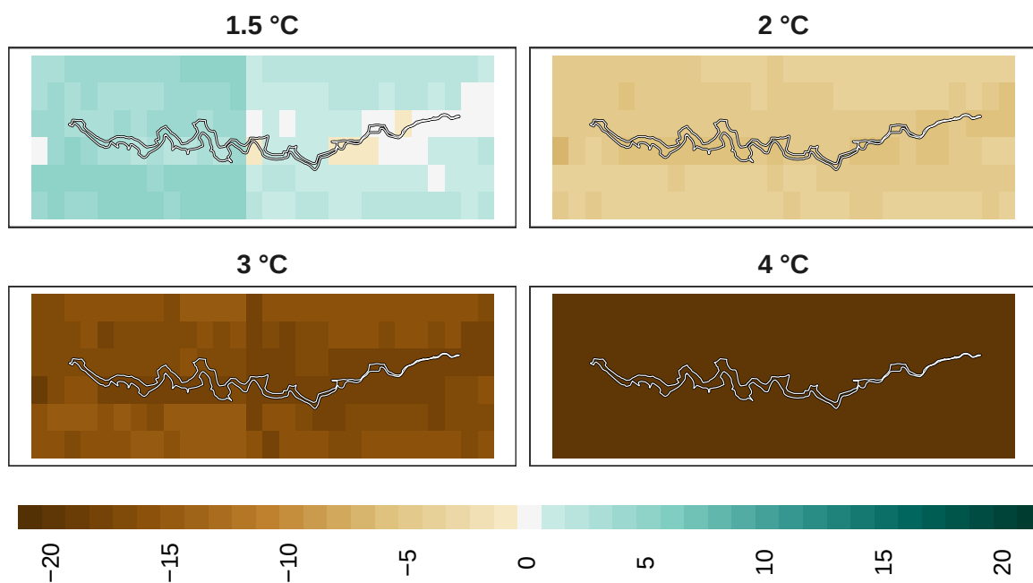
Figure 19: Adaptation effort for pollinators at 1 km resolution.
