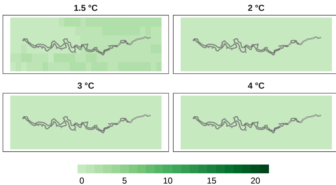
Figure 9: Number of models in agreement for plant refugia at 1 km resolution.
