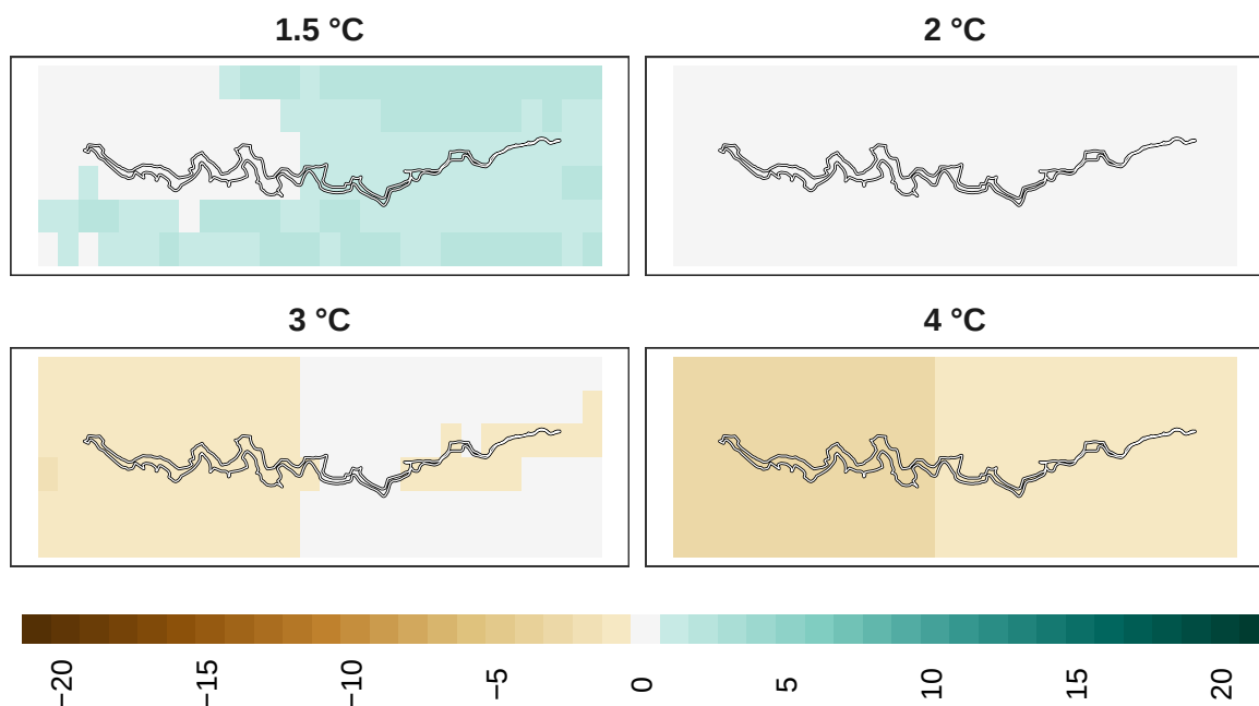
Figure 14: Adaptation effort for overall biodiversity at 1 km resolution.
