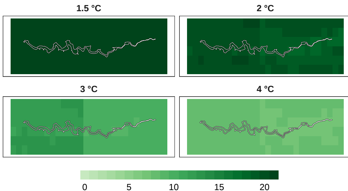
Figure 10: Number of models in agreement for bird refugia.
