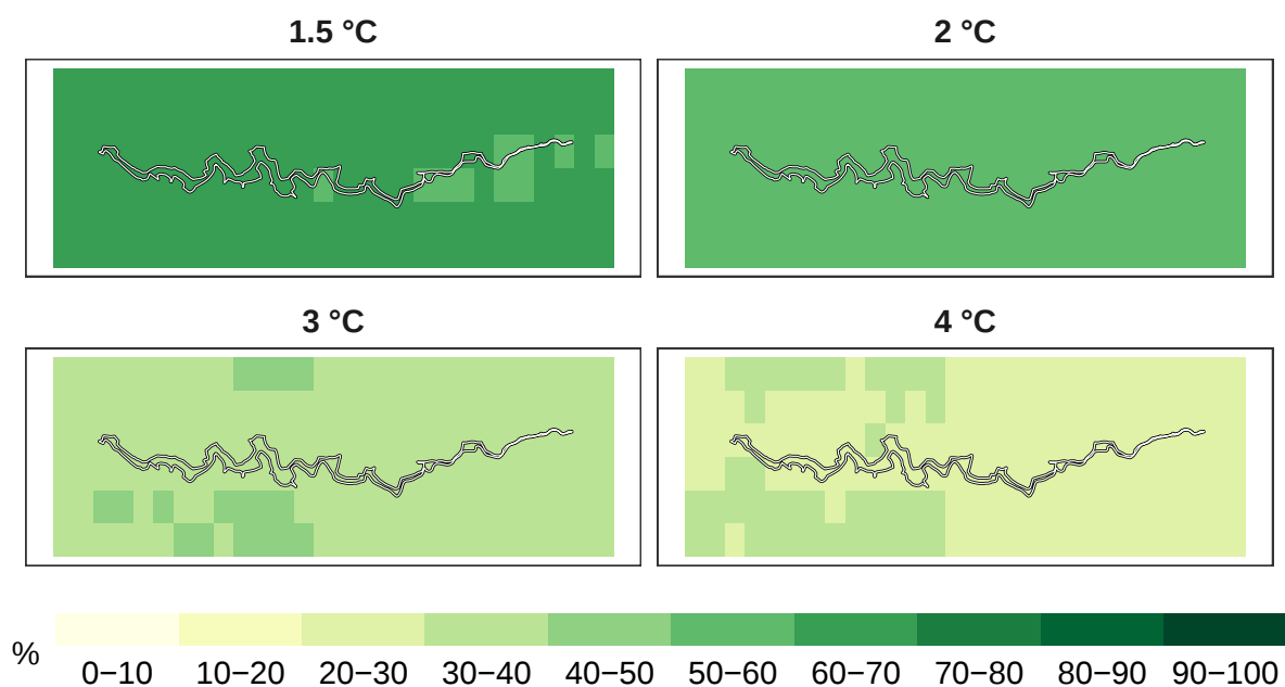
Figure 5: Percent insects remaining at 1 km resolution.
