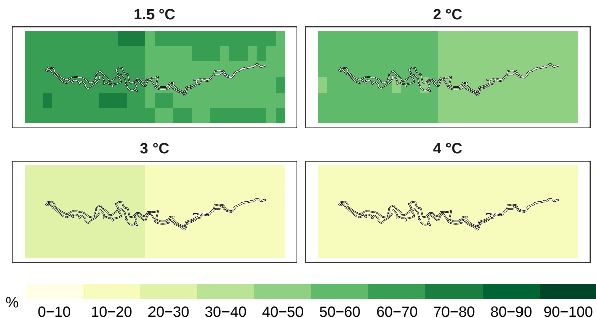
Figure 6: Percent pollinators remaining at 1 km resolution.
