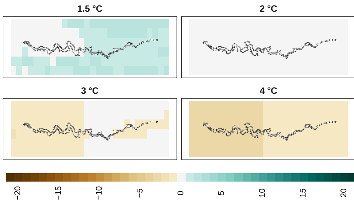
Figure 15: Adaptation effort for plants at 1 km resolution.
