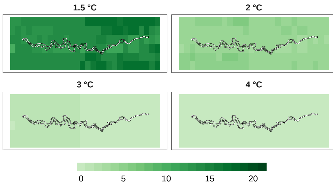
Figure 11: Number of models in agreement for mammal refugia at 1 km resolution.
