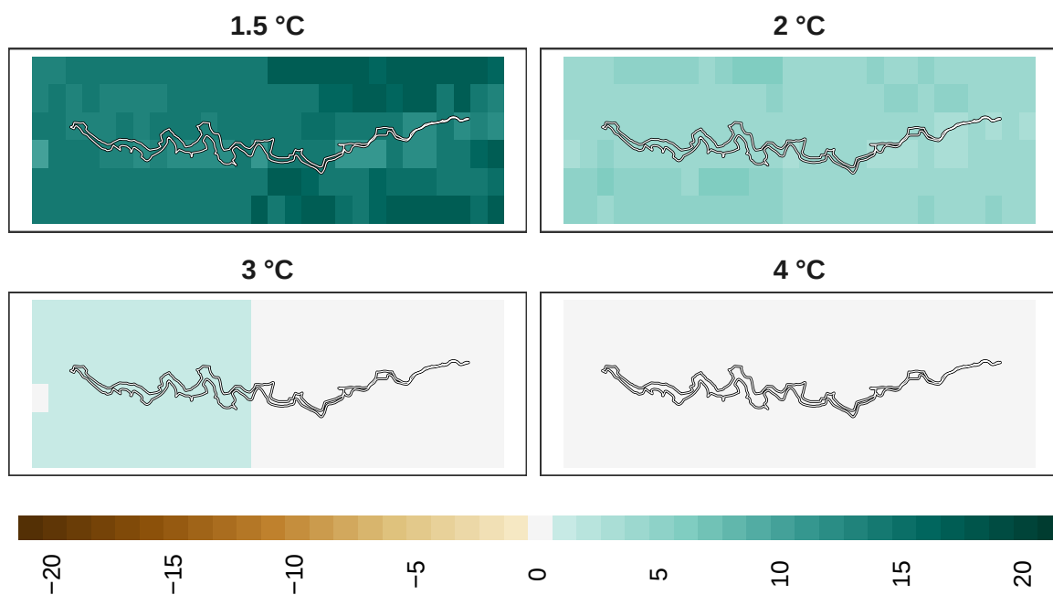
Figure 17: Adaptation effort for mammals at 1 km resolution.
