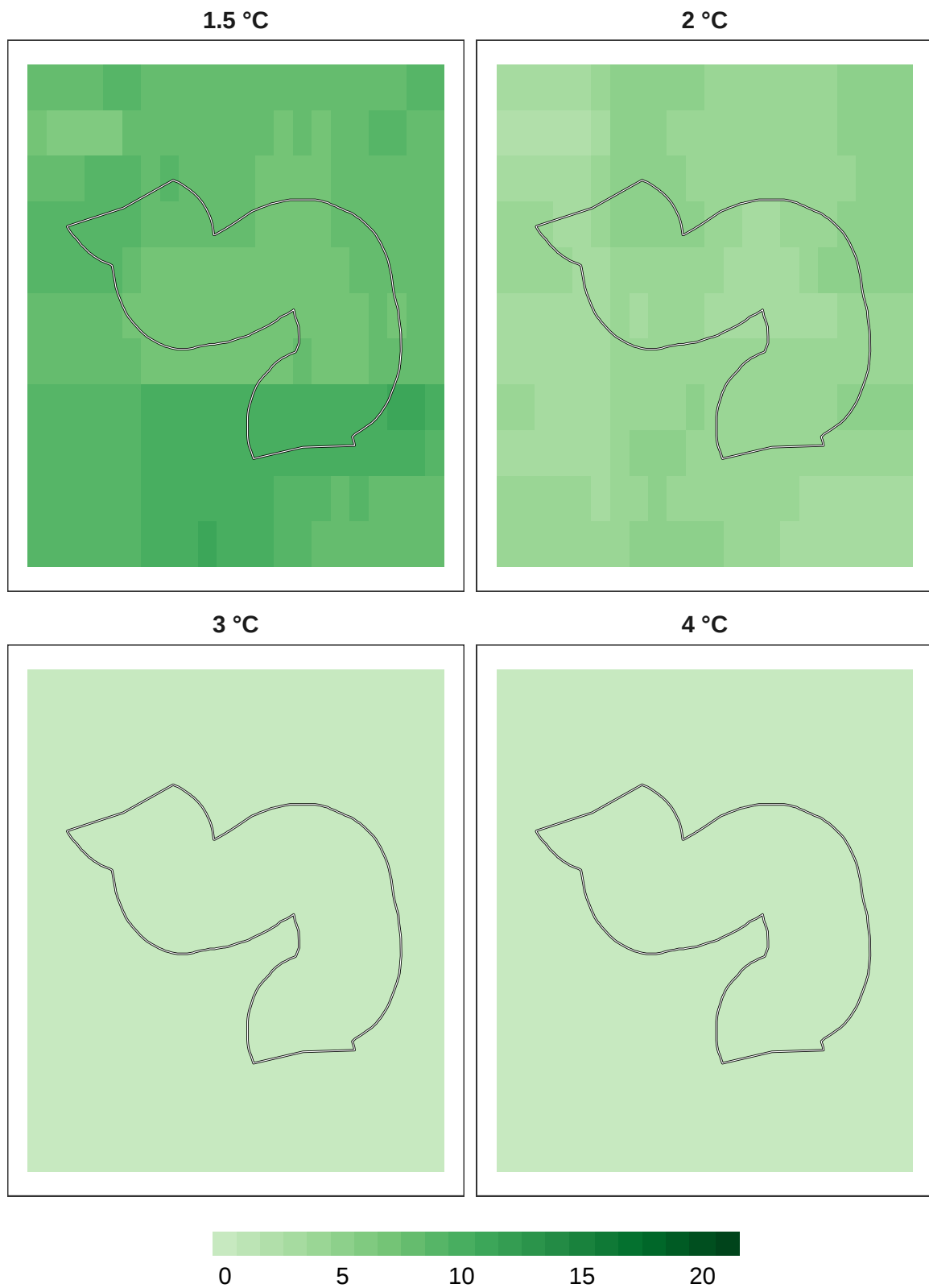
Figure 9: Number of models in agreement for insect refugia at 1 km resolution.
