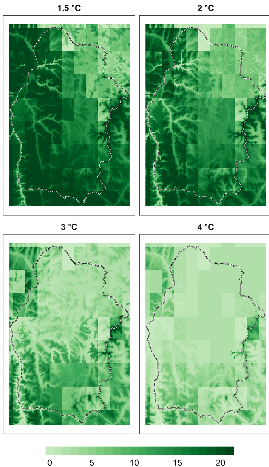
Figure 8: Number of models in agreement for mammal refugia at 1 km resolution.
