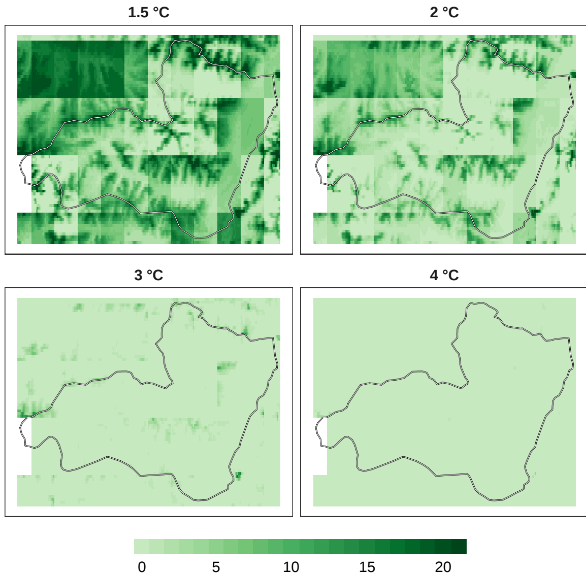
Figure 5: Number of models in agreement for plant refugia at 1 km resolution.
