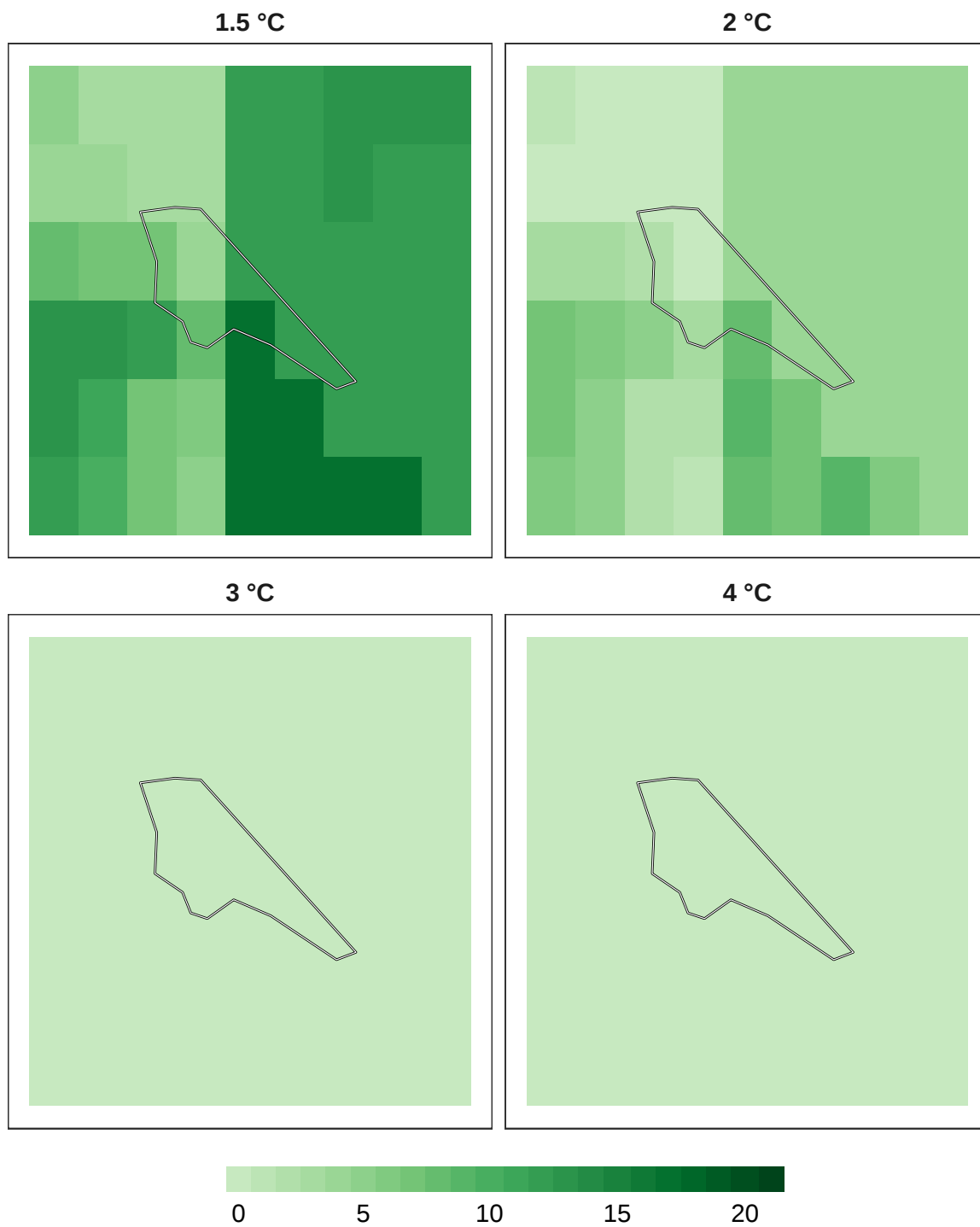
Figure 12: Number of models in agreement for reptile refugia at 1 km resolution.
