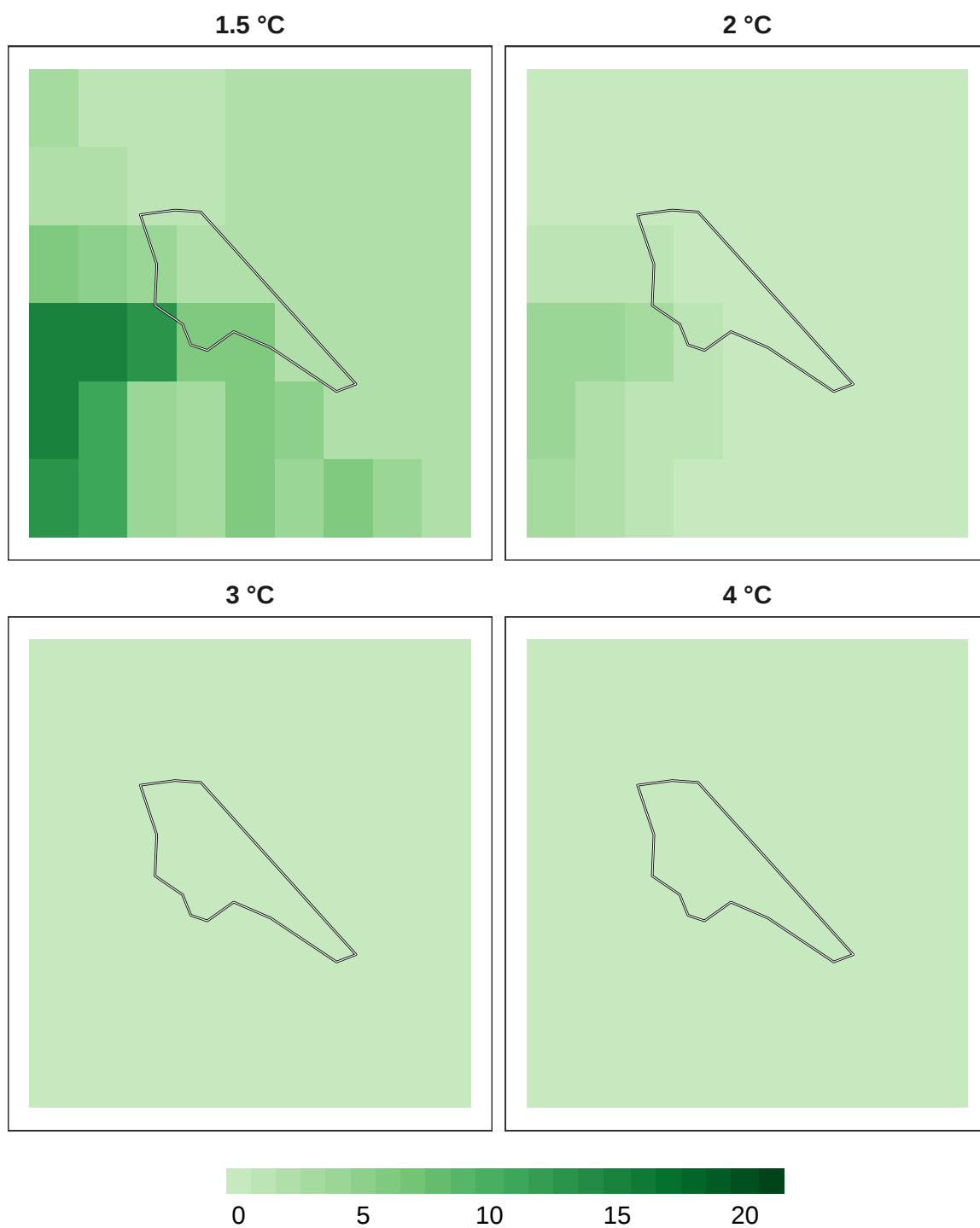
Figure 13: Number of models in agreement for insect refugia at 1 km resolution.
