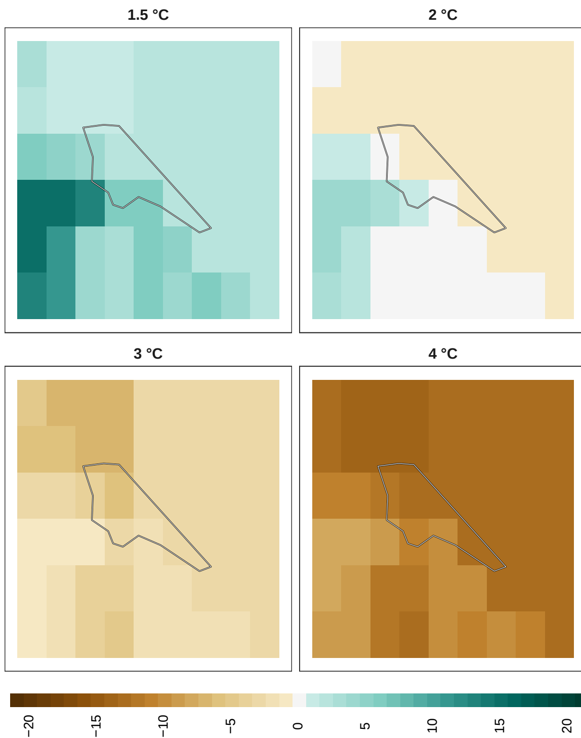
Figure 19: Adaptation effort for insects at 1 km resolution.
