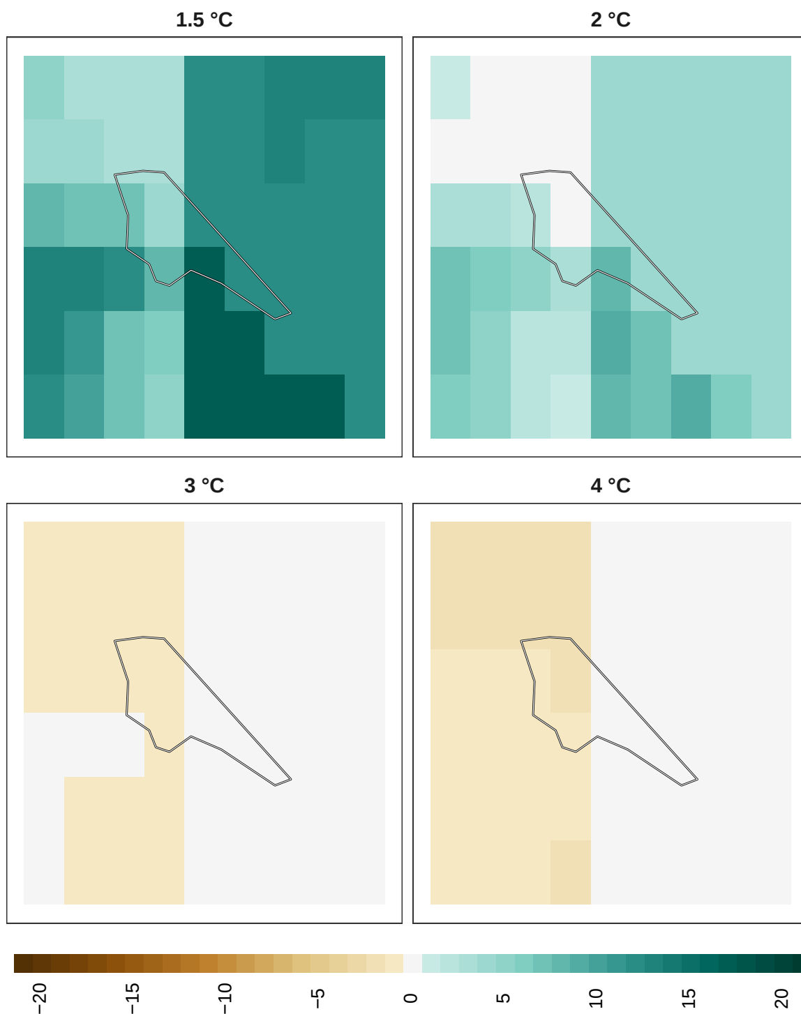
Figure 18: Adaptation effort for reptiles at 1 km resolution.
