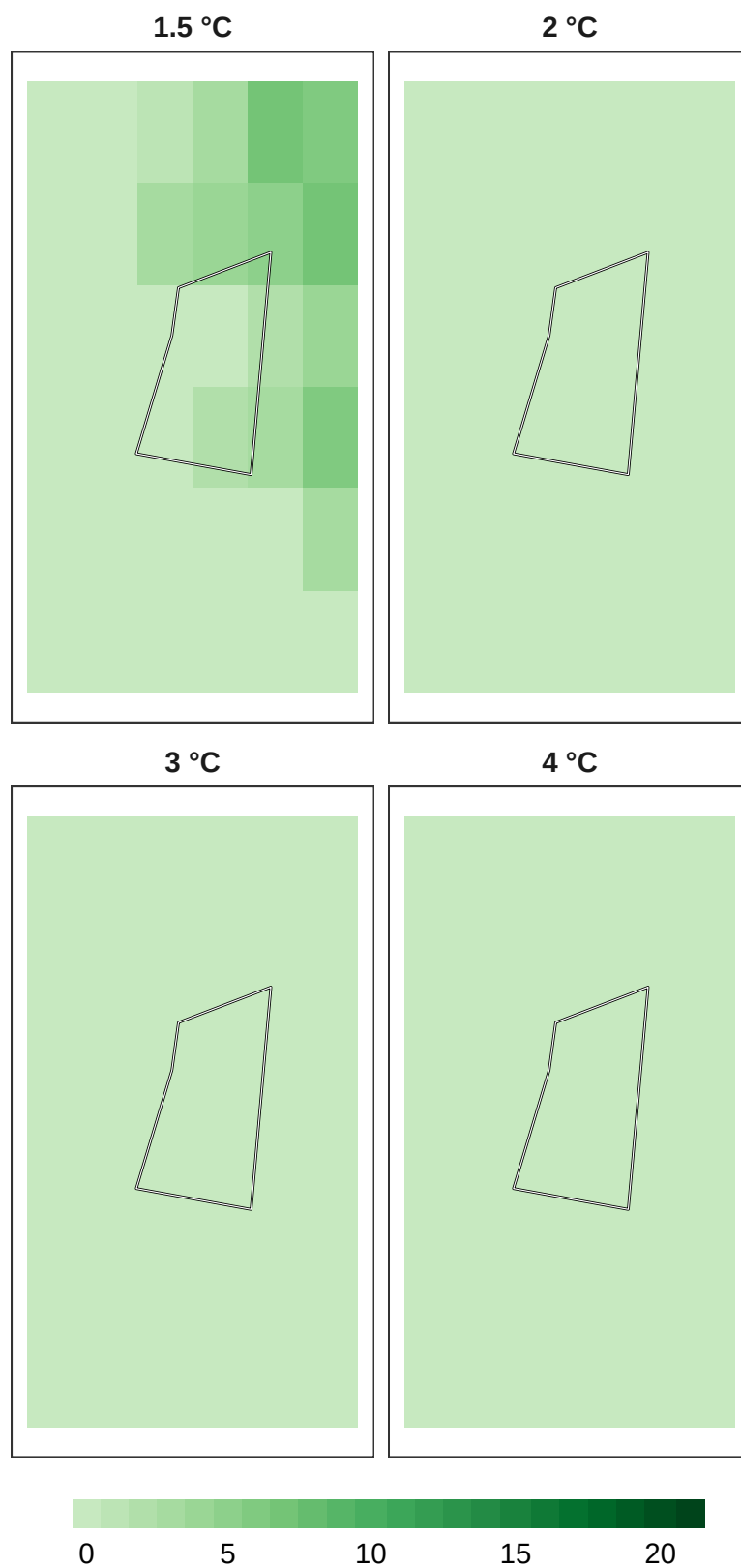
Figure 12: Number of models in agreement for pollinator refugia at 1 km resolution.
