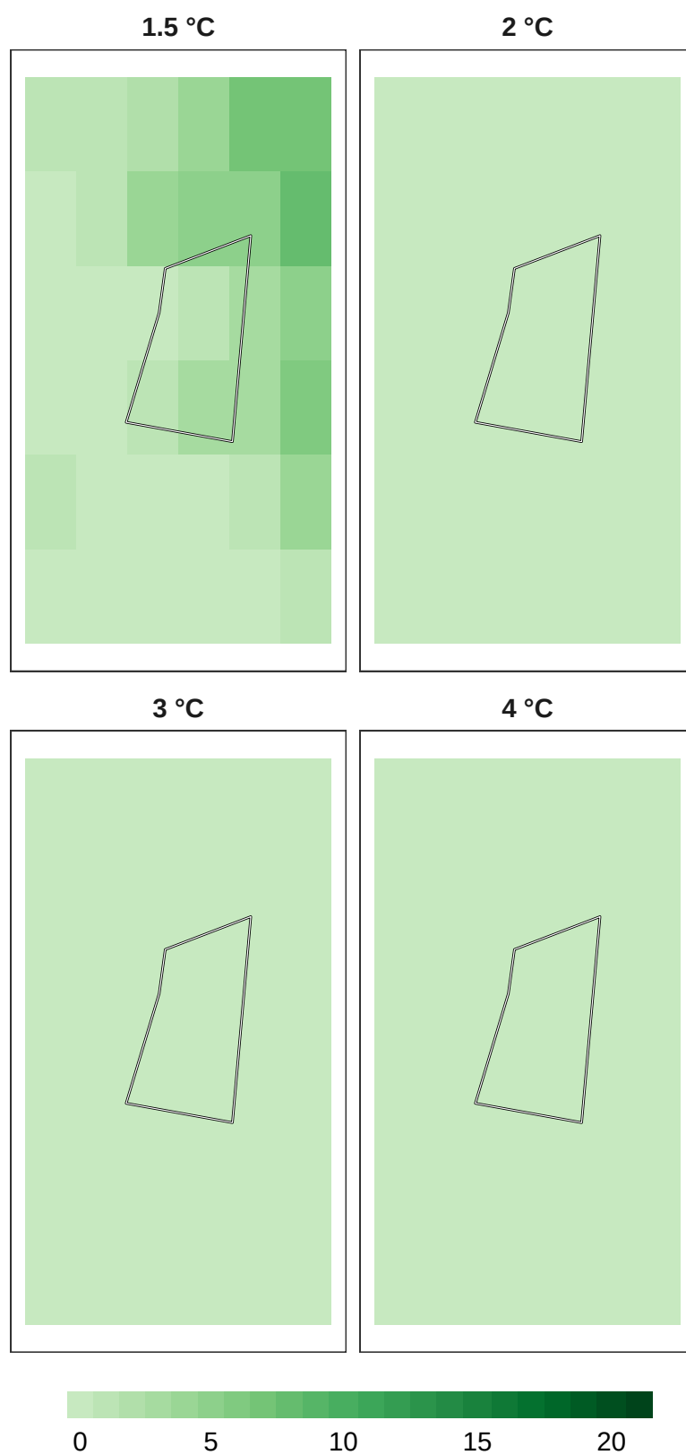
Figure 11: Number of models in agreement for insect refugia at 1 km resolution.
